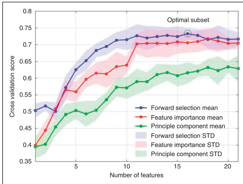
Figure 5. The classification performance for the HV-MI-MII task versus number of features for three different feature selection methods. The mean accuracy (Mean) and standard deviation (STD) are shown as solid lines and shaded areas, respectively. The forward feature selection (FFS) approach outperforms the feature importance and PCA methods.
