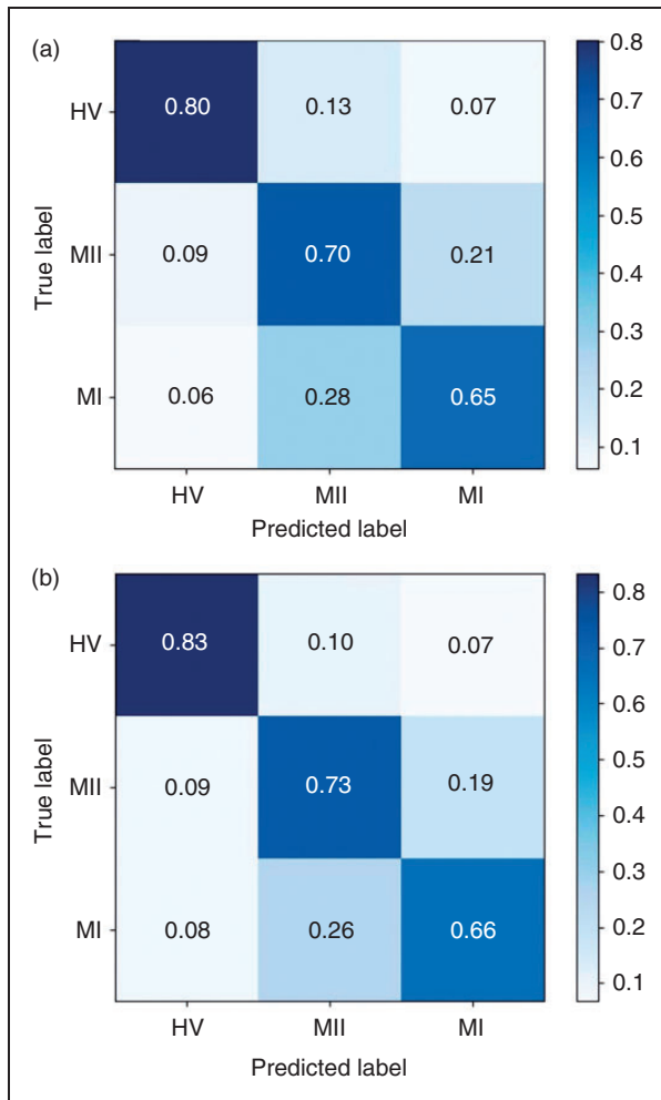
Figure 6. (a) The original confusion matrix; (b) confusion matrix after feature selection. Following forward feature selection, the diagonal elements of the matrix grow larger, indicating that more samples are correctly classified. This implies that FFS effectively boosts the system performance in migraine states classification tasks, while reducing the number of redundant features.
