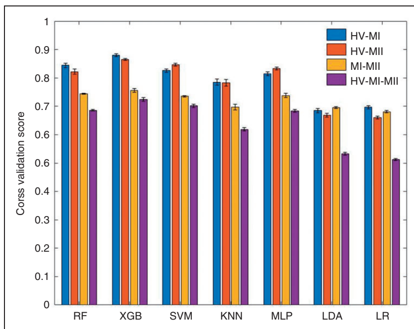
Figure 3. The accuracy measured by 10-fold cross validation score (mean \pm STD) for different tasks and various machine learning models. The algorithms are trained and tested on the entire feature set, and the classifier settings are optimized for each task.
