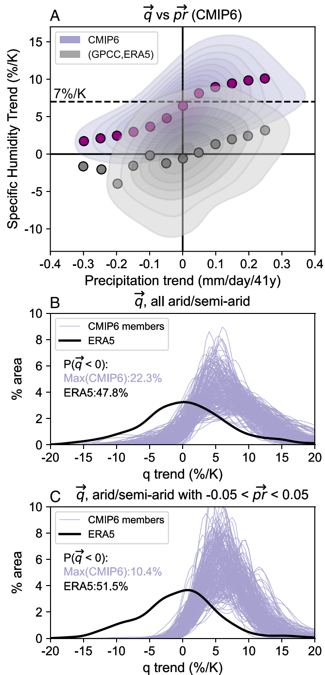
Fig. 4. Probabilities of specific humidity trends ( \vec{q} ) as a function of precipitation trends ( \vec{p} ) in arid and semi-arid regions. (A) area weighted joint probability distribution of specific humidity trend (expressed as a percentage of the 1980 to 1990 climatology and normalized by the land area average temperature trend, excluding Antarctica) versus precipitation trend for arid/semi-arid regions using a Gaussian kernel density estimate. Gray shows observation-based data (GPCC for \vec{p} and ERA5 for \vec{q} , see SI Appendix, Fig. S11 for alternatives) and purple shows the ensemble mean of the first member for each CMIP6 model (probability distribution calculated for each model first and then averaged). Contours show the probability per 0.025 mm/d/41 y \vec{p} by 0.5 %/K \vec{q} box with contours starting at 0.04% and increasing in increments of 0.02% and the circles show the area weighted average specific humidity trend for \vec{p} bins of width 0.05 mm/d/41 y. (B) Gaussian kernel density estimate of the % area of all arid/semi-arid regions exhibiting specific humidity trends using 0.5 %/K bins. Black shows ERA5 and purple lines show all members from all models for CMIP6. The text depicts the percent area exhibiting negative trends for ERA5 and the CMIP6 member with the maximum area of negative trends. (C) is as (B) but now the probability estimates are performed only on arid/semi-arid grid points that exhibit precipitation trends between -0.05 and 0.05 mm/d/41 y.
