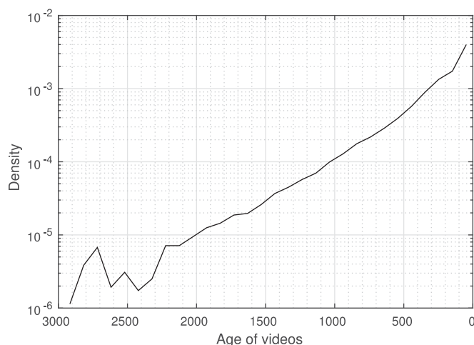
Fig. 7. Histogram of the number of videos in the dataset as a function of the age of the videos. There is a significant percentage of newer videos (videos with less age) compared to older videos. Hence, the dataset captures the exponential growth of the number of videos uploaded and is an unbiased sample of YouTube.
