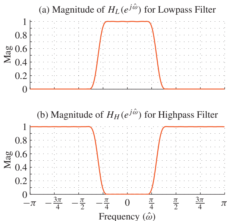
Figure 2: Frequency response magnitudes for (a) LPF and (b) HPF. Notice that |H_H(e^{j\hat{\omega}})| = 1 - |H_L(e^{j\hat{\omega}})| .
