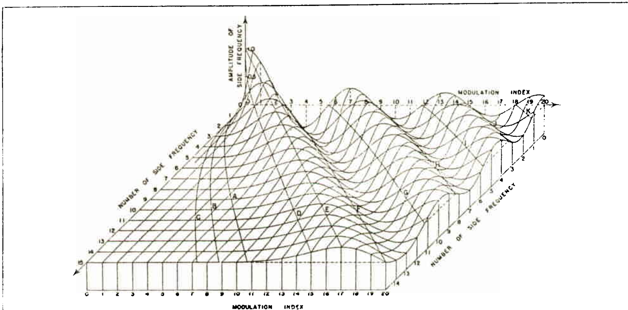
Fig. 8. Bessel functions, J_n through J_{15} and indexes 0 through 20. This representation allows a rapid determination of the bandwidth resulting from a given index.
