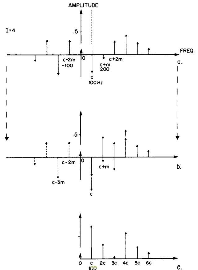
Fig. 4. Fig. 4a shows spectrum with components which lie in the negative frequency domain; b shows plot from a in which the frequencies in the negative domain are reflected around 0 Hz with an inversion of phase and added to the components in the positive domain; c is plot of the magnitude of the components of b.
