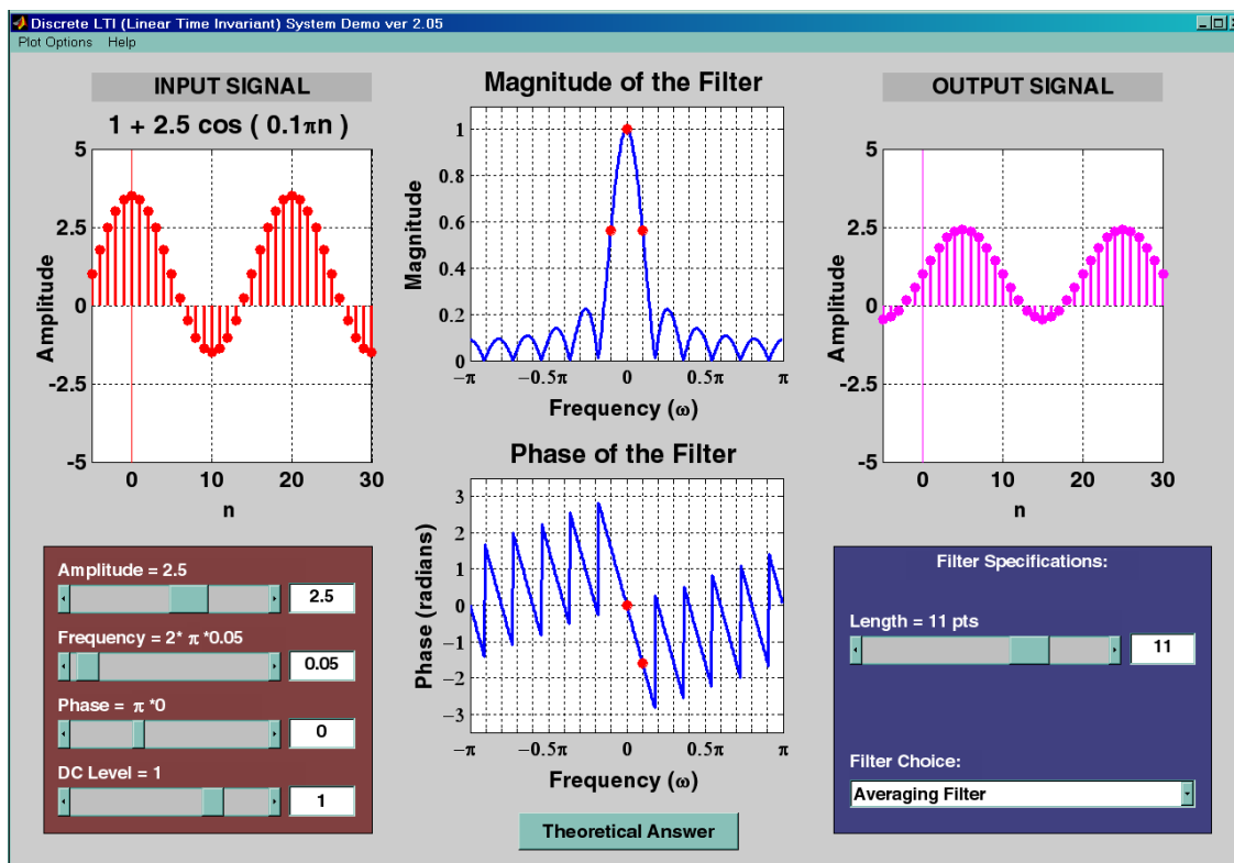
Figure 1: DLTl demo interface. The frequency label is \omega because MATLAB won’t display the hat in \hat{\omega} .
