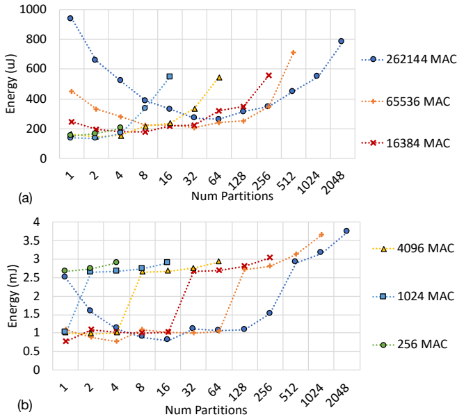
Fig. 12: Energy consumption in running (a) Layer Cba_3 from Resnet50 and (b) layer TF0 from Transformer, when scaling-up and scaling out with different MAC units
