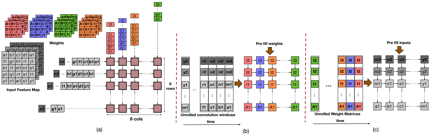
Fig. 3: Schematic showing the mapping in various dataflows (a) Output stationary; (b) Weight stationary; (c) Input stationary
