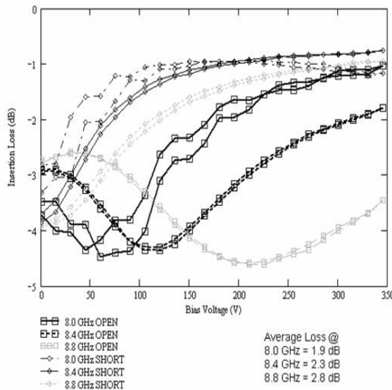
Figure 5. Measured insertion loss of ferroelectric phase shifter at three different X-band frequencies.
