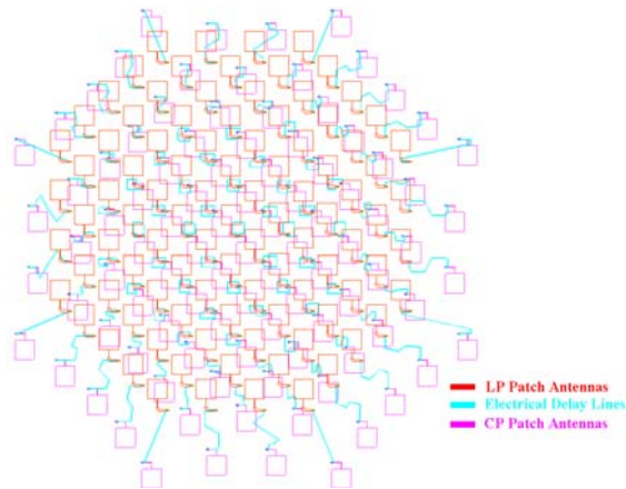
Fig. 3 Layout of the passive DLA
