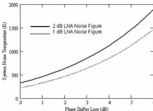
Figure 4. Calculated reflectarray system noise temperature as a function of phase shifter insertion loss. A background temperature of 55 K is assumed.
