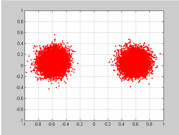
Figure 10. Output of the decision-directed PLL showing a BPSK constellation. The circular symmetry of the clusters indicates Gaussian noise.
