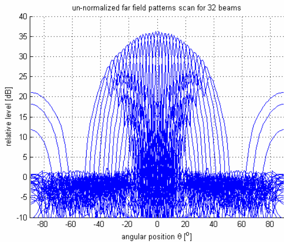
Fig. 3. Scan loss and un-normalized radiation pattern for 32 beams. Scalloping loss is better than 1.6dB (worst case).
