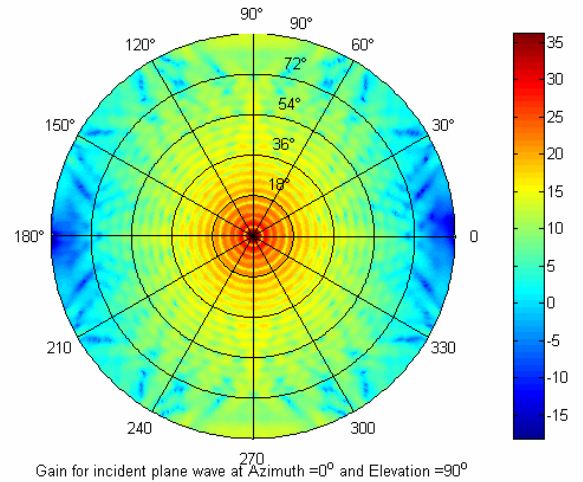
Gain for incident plane wave at Azimuth = 0° and Elevation = 90°
