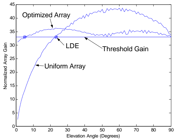
Fig. 9. The normalized link gains of the optimized SFL array and the uniform array as a function of elevation angle.
