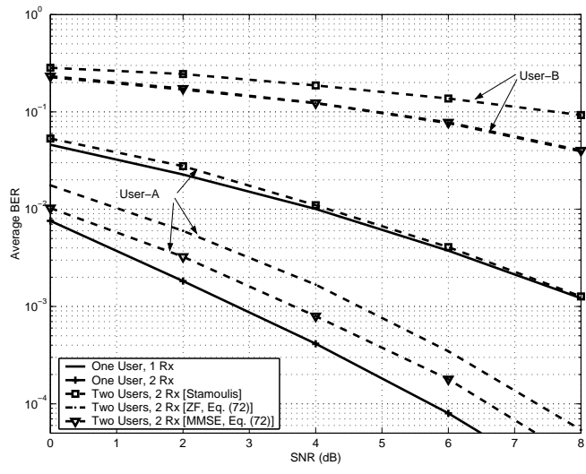
(b) Power imbalance, P_T(A) = 10P_T(B)
