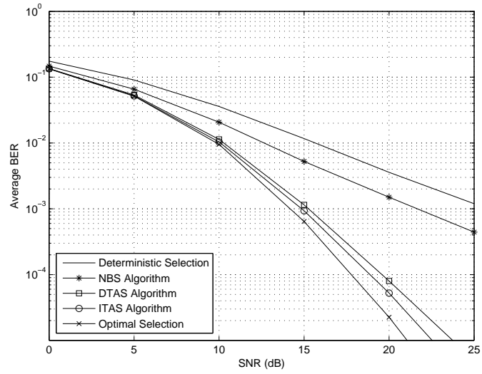
(a) SIR = 10 dB
