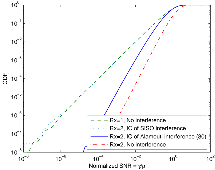
Figure 21: The cumulative density function of normalized SNR for various interference scenarios with SIR = 0\text{dB} .
