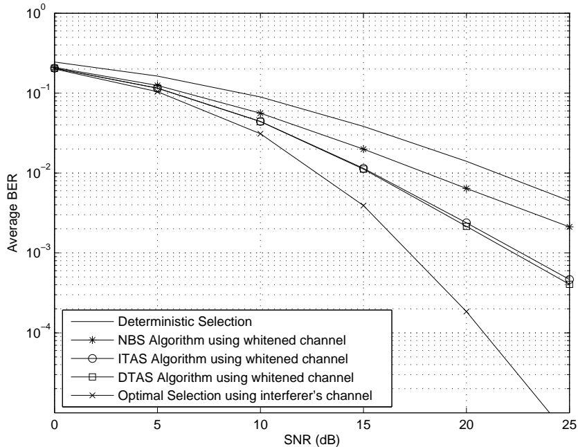
Figure 19: BER performance of MMSE receiver for (6,2) MIMO system in the presence of 2 interfering streams with SIR = 0\text{dB} . Four receive antennas are selected.
