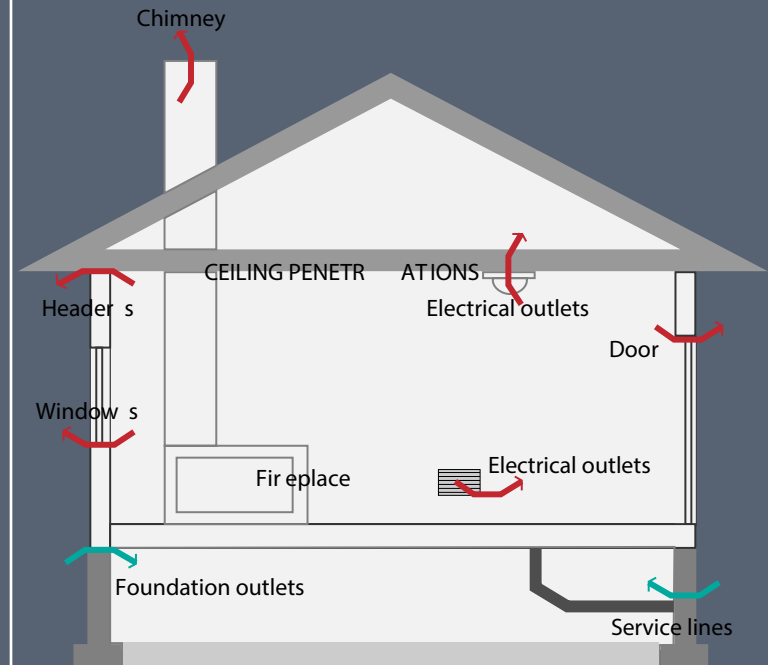
Critical areas for air sealing
