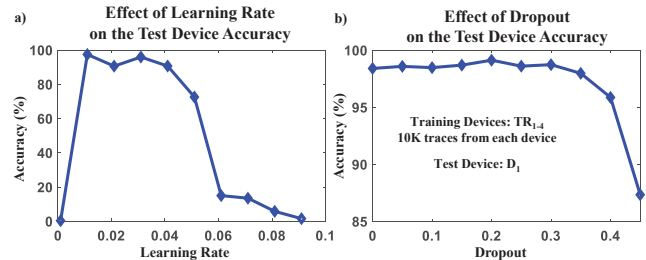
Figure 4: Effect of Model Hyper-parameters on the Test Accuracy (on the test device D_1 after training with TR_{1-4} ): (a) Learning rate (LR) of \sim 0.01 provides the maximum test accuracy, and higher LR leads to overfitting of the DNN reducing the test accuracy. (b) Lower dropout shows higher accuracy which implies that the data gathered from the microcontroller devices has sufficient electronic noise which helps generalize to unseen data. Dropout higher than 0.3 reduces the accuracy.
