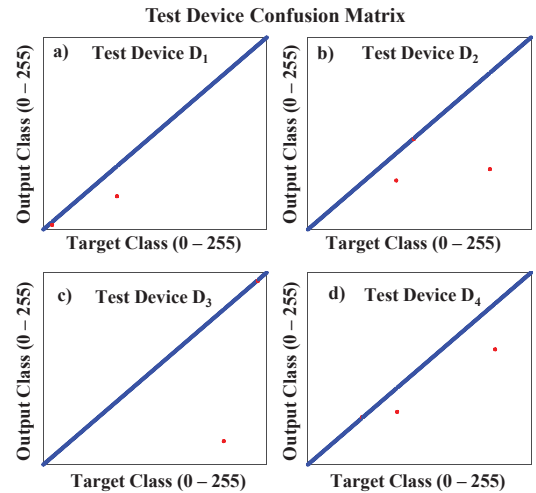
Figure 7: Confusion matrix for each of the test devices ( D_{1-4} ). At most 3 key bytes out of the 256 (~ 99% overall accuracy) are getting misclassified for each of the test devices, with the DNN model trained with 10K traces from each of the 4 training devices ( TR_{1-4} ).
