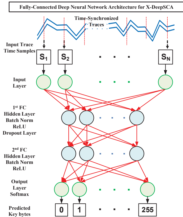
Figure 3: Architecture of the proposed Fully Connected DNN for X-DeepSCA. The input layer consists of N = 500 neurons. The 1^{st} fully-connected (FC) hidden layer consists of 200 hidden neurons, followed by Batch Normalization, Rectified Linear Unit (ReLU) activation, and a dropout layer. The 2^{nd} hidden layer is similar without the dropout layer. Finally, the output layer has 256 neurons for predicting the correct key byte utilizing the softmax function. If the traces are not aligned in time, a convolutional layer as the input layer would be required. In this work, we use the Fully Connected DNN as the traces captured from the Chipwhisperer are time-aligned.
