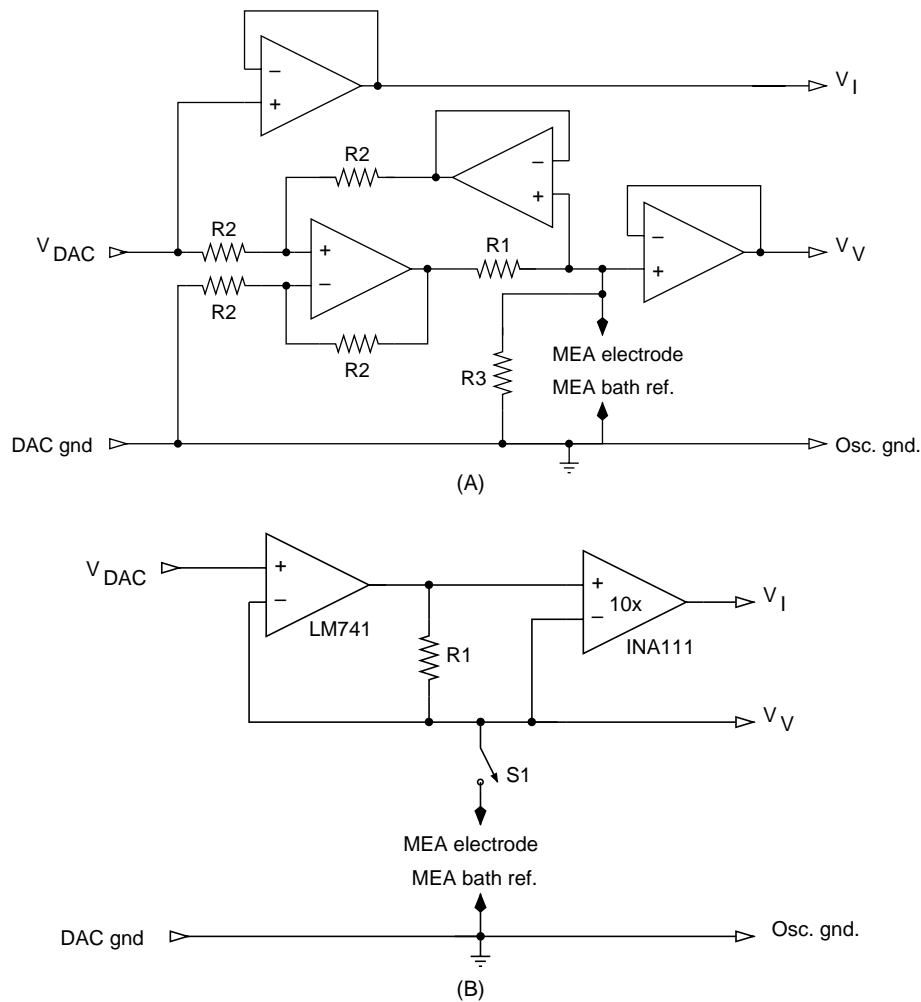
Fig. 1. Stimulation hardware. (A) Circuit for current-controlled stimulation. V_{DAC} is converted to a current I = V_{DAC}/R_1 through the resistor R_1 = 150\text{ k}\Omega . R_3 = 6.8\text{ M}\Omega acts as a shunt to prevent runaway electrode voltages (electrode impedances are 50–200 k \Omega at 1 kHz). R_2 = 150\text{ k}\Omega . Opamps are 1/4 LM348. The terminals V_V and V_I are used to monitor the electrode voltage and the driving current (multiplied by R_1 ). (B) Circuit for voltage-controlled stimulation. The MEA electrode is driven at the voltage V_{DAC} . The voltage across R_1 = 5.0\text{ k}\Omega , amplified and measured at V_I , directly reflects the current passing through the electrode. The electronic switch S_1 can be used to effectively disconnect the stimulator from the MEA, allowing neuronal signals to be recorded through the stimulated electrode shortly after stimulation. This circuit is part of a device for delivering stimuli to any electrode in an MEA with rapid switching between channels (Wagenaar and Potter, 2004).
