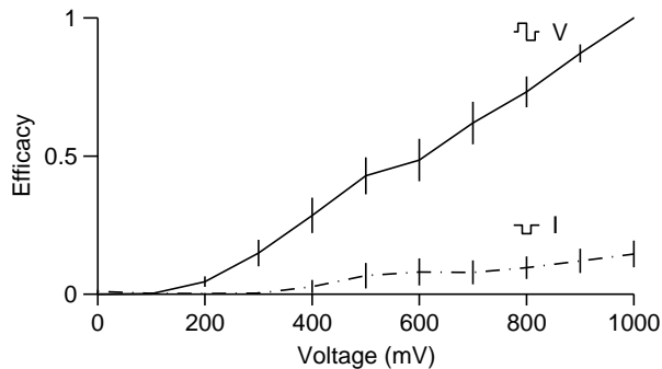
Fig. 8. Efficacy (see text) of positive-then-negative voltage-controlled pulses of 400 \mu s per-phase (solid) and monophasic negative current pulses of 50 \mu s duration for which the resulting voltage was measured (dashed). The voltage-controlled pulses are significantly more effective (average and S.E.M., N = 6 ).
