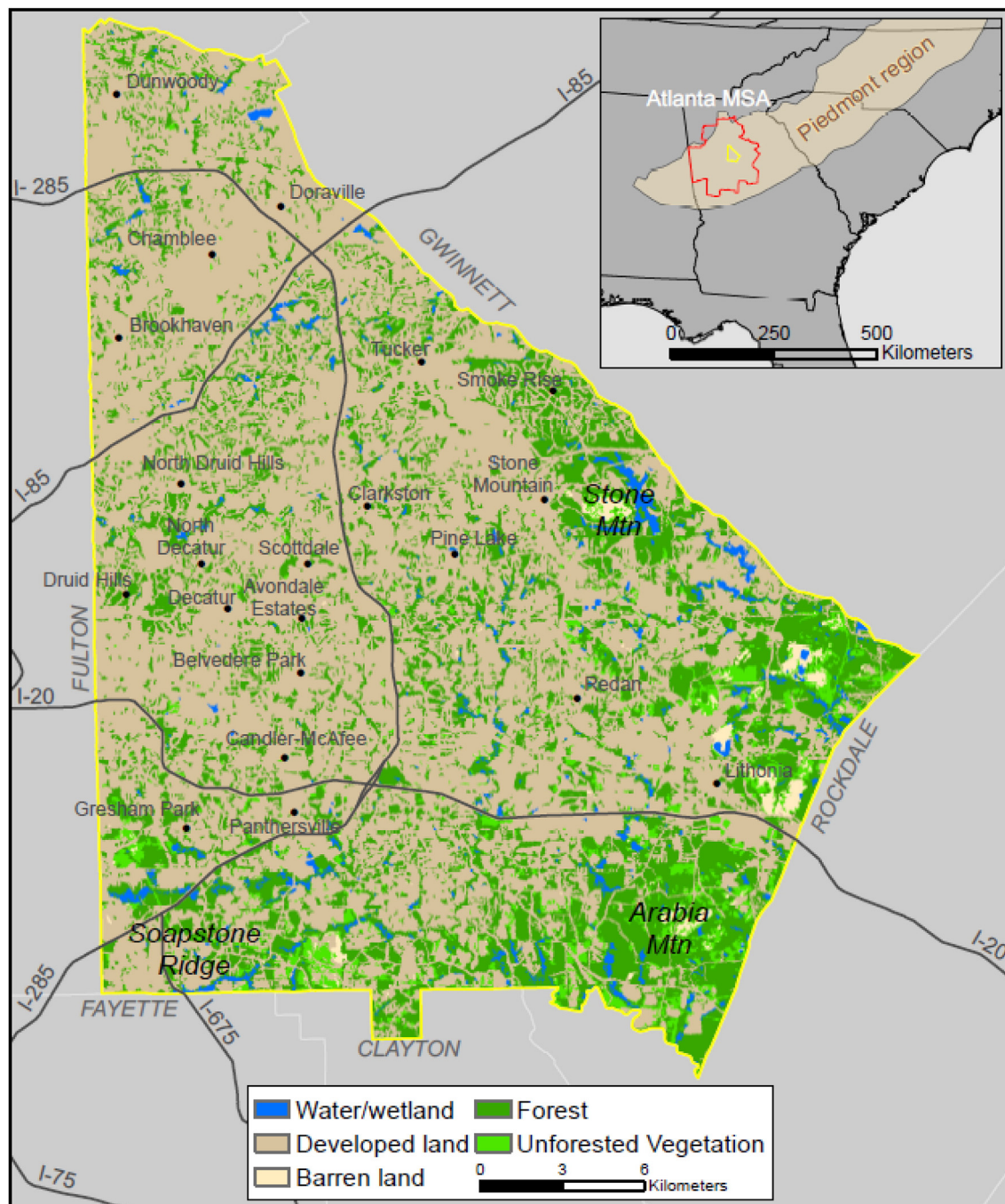
Fig. 1. This effort's study region, DeKalb County, Georgia. (Base map from Homer et al., 2015).
