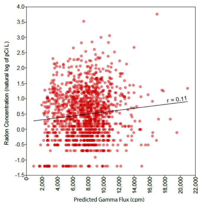
Fig. 6. Scatterplot of log-transformed indoor radon levels and predicted gamma flux.
