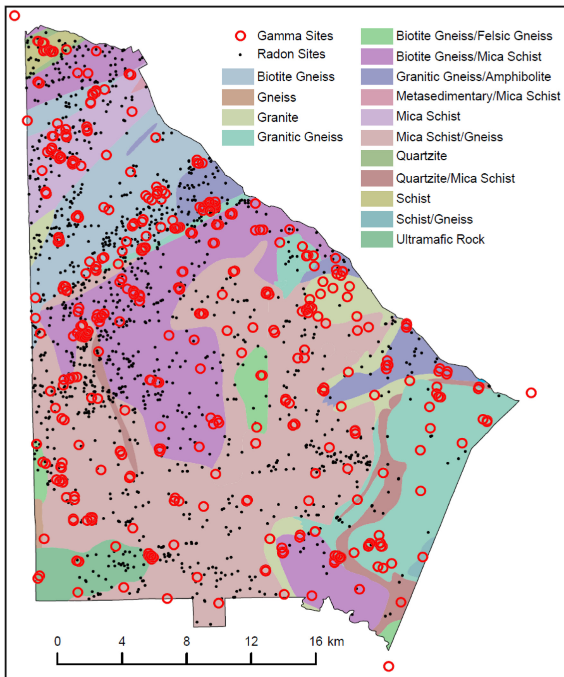
Fig. 2. DeKalb's underlying geology with gamma and radon sample sites highlighted. (Base map from Dicken et al., 2007 with corrections based on Higgins et al., 2003).
