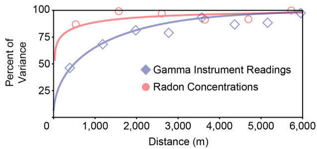
Fig. 4. Semivariograms of gamma readings and indoor radon concentrations.
