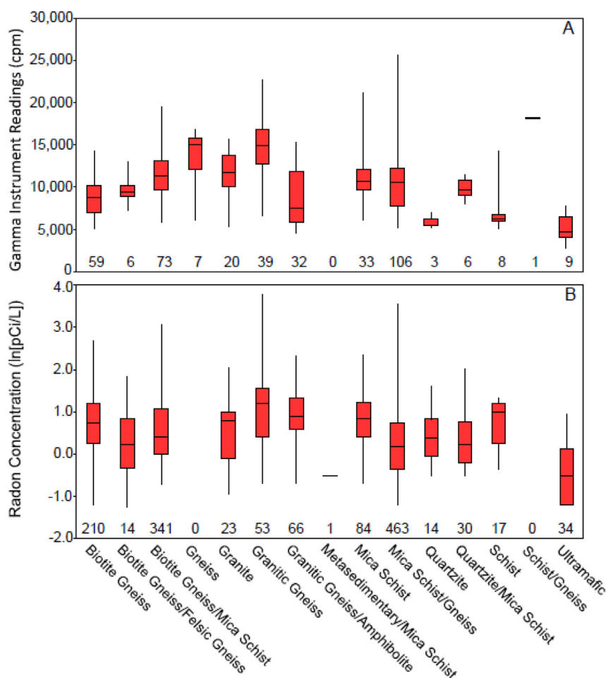
Fig. 3. Box and whisker plots of gamma readings and log-transformed indoor radon concentrations as grouped by bedrock type. The numbers are the sample sizes for each bedrock type.
