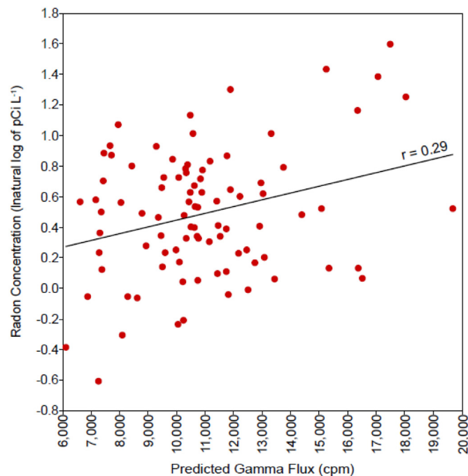
Fig. 7. Scatterplot of log-transformed indoor radon levels and predicted gamma flux with both aggregated to 3 km grid cells.
