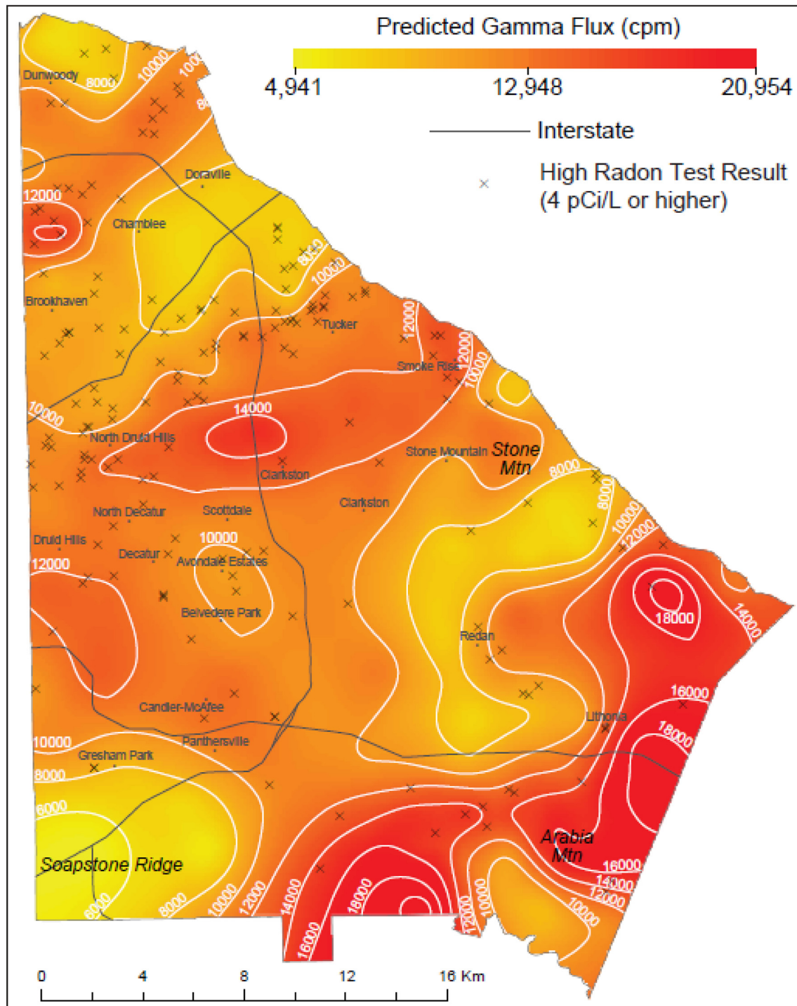
Fig. 5. A map of predicted gamma flux throughout DeKalb.
