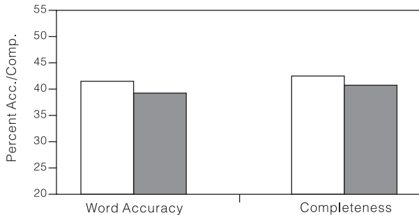
Figure 3 Word accuracy (left) and completeness (right) scores for the net trained with three cues (phon-ub-stress — white bars) and the net trained with two cues (phon-ub — grey bars).
