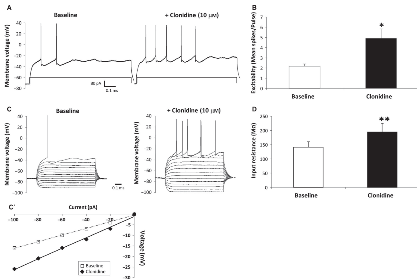
Fig. 1. \alpha_2 -AR-mediated increase in mPFC pyramidal neuron excitability and input resistance. In vitro clonidine (10 \mu\text{M} ) elevated excitability in an individual neuron from 2 to 5 spikes/pulse (A) and significantly elevated mean excitability (B) ( N = 6 cells). Clonidine also elevated membrane input resistance in an individual neuron from 157 to 251 \text{M}\Omega , as shown by voltage responses to a series of hyperpolarising to depolarising current steps (C) and in a current–voltage plot (C'), and significantly elevated mean input resistance (D) ( N = 6 cells). Significant change from baseline by paired Student's t -test (* P < 0.05 , ** P < 0.01 ). Data are represented as mean + SEM.
