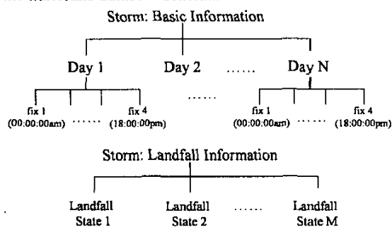
Figure 2. Hierarchy of Hurricane Tracking Data
