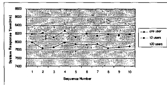
Figure 7. Performance Experiment Result of AHO
