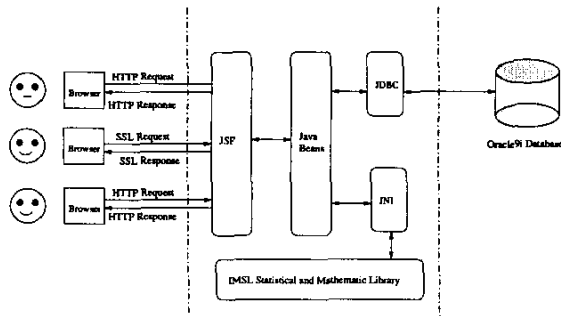
Figure 1. Illustration of the Overall System Architecture
