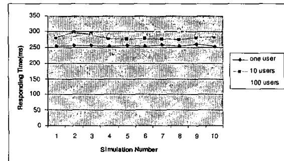
Figure 8. Performance Experiment Result of SGT
