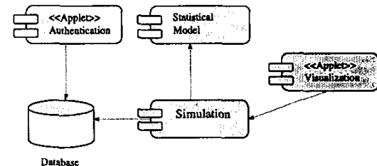
Figure 4. Component Diagram for AHO
