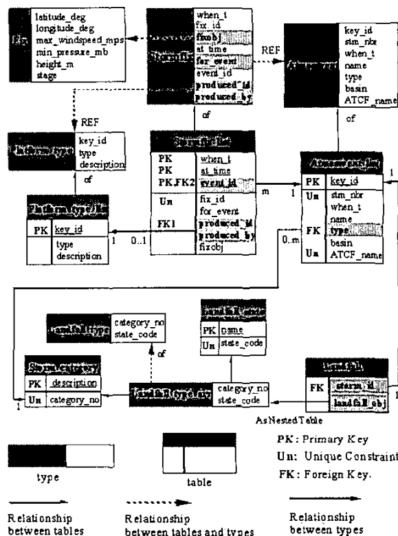
Figure 3. Database Schema
