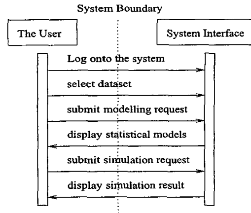
Fig. 2. Interaction flow between the user and the system
