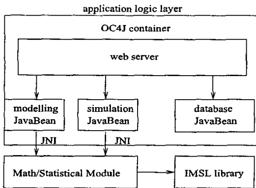
Fig. 4. Basic structure of application logic layer
