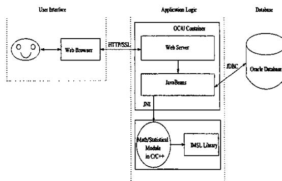
Fig. 1. Detailed architecture of the system
