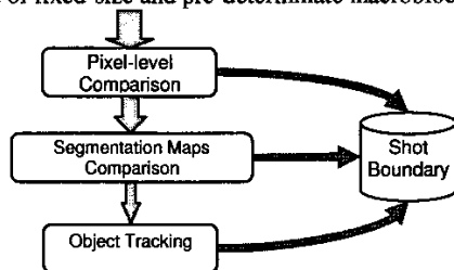
Figure 3: The workflow of the proposed method.
