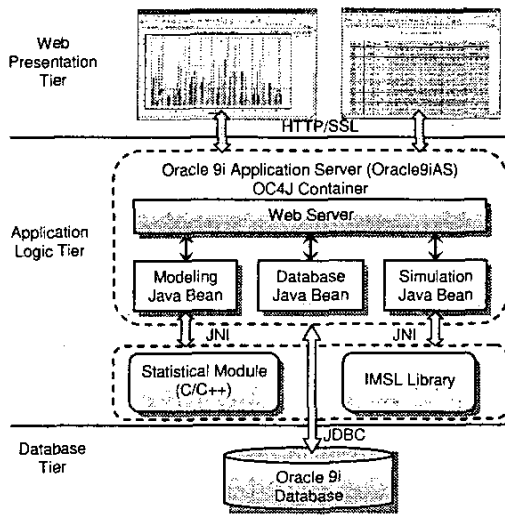
Figure 1. System architecture
