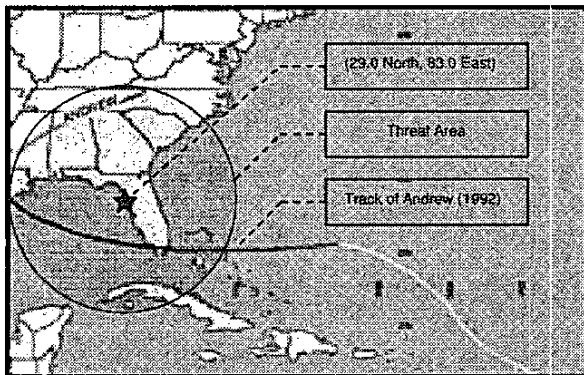
Figure 3. Threat area and the storm track of hurricane Andrew 1992
