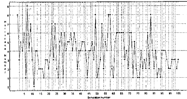
Figure 4. Simulated 100-year annual hurricane occurrence distribution
