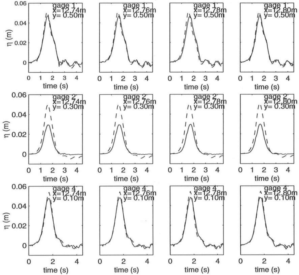
Figure A.3: Time series of surface elevations for x = 12.74 - 12.80 m and H = 5.48 cm. The solid line is the experimental data and the dashed line is model results.
