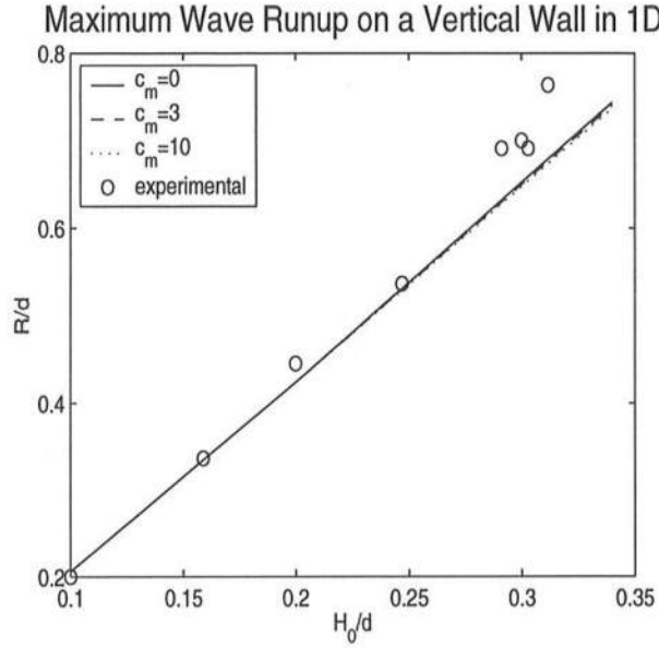
Figure 2.6: Wave runup vs. incident wave height. Nine numerical tests were carried out, three different wave heights ( H = 3, 6 , and 10\text{ cm} ) for each of three mixing coefficients ( c_m = 0, 3 , and 10 ). Circles represent experimental data from Chan and Street (1970).
