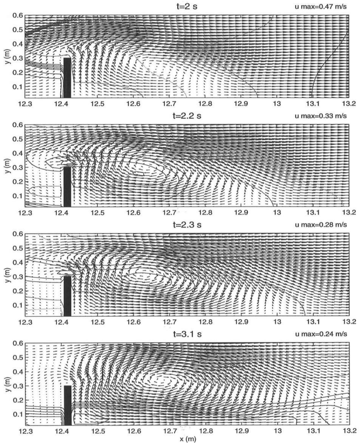
Figure 3.15: Contours of surface elevation (m) with velocity vectors from the model for H = 10.3 cm at t = 2.0 - 3.1 s.
