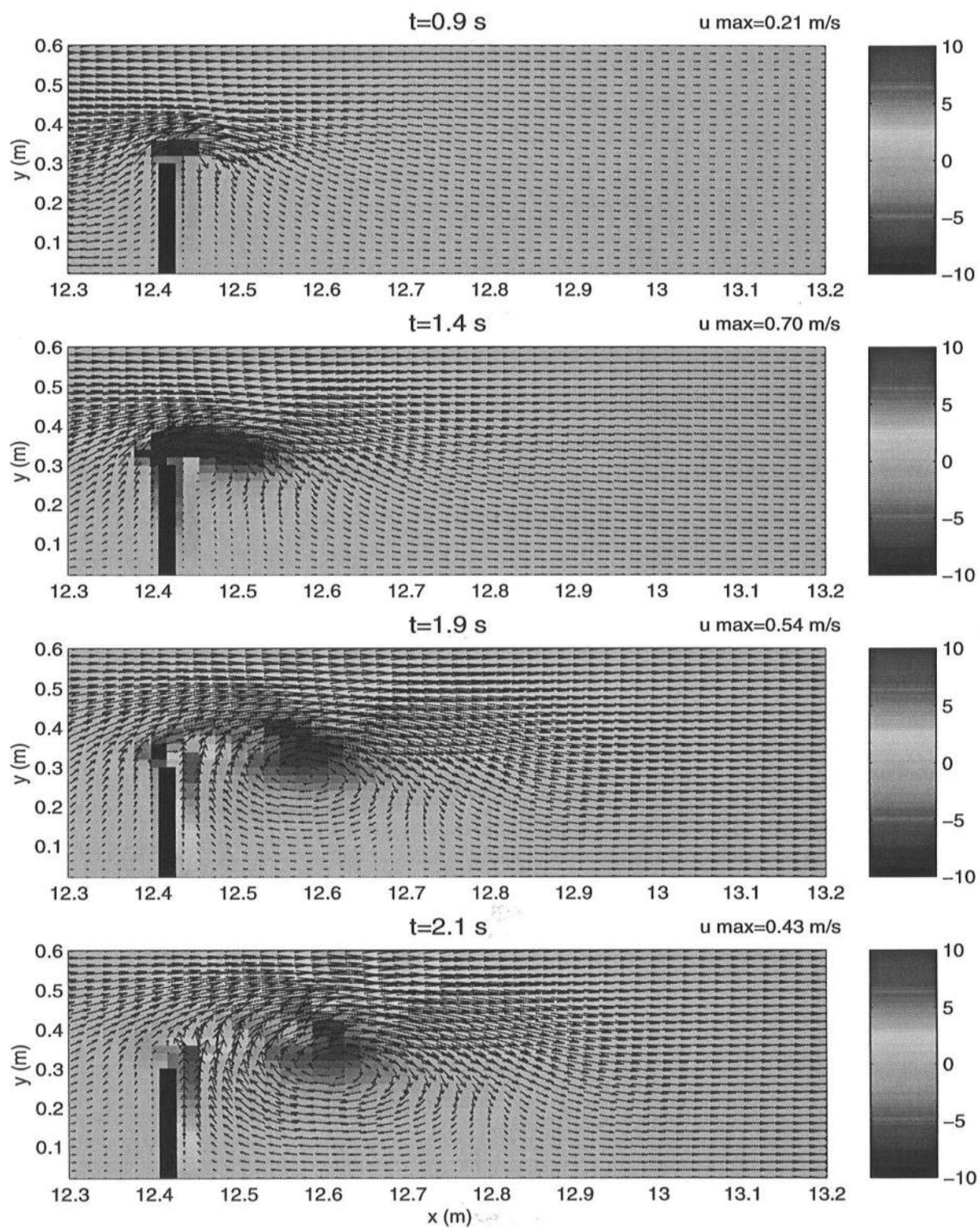
Figure 3.16: Velocity vectors overlaid on the vorticity field for H = 5.48 cm. Color-bars give the vorticity in units of s^{-1} .
