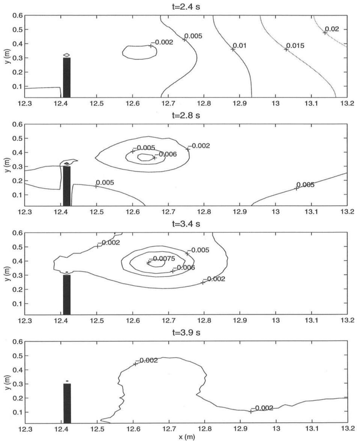
Figure 3.5: Contours of surface elevation (m) from the model data for H = 5.48 cm at four instances in time.
