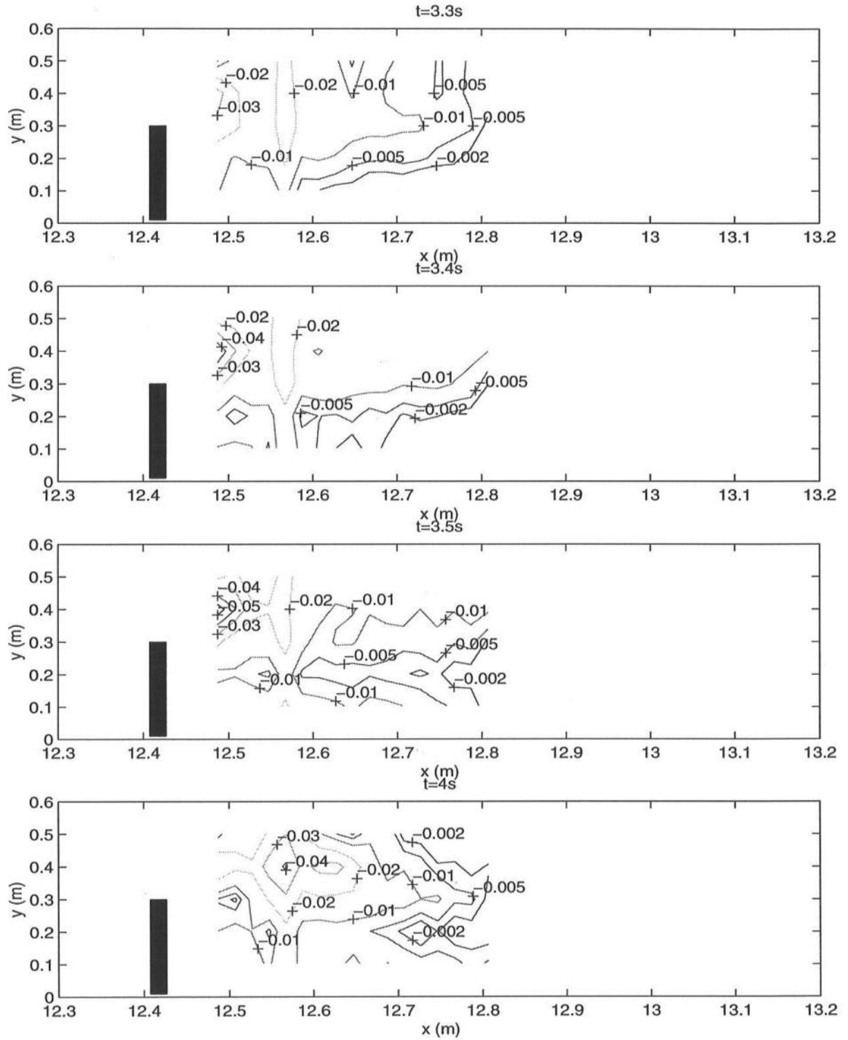
Figure 3.10: Contours of surface elevation (m) from the experimental data for H = 10.3 cm at t = 1.5 - 1.8 s.
