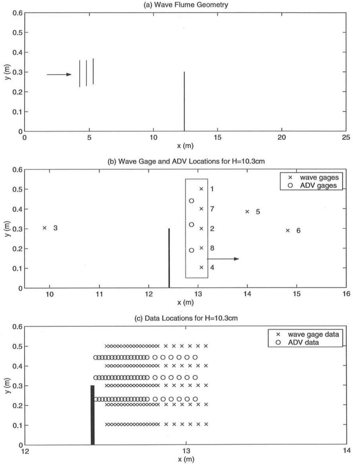
Figure 2.4: (a) Wave flume, (b) gage locations, and (c) data locations for H = 10.3 cm.
