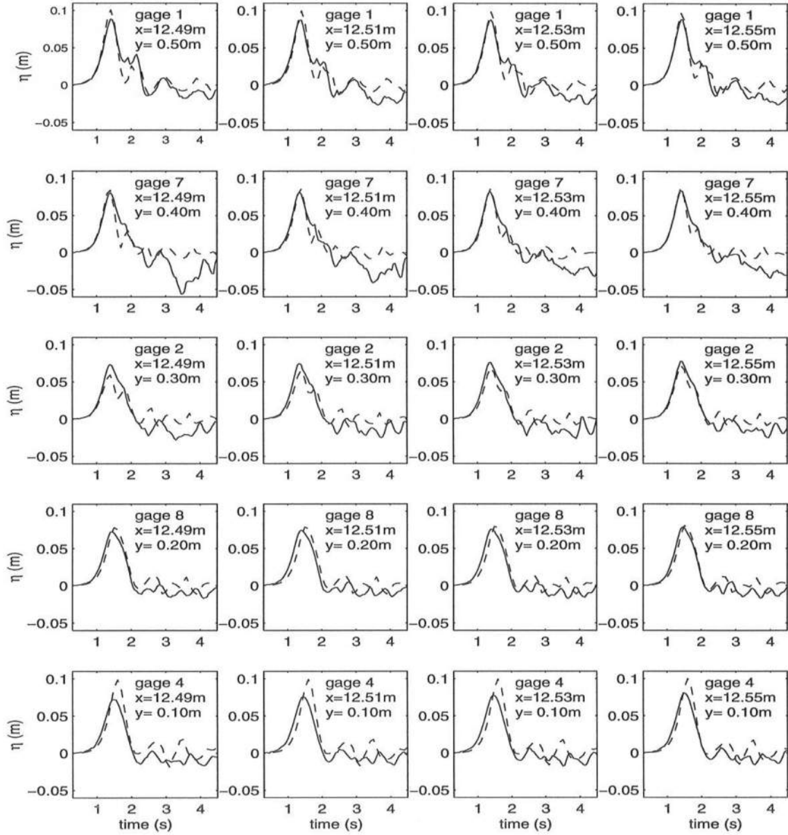
Figure B.1: Time series of surface elevations for x = 12.49 - 12.55\text{ m} and H = 10.3\text{ cm} . The solid line is the experimental data and the dashed line is model results.
