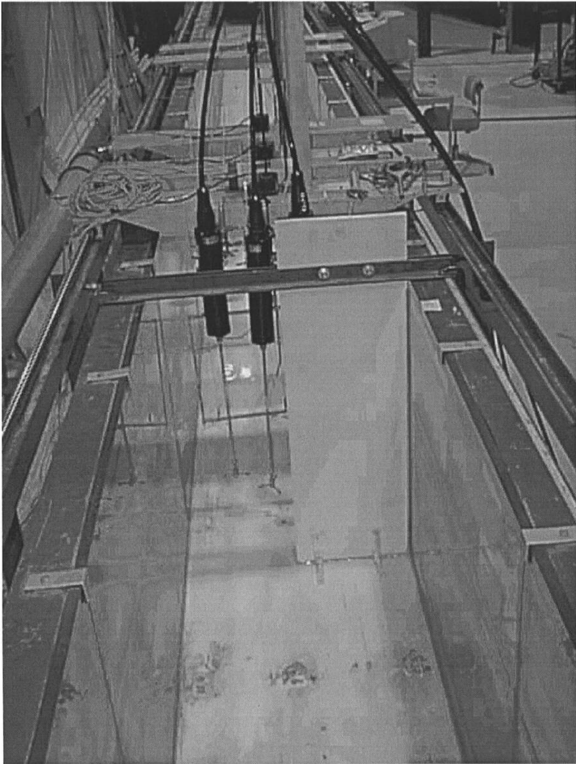
Figure 2.2: Digital photograph showing the breakwater and instrument setup.
