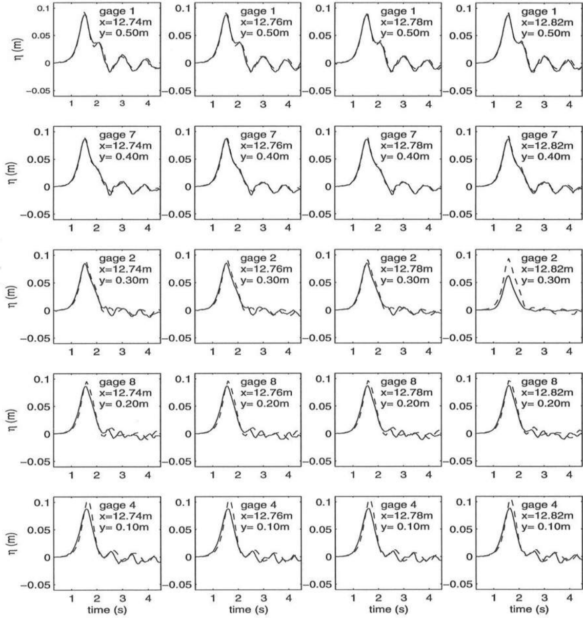
Figure B.4: Time series of surface elevations for x = 12.74 - 12.82\text{ m} and H = 10.3\text{ cm} . The solid line is the experimental data and the dashed line is model results.
