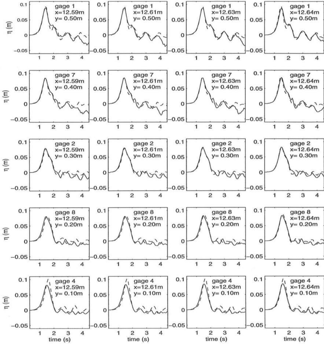
Figure B.2: Time series of surface elevations for x = 12.59 - 12.64\text{ m} and H = 10.3\text{ cm} . The solid line is the experimental data and the dashed line is model results.
