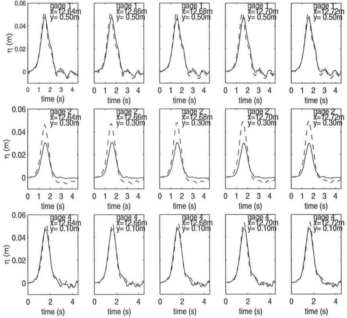
Figure A.2: Time series of surface elevations for x = 12.64 - 12.72 m and H = 5.48 cm. The solid line is the experimental data and the dashed line is model results.
