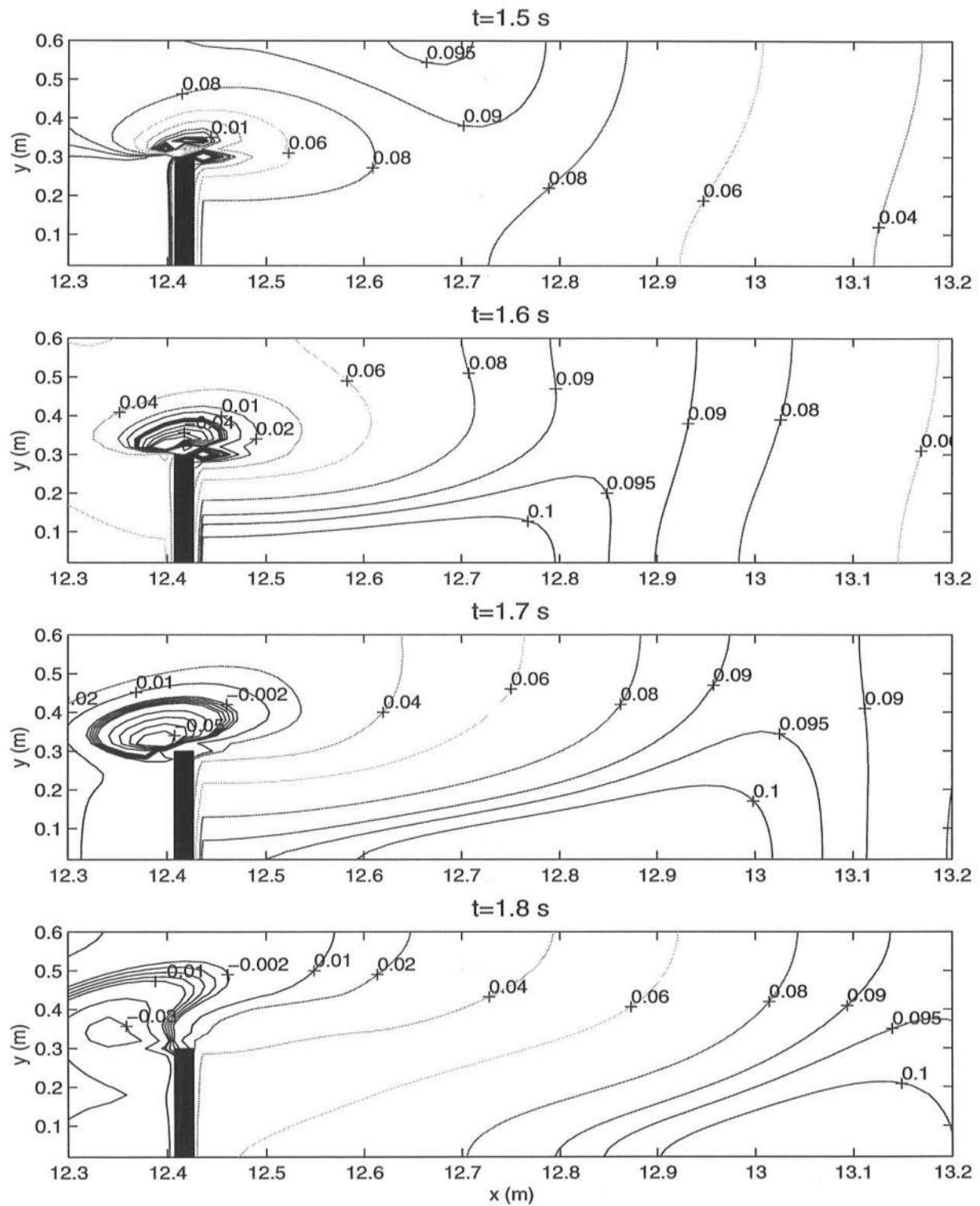
Figure 3.12: Contours of surface elevation (m) from the model for H = 10.3 cm at t = 1.5 - 1.8 s.
