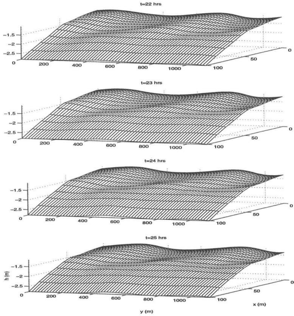
Figure 6.21: 3D snapshots of the topography for k = 1.14 with constant forcing terms in the momentum equations. The flow is from left to right.
