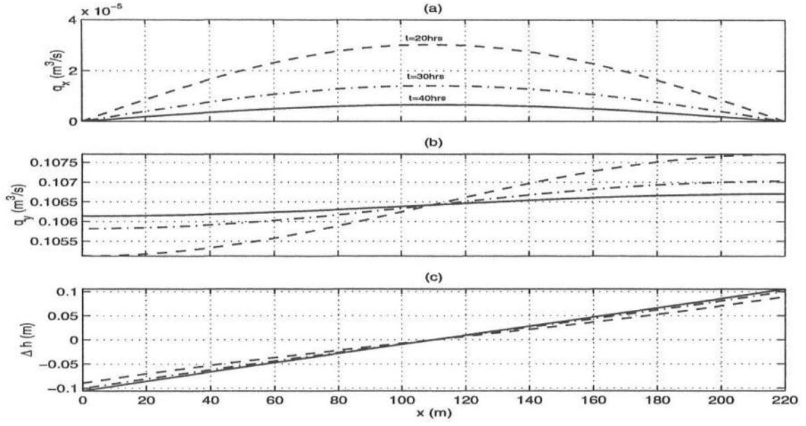
Figure 5.2: Cross-channel profiles of (a) cross-channel sediment transport rate, (b) along-channel sediment transport rate and (c) depth change at different time levels.
