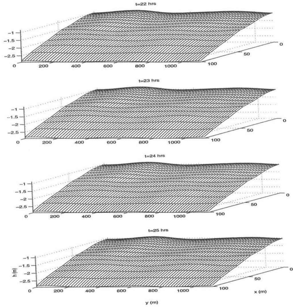
Figure 6.17: 3D snapshots of the topography for k = 1.14 . The flow is from left to right (continued).
