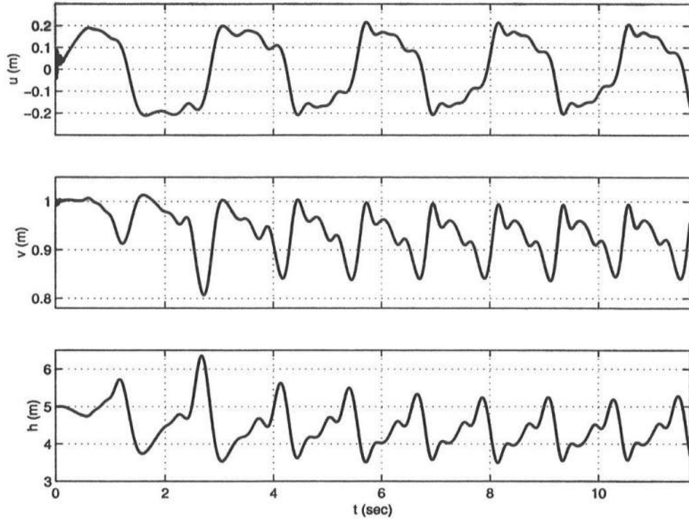
Figure 5.30: Time series of u , v and h at (x, y) = (110m, 0.5L_y) for k = 3.1 and c_f = 0.03 .
