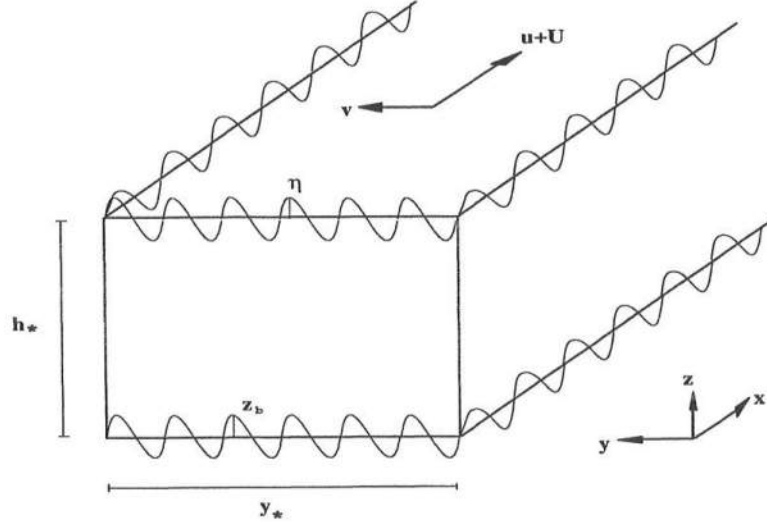
Figure 2.1: Sketch of the physical layout: rectangular channel.
