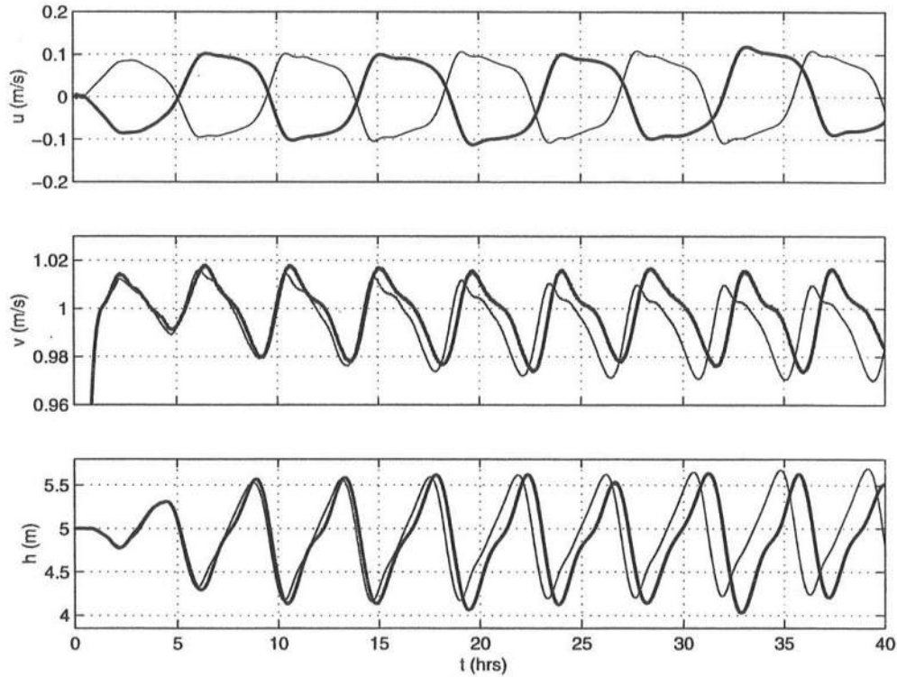
Figure 5.20: Time series of u , v and h at (x, y) = (110m, 0.5L_y) for k = 1.35 . (—) L_y = 2\lambda_y , (---) L_y = \lambda_y
