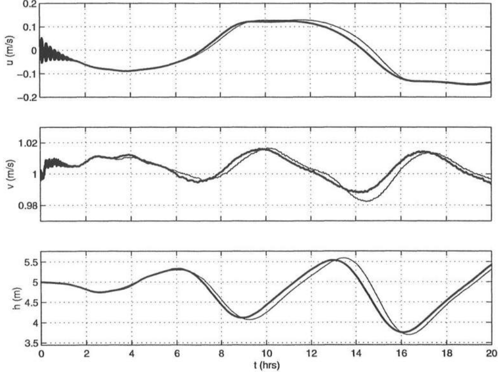
Figure 5.14: Time series of u , v and h at (x, y) = (110m, 0.5L_y) for (—) L_y = 4\lambda_y and (---) L_y = 2\lambda_y .
