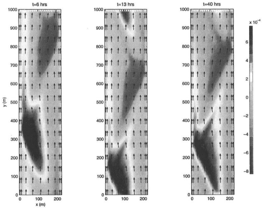
Figure 5.19: Snapshots of the velocity field on top of the vorticity for L_y = \lambda_y , k = 1.35 .
