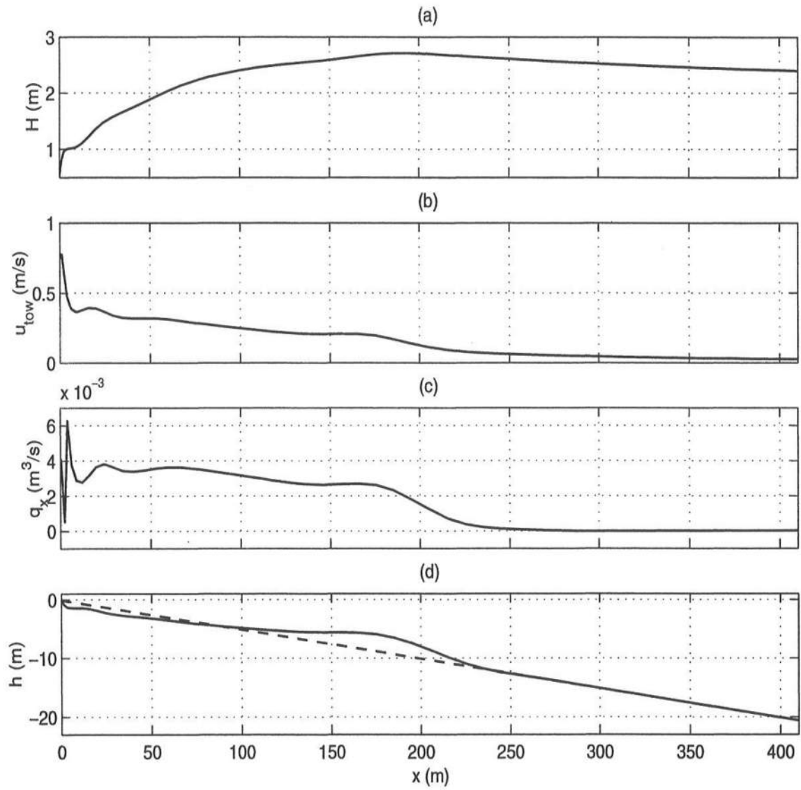
Figure 7.3: Cross-shore profiles at t = 25\text{hrs} . (a) Wave height, (b) Undertow, (c) Sediment transport rate, (d) Topography.
