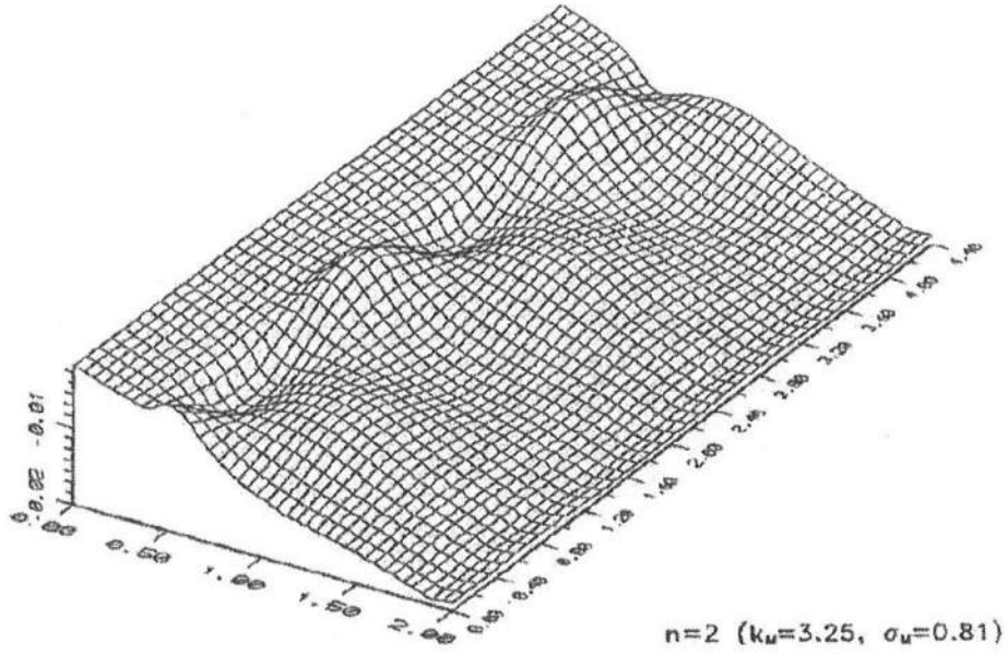
Figure 2.6: Bottom topography for modes 1 and 2. R = 1 , m = 0.01 , F = 0.3 (from Falquès et al. , 1996a).
