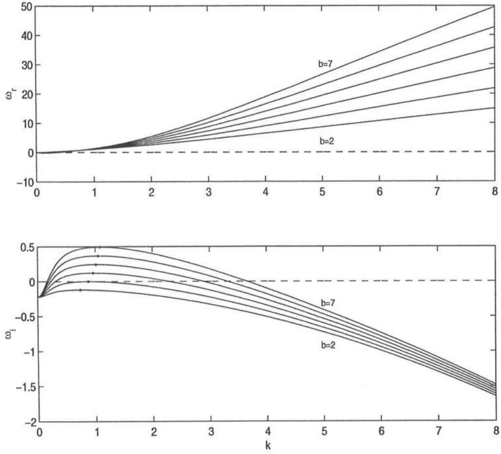
Figure 3.7: 2D channel dispersion curves for b = 2 - 7 with parameters: U = 1\text{ m/s} , R = 44 , v_c = 0 , \gamma' = 1 , c_f = 0.003 .
