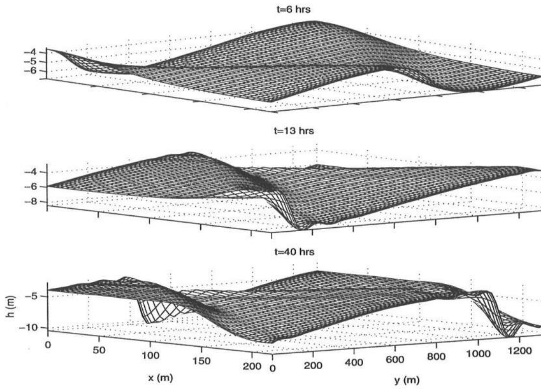
Figure 5.7: Snapshots of simulated bed evolution in 3D for L_y = \lambda_y , k_{max} = 1.05 .
