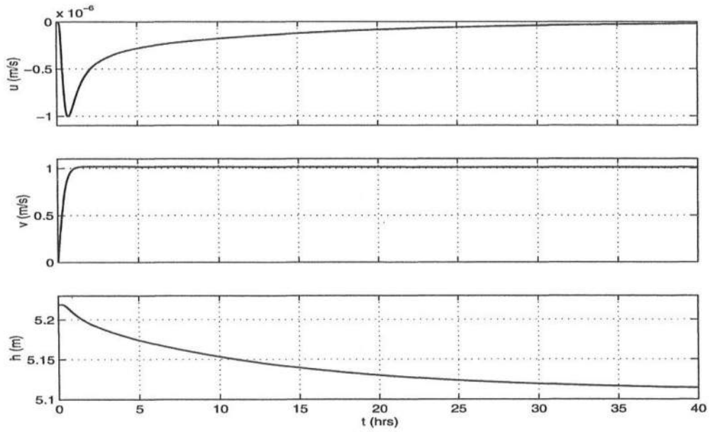
Figure 5.3: Time series of u , v and h at (x, y) = (219\text{m}, 0.5L_y) for test case.
