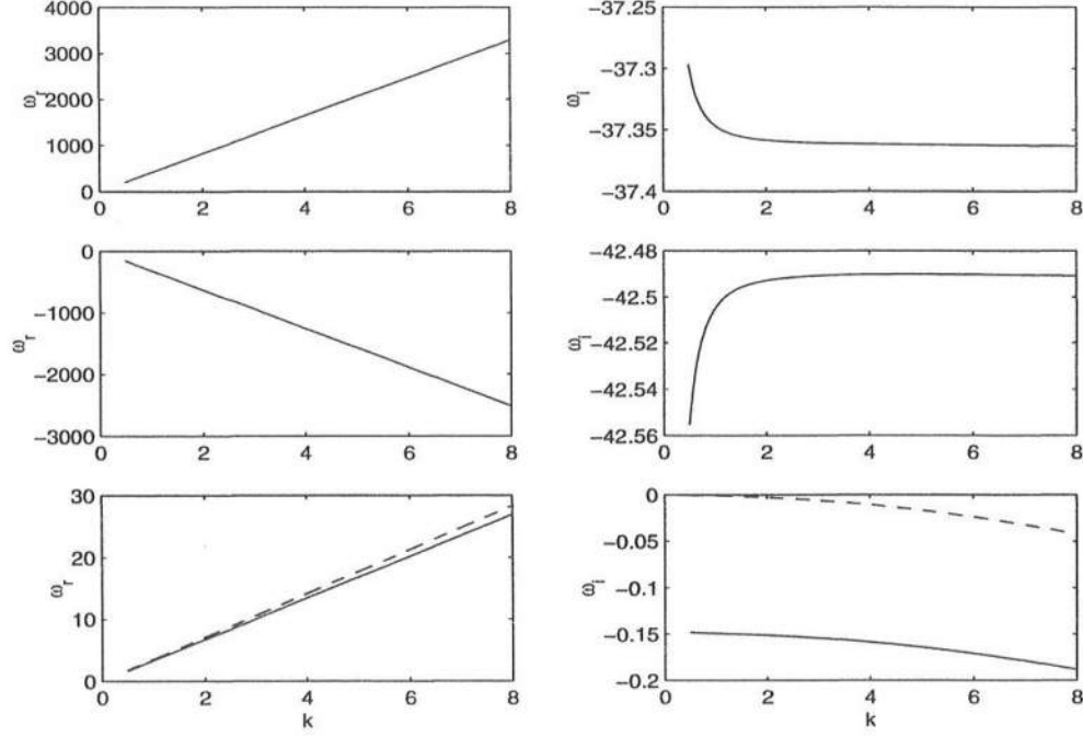
Figure 3.3: A comparison between dispersion curves for a 1D channel with parameters: U = 1m/s , b = 6 , v_c = 0.1m/s , \gamma' = 1 , h_* = 5m , x_* = 4000m , c_f = 0.001 . (—) results without assumptions,(- -) results with assumptions.
