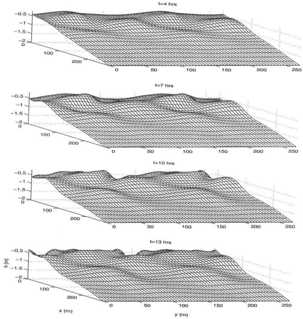
Figure 6.11: 3D view of the topography for k = 3.25 with constant momentum forcing terms. The flow is from left to right.
