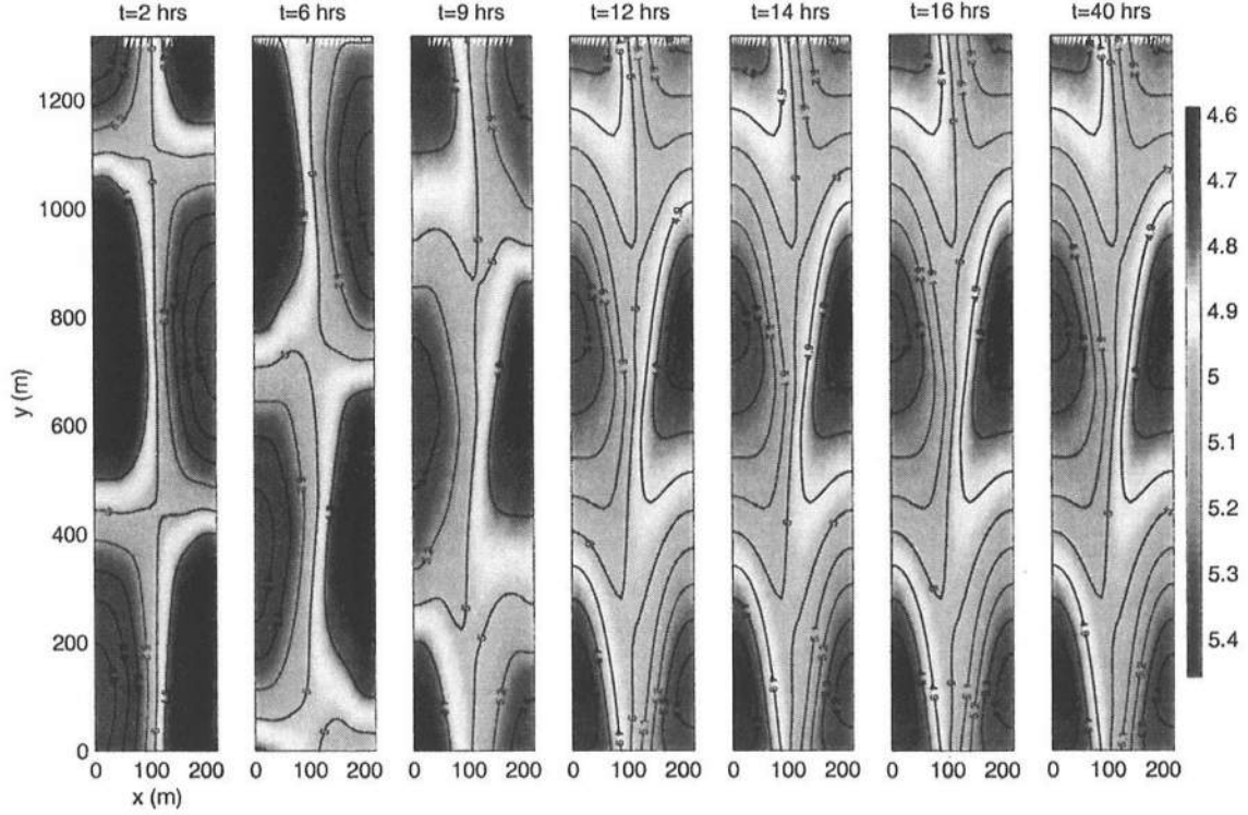
Figure 5.32: Snapshots of the bed evolution for k = 1.05 and b = 2 .
