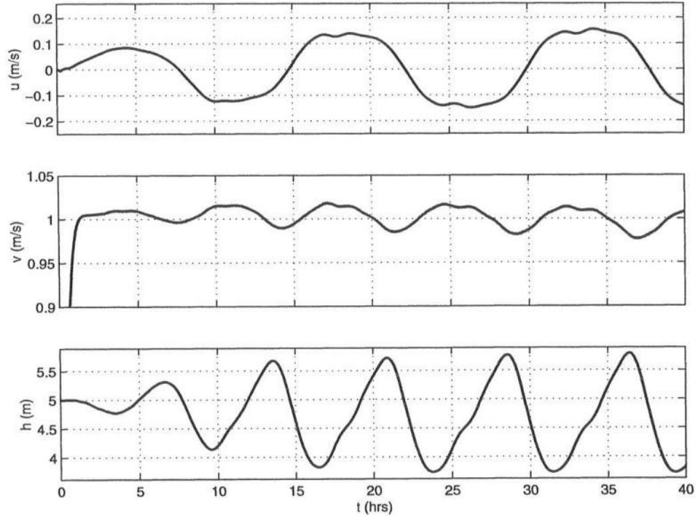
Figure 5.9: Time series of u , v and h at (x, y) = (110\text{m}, 0.5L_y) for L_y = \lambda_y .
