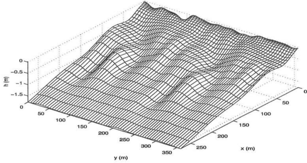
Figure 6.7: 3D view of the topography for k = 3.25 at t = 7.5 hours. Initial bed perturbation located around x = 100m . The flow is from left to right
