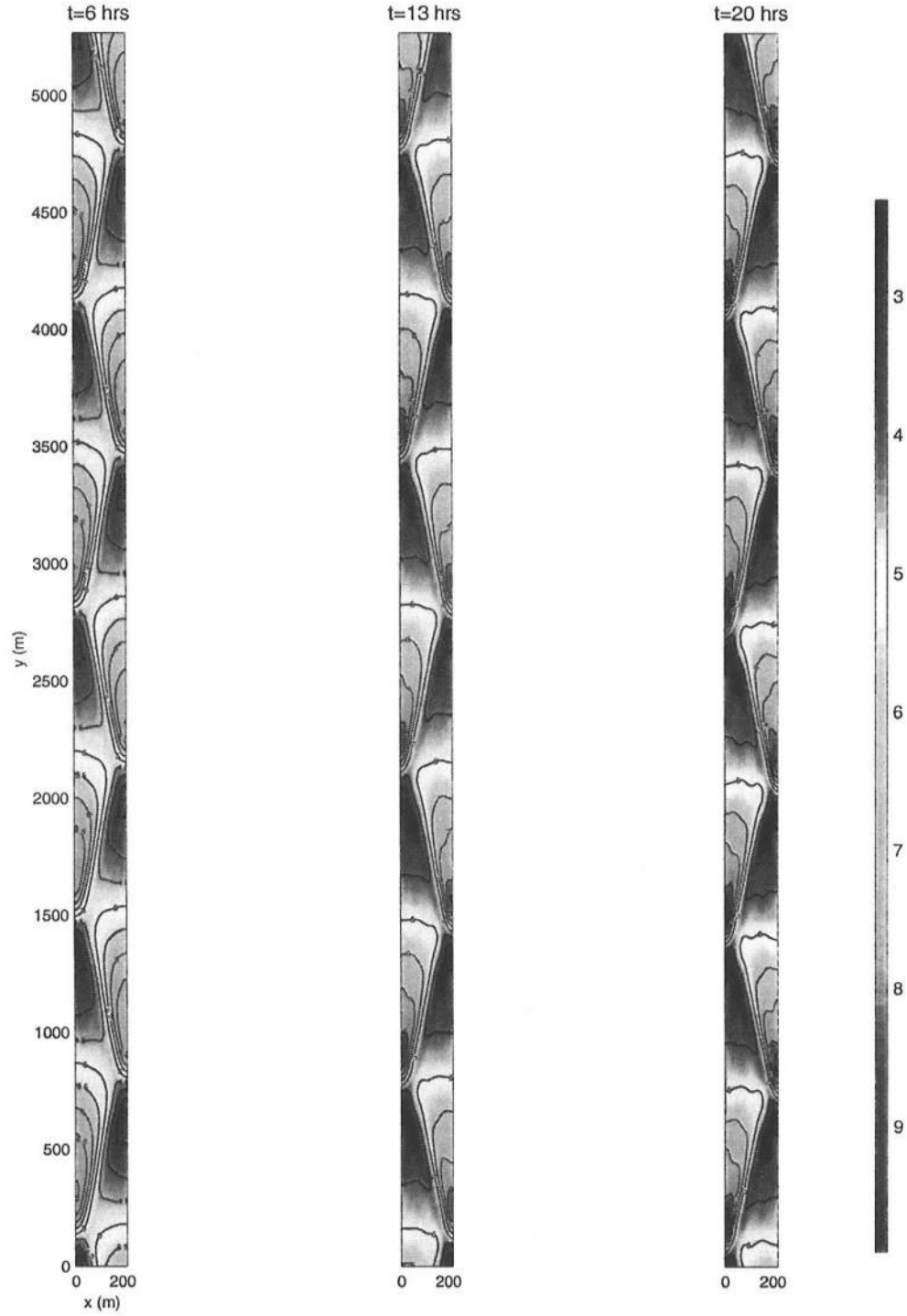
Figure 5.15: Simulated bed evolution for L_y = 4\lambda_y , k = 1.05 .
