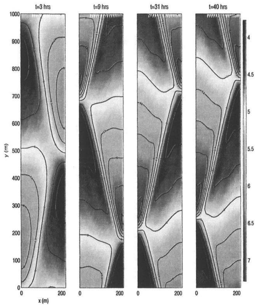
Figure 5.18: Simulated bed evolution for L_y = \lambda_y , k = 1.35 .
