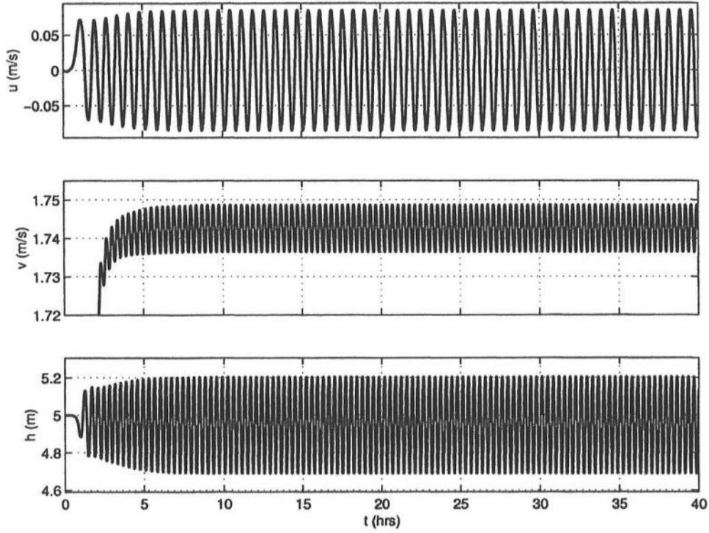
Figure 5.28: Time series of h at (x, y) = (110m, 0.5L_y) for k = 1.05 and c_f = 0.001 .
