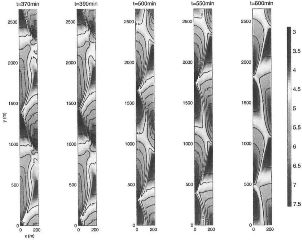
Figure 5.35: Snapshots of the bed evolution for k = 1.05 with K = 2 in the bed perturbation (continued).
