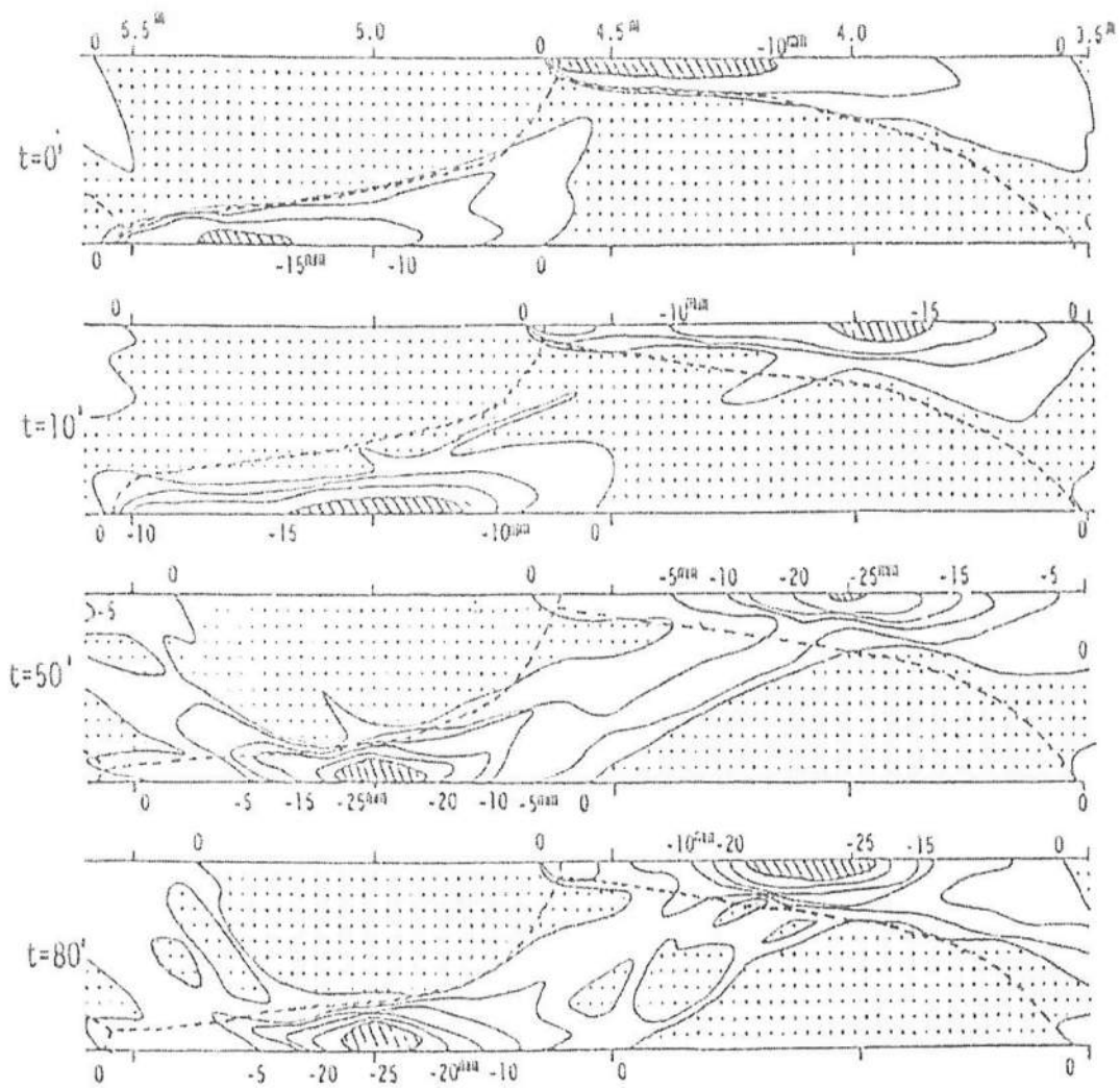
Figure 5.37: Alternate bar deformation in a laboratory flume (Uchijima, 1990). Hatched sections: scour, smudged sections: high bed level. The dashed line represents the barfront.
