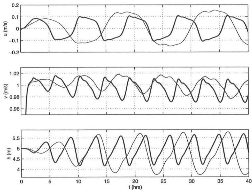
Figure 5.17: Time series of u , v and h at (x, y) = (110m, 0.5L_y) for L_y = \lambda_y . (—) k = 1.35 , (---) k = 1.05
