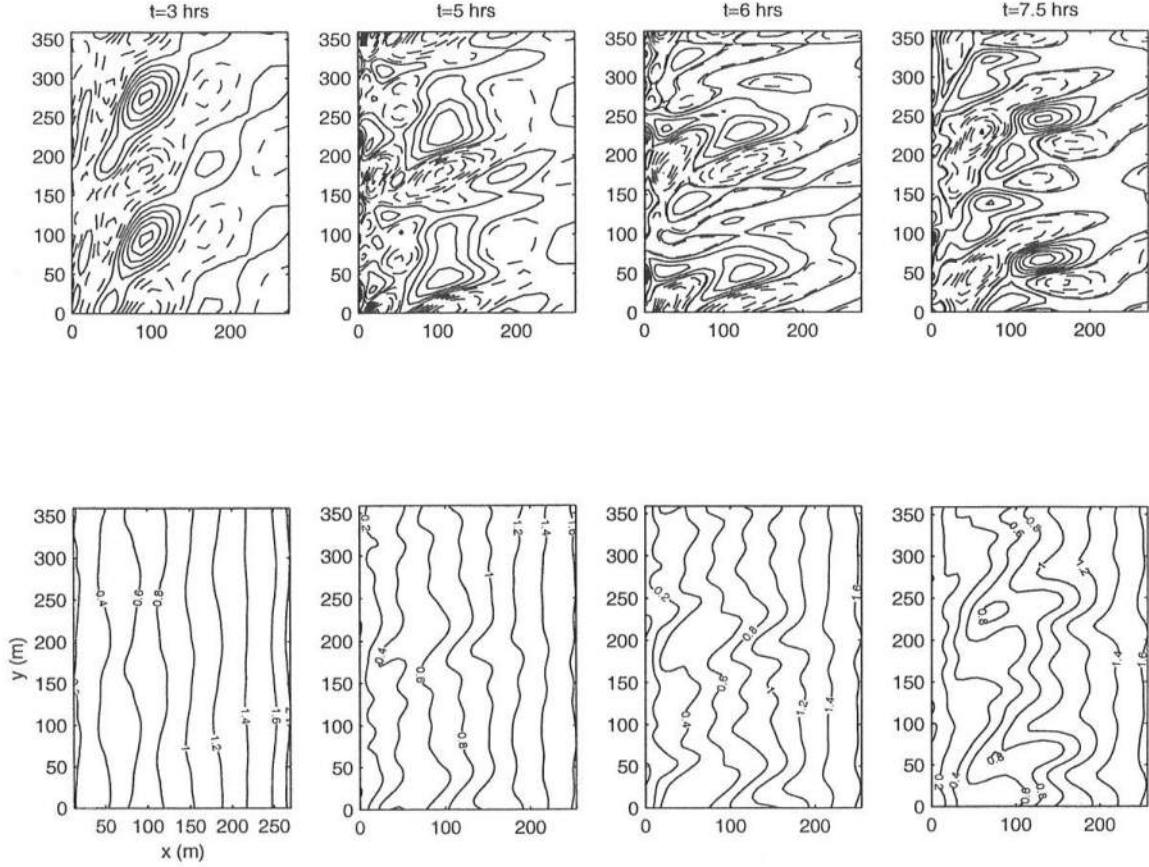
Figure 6.6: Simulated bed evolution for k = 3.5 , m = 0.006 , H_o = 0.3727m , \theta_o = 6.9^\circ , T = 7.7s , c_f = 0.003 . Initial bed perturbation located around x = 100m . Top panel: bed change contours (dashed lines: erosion, solid lines: deposition). Bottom panel: topography.
