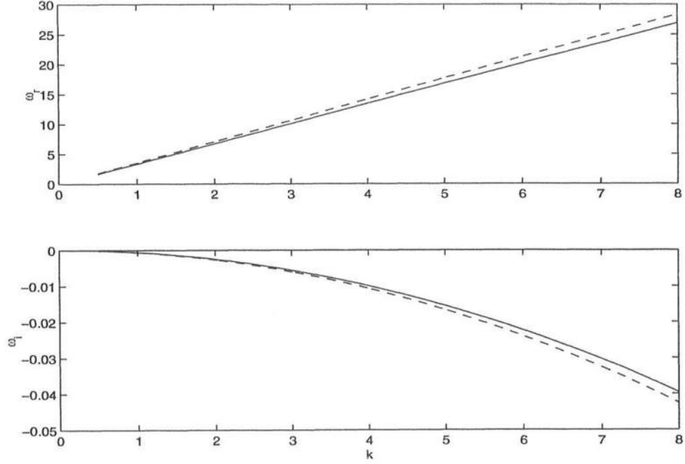
Figure 3.4: A comparison between dispersion curves for a 1D channel with parameters: U = 1m/s , b = 6 , v_c = 0.1m/s , \gamma' = 1 , h_* = 5m , x_* = 4000m , c_f \approx 0.0 . (—) results without assumptions, (---) results with assumptions.
