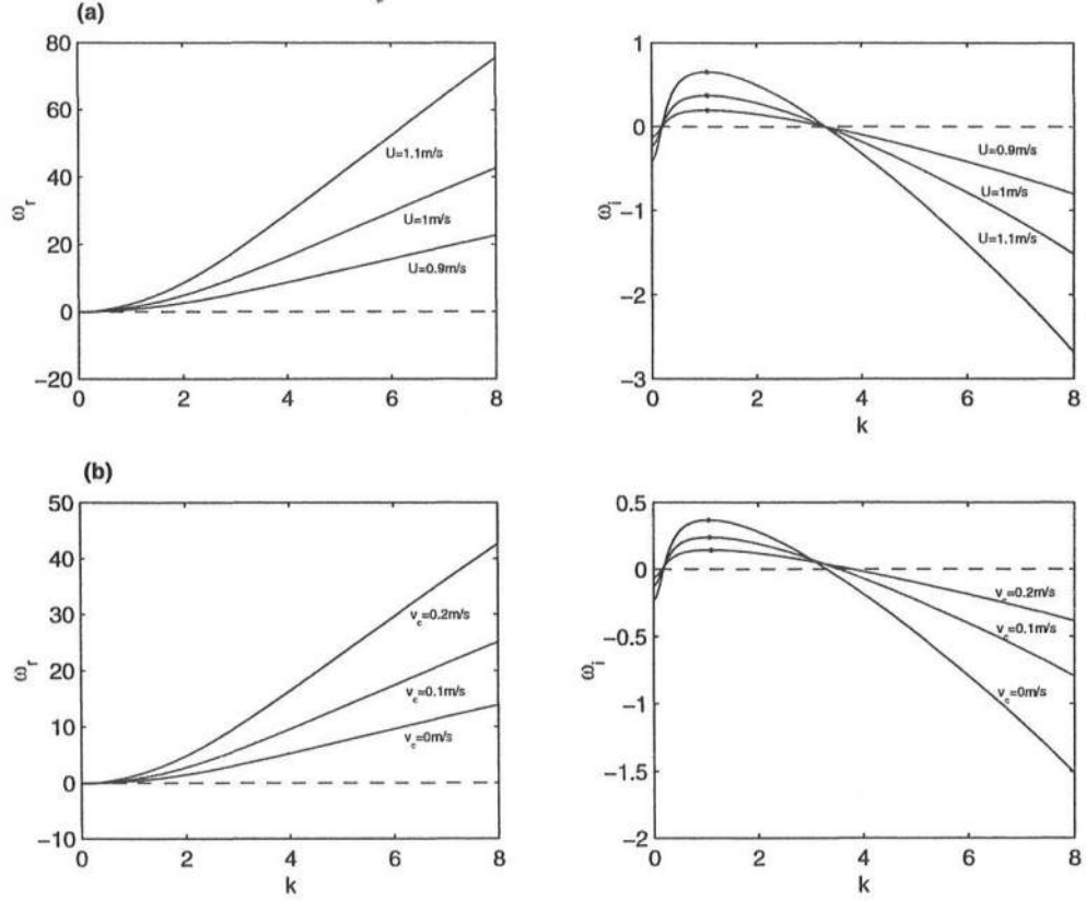
Figure 3.9: 2D channel dispersion curves for different ranges of U and v_c values, with parameters: R = 44 , b = 6 , \gamma' = 1 , c_f = 0.003 , (a) v_c = 0 , (b) U = 1 m/s.
