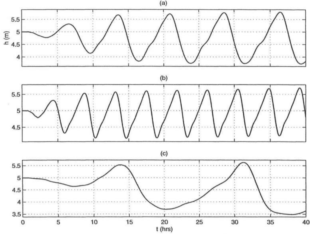
Figure 5.23: Time series of h at (x, y) = (110m, 0.5L_y) for (a) k = 1.05 , (b) k = 1.35 , (c) k = 0.67 .
