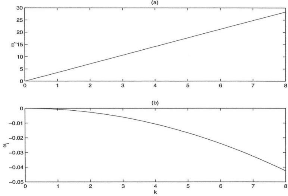
Figure 3.2: Dispersion curves for a 1D channel, with parameters: U = 1m/s , b = 6 , v_c = 0.1m/s , \gamma' = 1 , h_* = 5m , x_* = 4000m .
