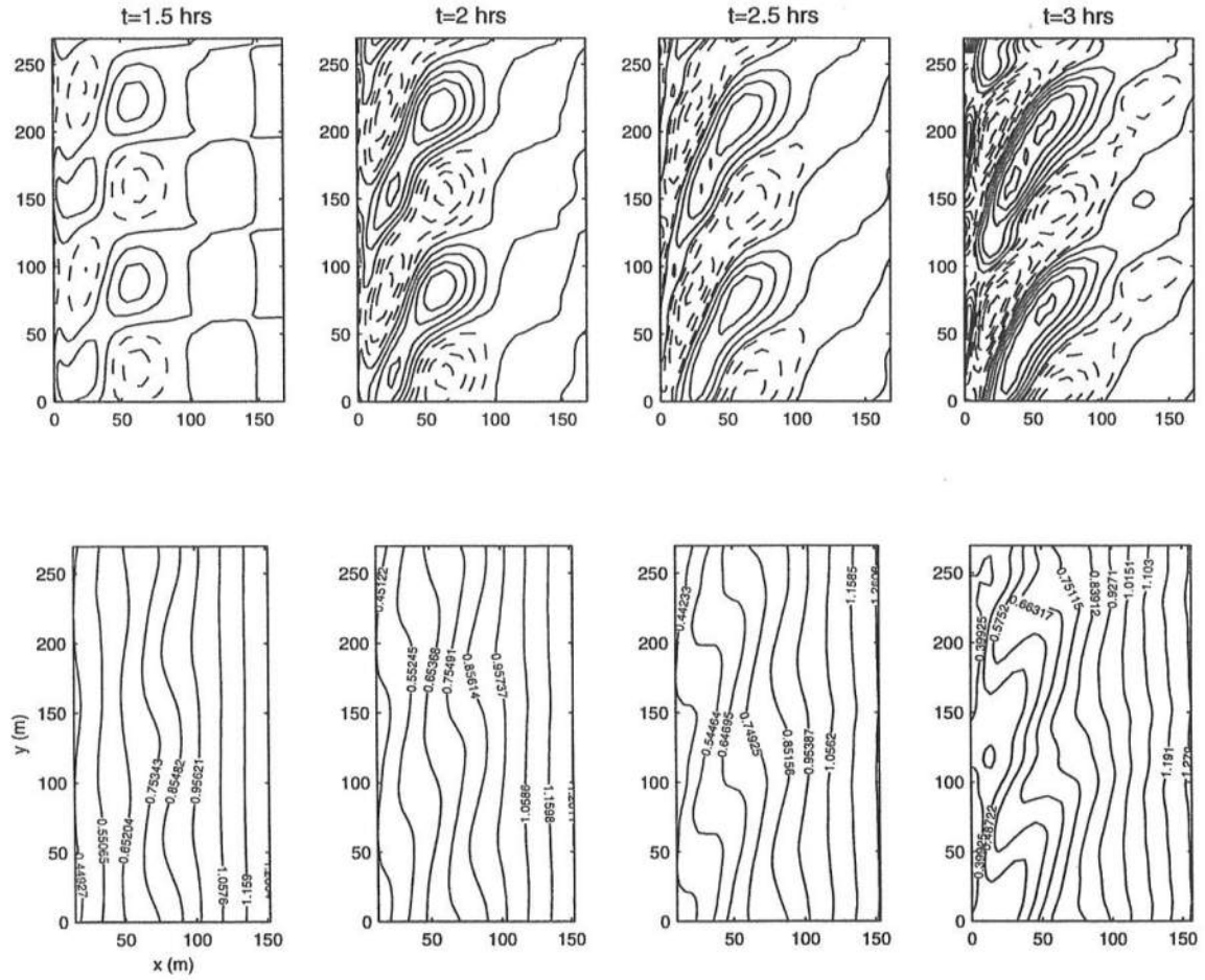
Figure 6.1: Simulated bed evolution for k = 3.5 , m = 0.006 , H_o = 0.3727m , \theta_o = 6.9^\circ , f = 0.13 \text{ rad/s} , c_f = 0.003 . Top panel: bed change contours (dashed lines: erosion, solid lines: deposition). Bottom panel: topography.
