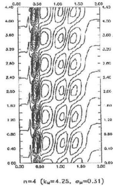
Figure 2.5: Contour lines of bed perturbation for modes 1,2,3 and 4. R = 1 , m = 0.01 , F = 0.3 (from Falquès et al. , 1996a).
