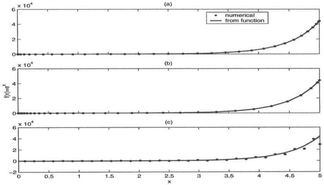
Figure 4.4: Comparison of three transformations used in the model for f(x) = e^x . (a) Transformation (4.29), (b) Transformation (4.30), (c) Transformation (4.31).
