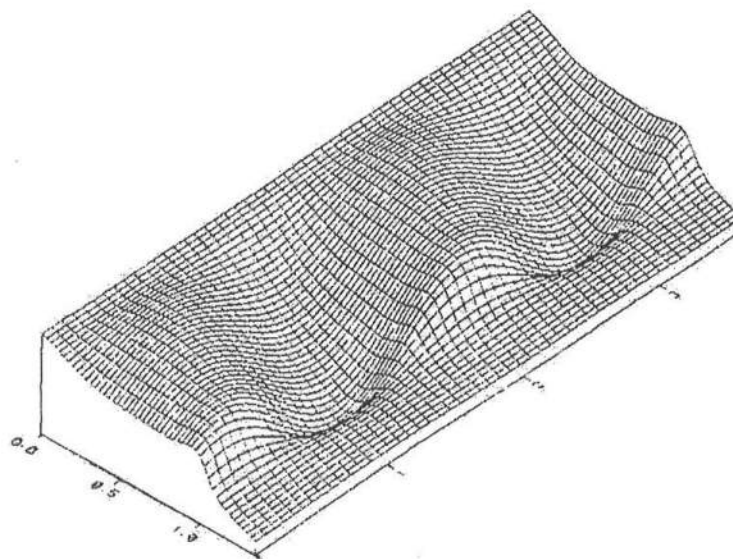
Figure 2.8: Wave dominated bottom topography for R = 0.5 , \alpha_b = 12.3^\circ , N = 0.005 , \gamma_b = 0.4 , F = 0.16 , k = 3.5 (from Falqués et al. , 1996b).
