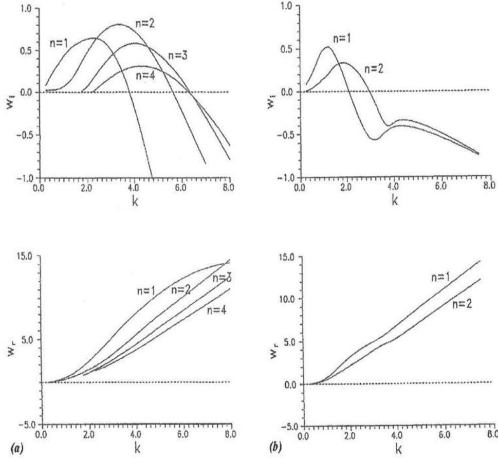
Figure 2.4: Dispersion curves, for different modes. F = 0.3 , m = 0.01 , (a) R = 1 , (b) R = 0.35 (from Falquès et al. , 1996a).
