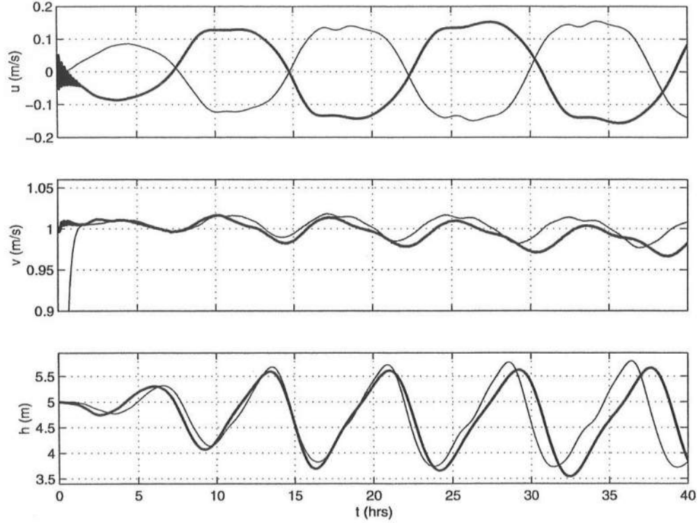
Figure 5.11: Time series of u , v and h at (x, y) = (110m, 0.5L_y) for (—) L_y = 2\lambda_y and (---) L_y = \lambda_y .
