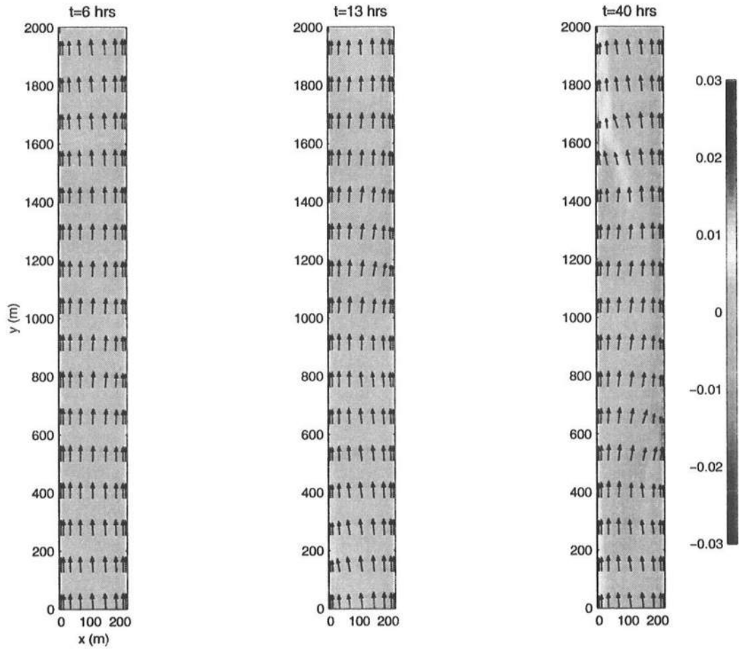
Figure 5.26: Snapshots of the flow field and corresponding vorticity for L_y = \lambda_y , k = 0.67 .
