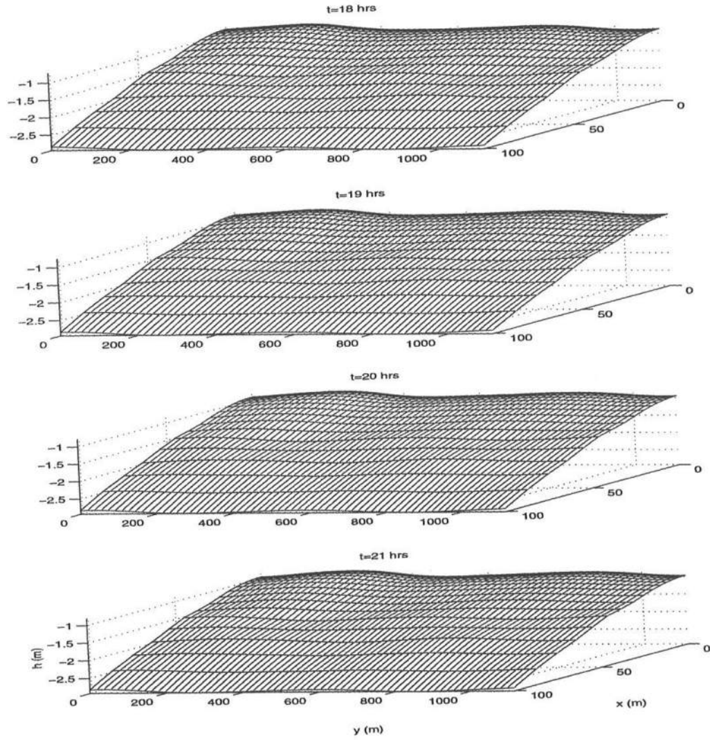
Figure 6.16: 3D snapshots of the topography for k = 1.14 . The flow is from left to right.
