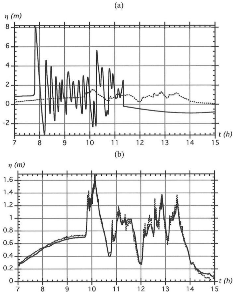
Fig. 16: Simulation with FUNWAVE-TVD (MHW+SLR reference level) of the calibrated M2 tide plus CVV tsunami (TT1 phase situation). Time series of surface elevation at: (a) SE corner (solid) and NOAA station #2 Sewells Pt (dashed), in 154 m grid (Fig. 2); (b) at NOAA station #2 Sewells Pt, in 154 m grid (solid) and in 39 m grid (Fig. 3) (dashed). Time is from the start of the CVV event
