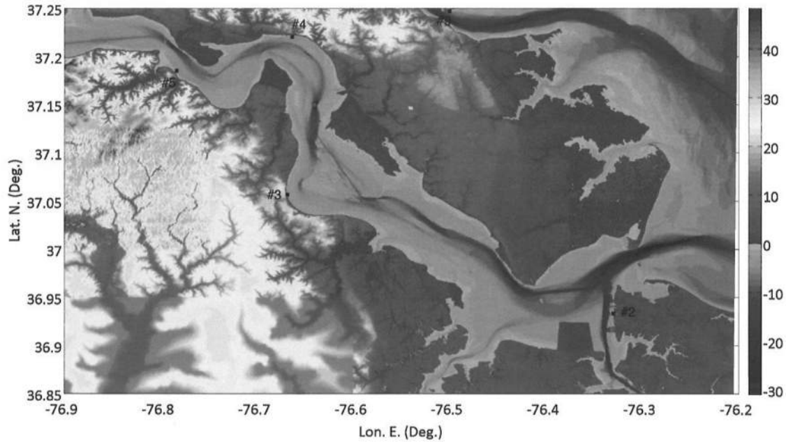
Fig. 3: James River in area of the 39 m Cartesian grid used in FUNWAVE-TVD simulations (Table 4). Bathymetry/topography (in meter) is from 10 m NTHMP and FEMA DEMs (referred to MHW level). The black boxes mark locations of NOAA tide gages (Table 5), and the red circle is the “river station”.
