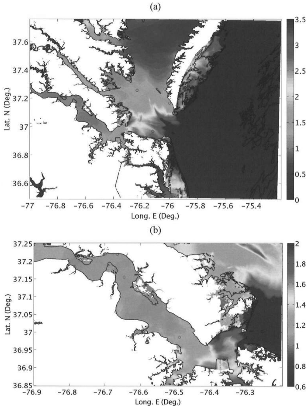
Fig. 18: Simulation with FUNWAVE-TVD (MHW+SLR reference level) of the calibrated M2 tide plus CVV tsunami (TT1 phase situation). Envelope of maximum surface elevation in: (a) 154 m grid; (b) 39 m grid. Circles mark locations of the NOAA stations (Table 5) and the “river station”; solid circle symbol is Sewells Point (Station #2).
