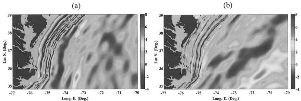
Fig. 9. Surface elevation (color scale in meter) computed at t = (a) 8h 20 min.; and (b) 9h 20 min., in FUNWAVE-TVD simulation of the 450 \text{ km}^3 CVV flank collapse in 20 arc-sec grid (Figs. 1, 2; Table 2).
