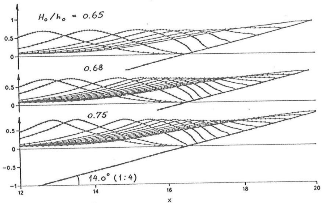
Figure 8: Waves Close to a Surging Breaking
