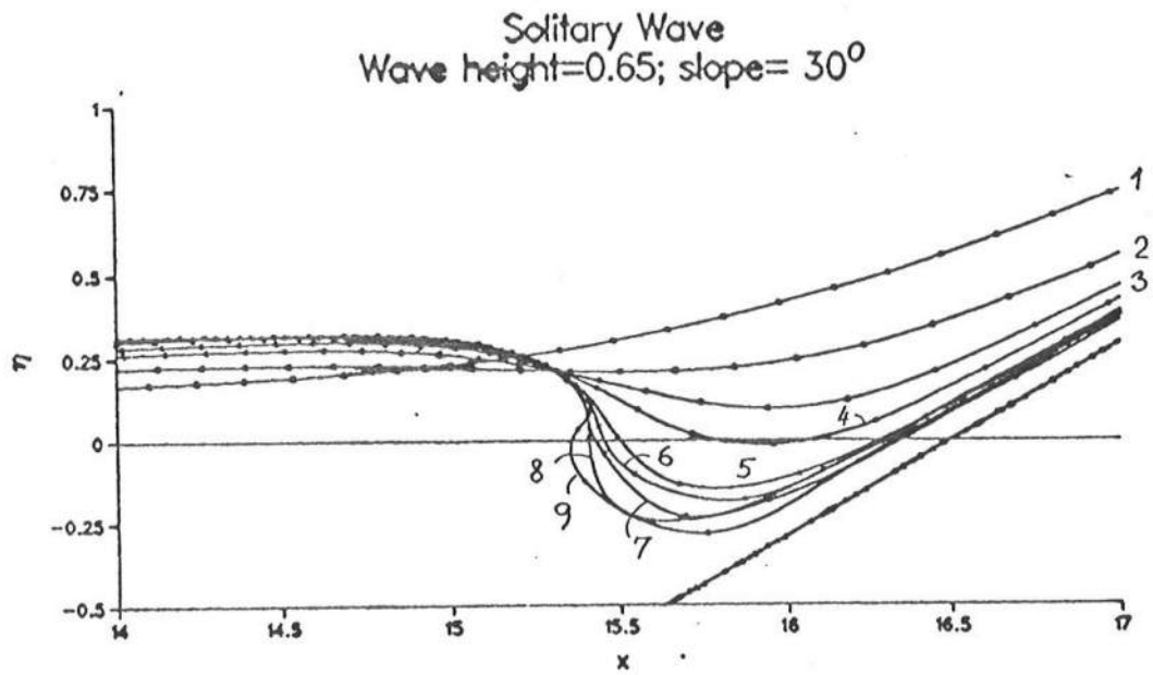
Figure 9: Breaking During Run Down.
