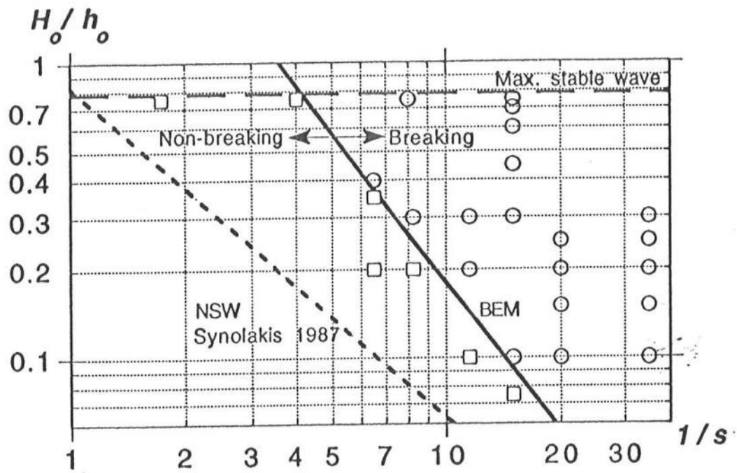
Figure 7: Wave Breaking Criterion
