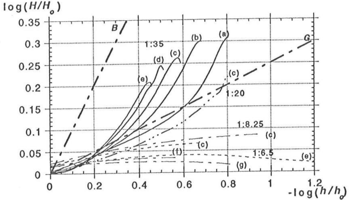
Figure 4: Shoaling of Solitary Waves of Different H_0/h_0 on Different Slopes.
