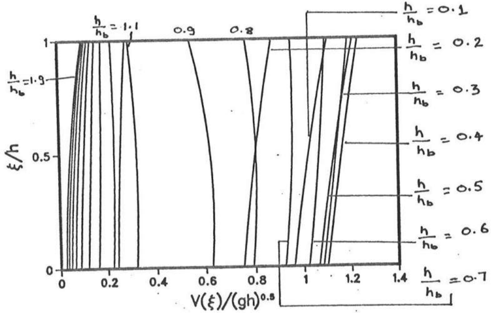
Figure 4: Computed vertical variation of the longshore current
