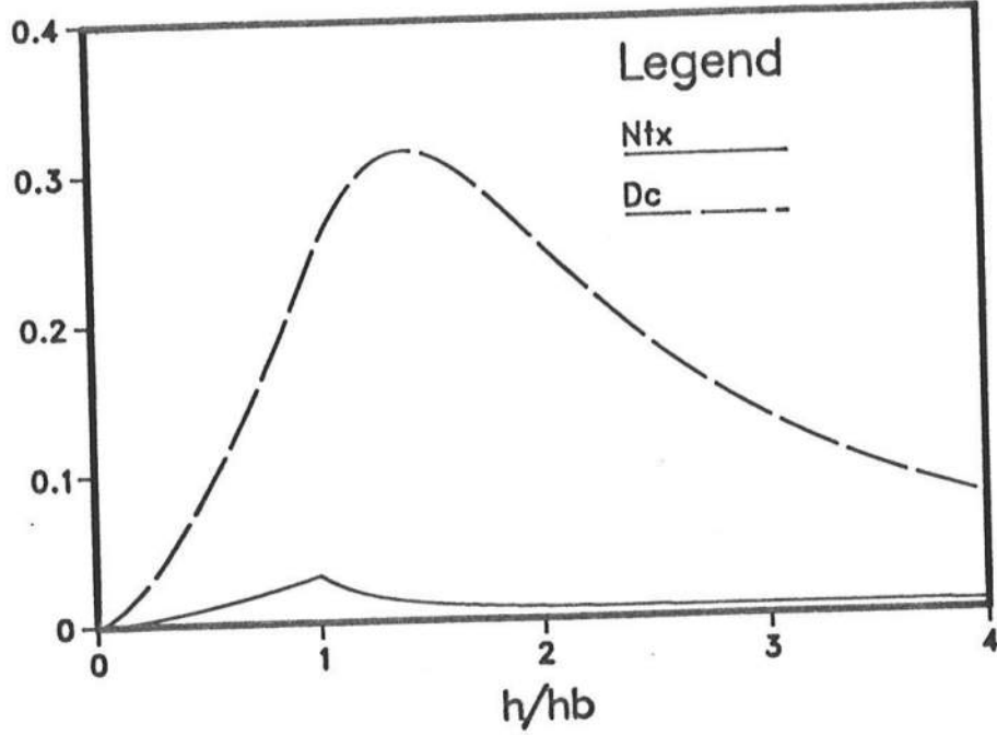
Figure 2: Variation of \nu_{tx} and D_c
