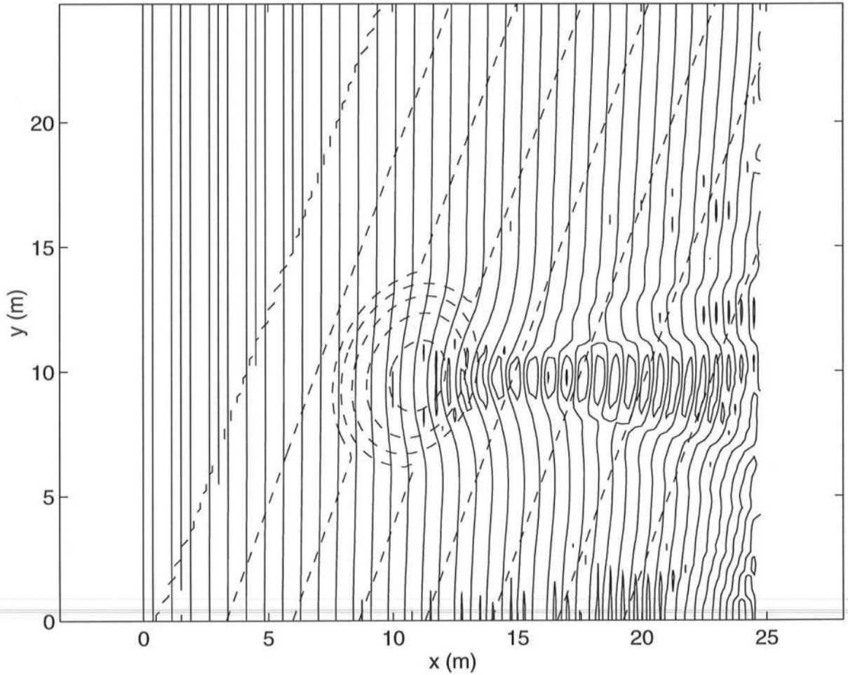
Figure 16: Results for waves propagating over a submerged shoal: surface elevation contours.
