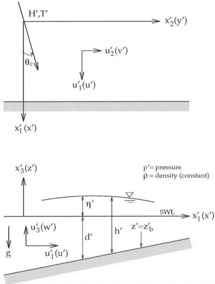
Figure 2.1: Definition sketch for obliquely incident wave motion on an impermeable slope.
