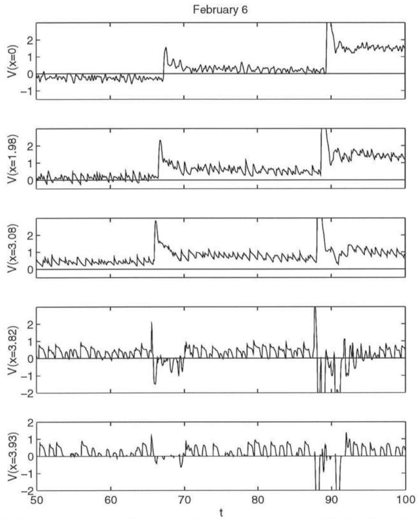
Figure 4.23: Computed temporal variations with sudden jumps of depth-averaged alongshore velocity V at x = 0, 1.98, 3.08, 3.82 and 3.93 for February 6 with \Delta t \simeq 0.0007 plotted from t = 50 to t = 100 .
