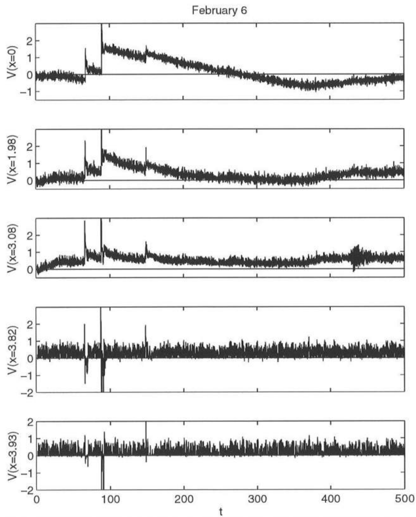
Figure 4.22: Computed temporal variations with sudden jumps of depth-averaged alongshore velocity V at x = 0, 1.98, 3.08, 3.82 and 3.93 for February 6 with \Delta t \simeq 0.0007 .
