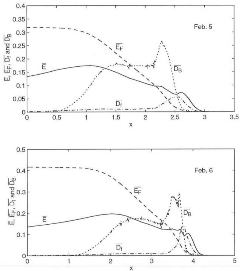
Figure 4.40: Computed cross-shore variations of specific energy \bar{E} , energy flux \bar{E}_F , dissipation rate \bar{D}_f , and \bar{D}_B due to bottom friction and wave breaking, respectively, for February 5 and February 6.
