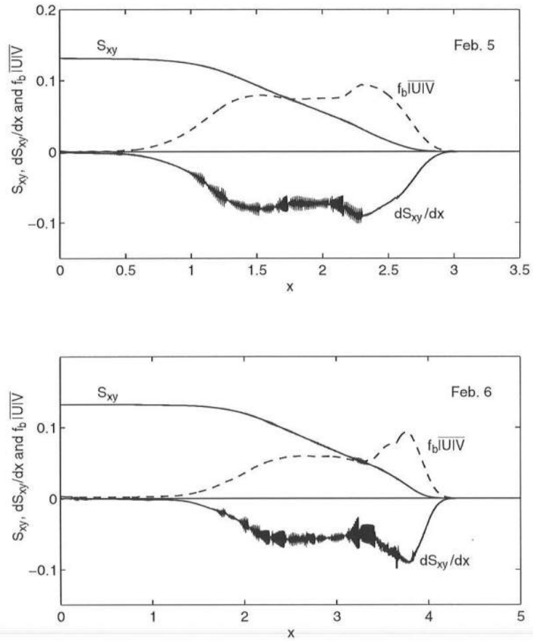
Figure 4.35: Computed cross-shore variations of alongshore radiation stress S_{xy} , its gradient and time-averaged alongshore bottom shear stress for February 5 and 6.
