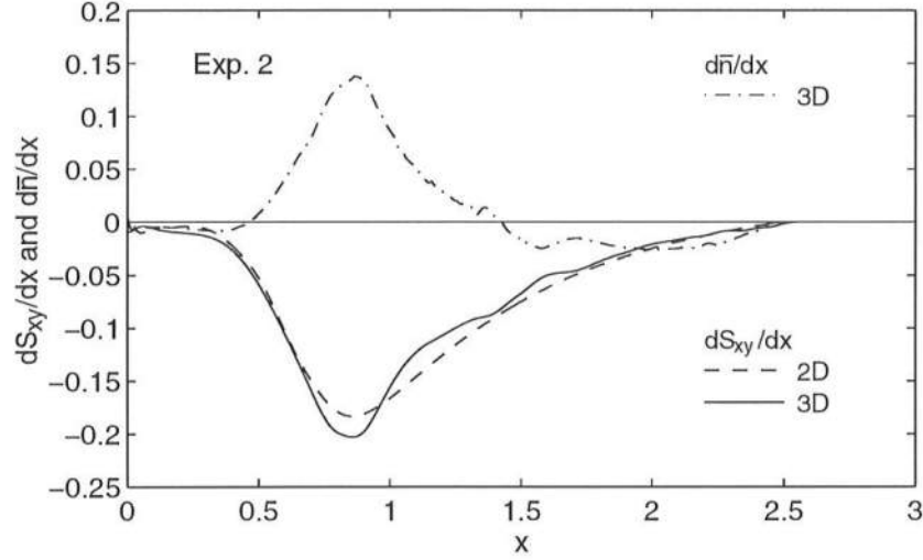
Figure 5.5: Computed cross-shore gradients of S_{xy} and \bar{n} for experiment 2.
