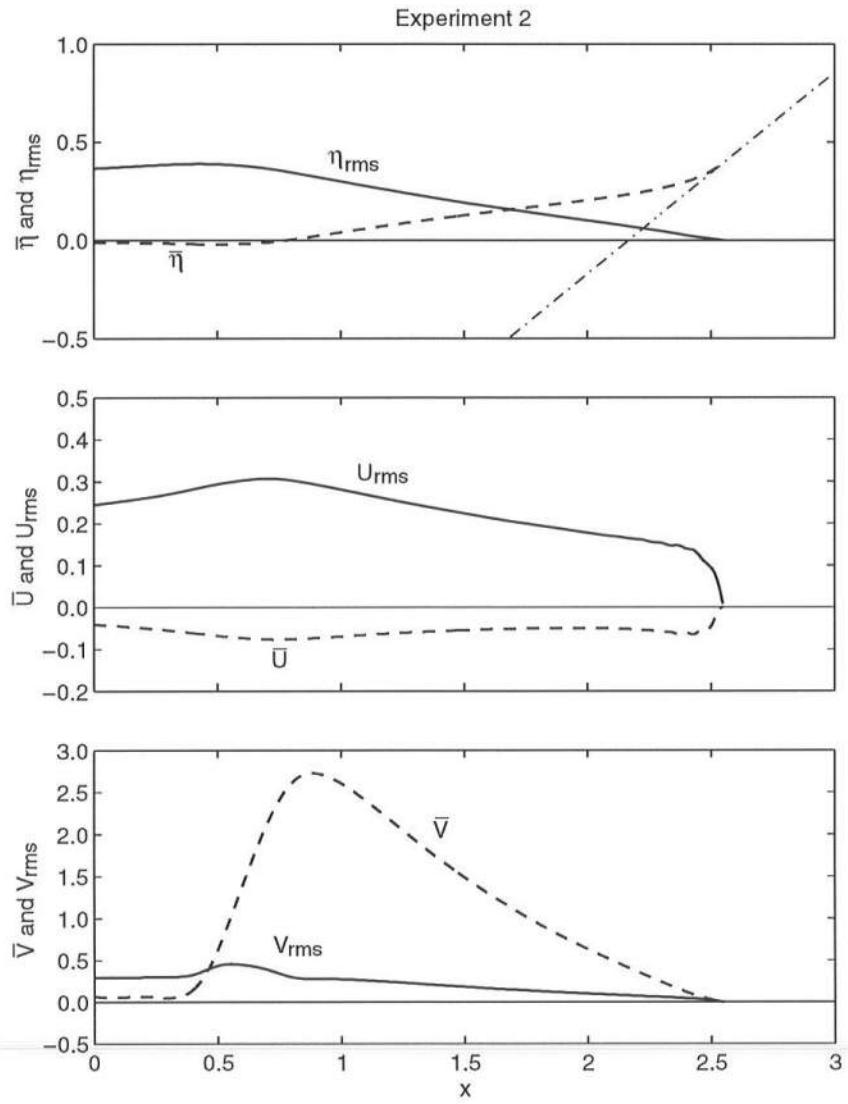
Figure 4.5: Cross-shore variations of \bar{\eta} , \eta_{rms} , \bar{U} , U_{rms} , \bar{V} , and V_{rms} .
