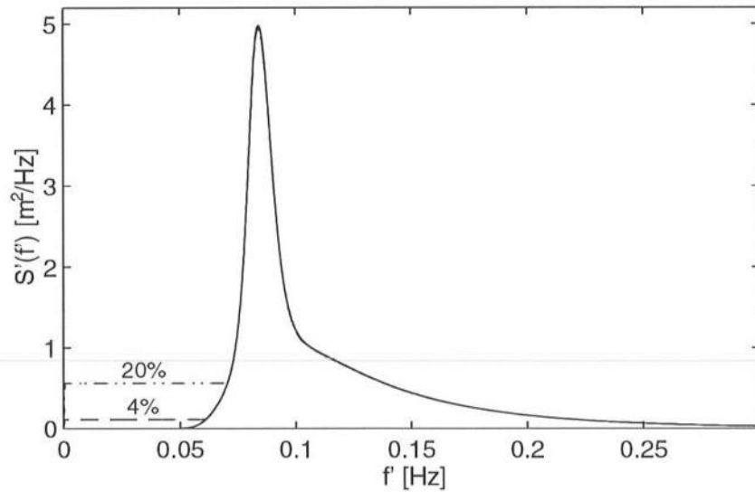
Figure 6.5: Incident wave frequency spectrum at the seaward boundary including the 4% and 20% low-frequency components.
