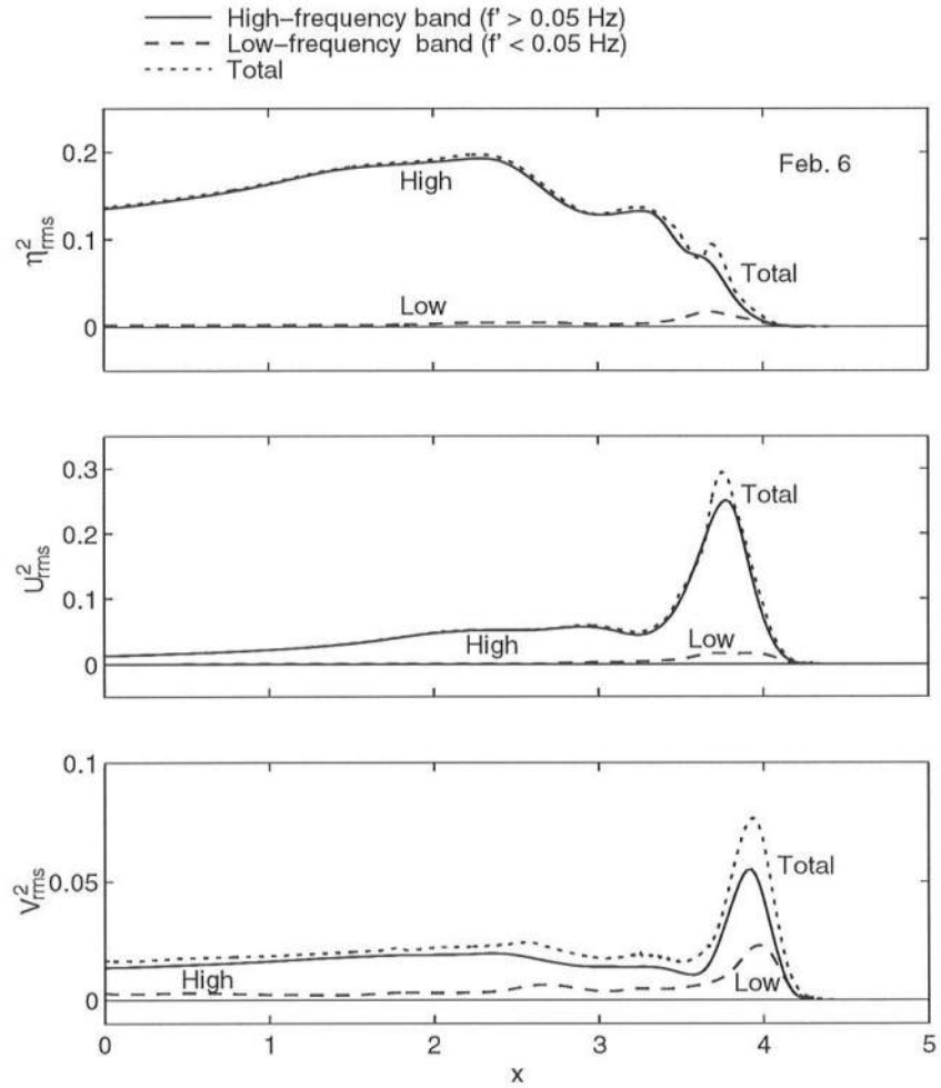
Figure 4.42: Computed cross-shore variations of variances of free surface elevation \eta , cross-shore velocity U and alongshore velocity V in high ( f' > 0.05\text{Hz} ) and low ( f' < 0.05\text{Hz} ) frequency bands for February 6.
