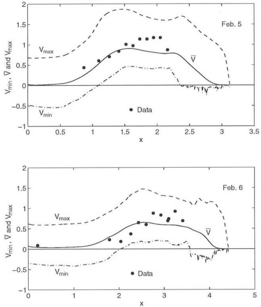
Figure 4.34: Comparisons between measured and computed longshore current \bar{V} together with computed maximum and minimum alongshore velocities, V_{max} and V_{min} , on February 5 and 6.
