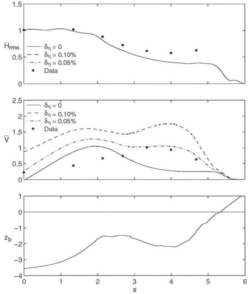
Figure 6.7: Effects of alongshore decrease of incident wave intensity on cross-shore variations of root-mean-square wave height H_{rms} and longshore current \bar{V} for barred beach.
