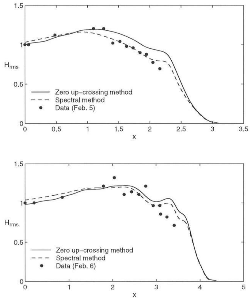
Figure 4.33: Comparisons between measured and computed root-mean-square wave height H_{rms} on February 5 and 6.
