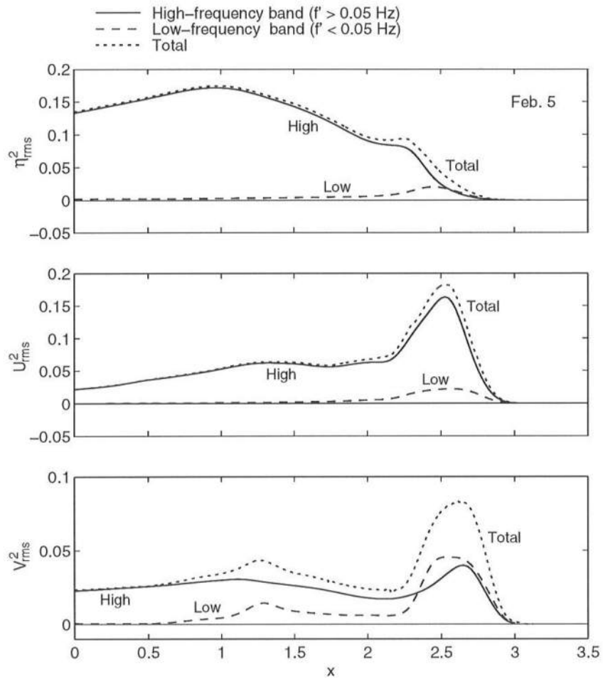
Figure 4.41: Computed cross-shore variations of variances of free surface elevation \eta , cross-shore velocity U and alongshore velocity V in high ( f' > 0.05 Hz ) and low ( f' < 0.05 Hz ) frequency bands for February 5.
