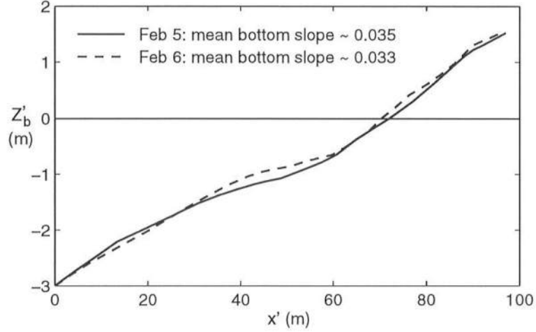
Figure 4.11: Measured bottom profiles for February 5 and 6.
