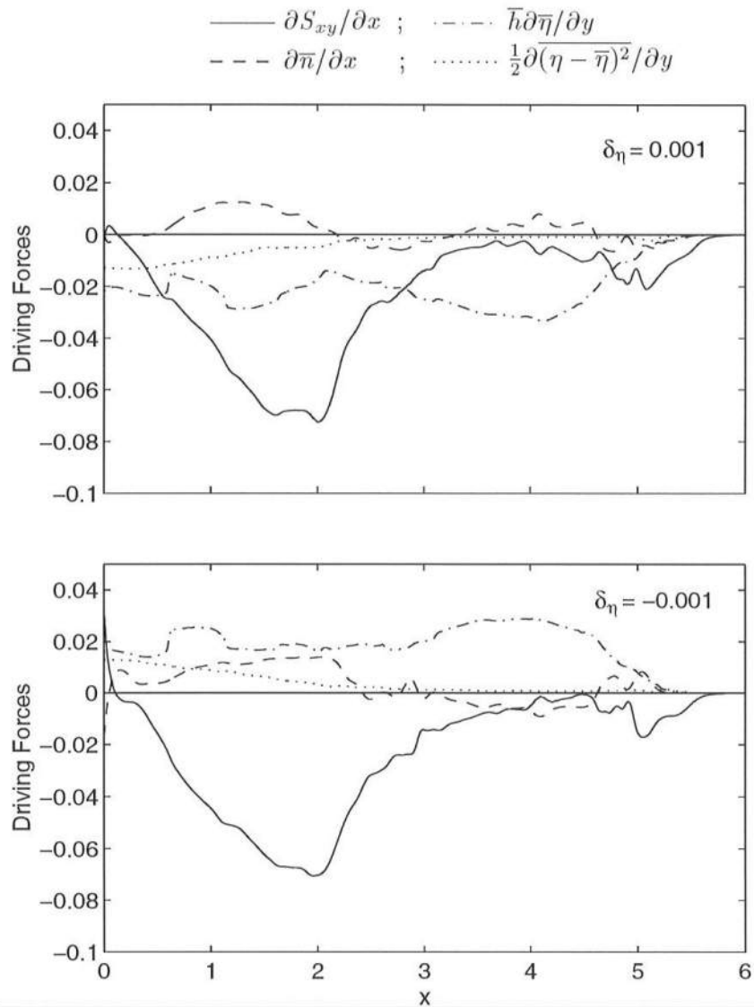
Figure 6.9: Computed cross-shore variations of driving forces in time-averaged alongshore momentum equation (6.1) for \delta_\eta = 0.001 with \partial \bar{\eta} / \partial y < 0 (wave setup decreasing in down-wave direction) and for \delta_\eta = -0.001 with \partial \bar{\eta} / \partial y > 0 .
