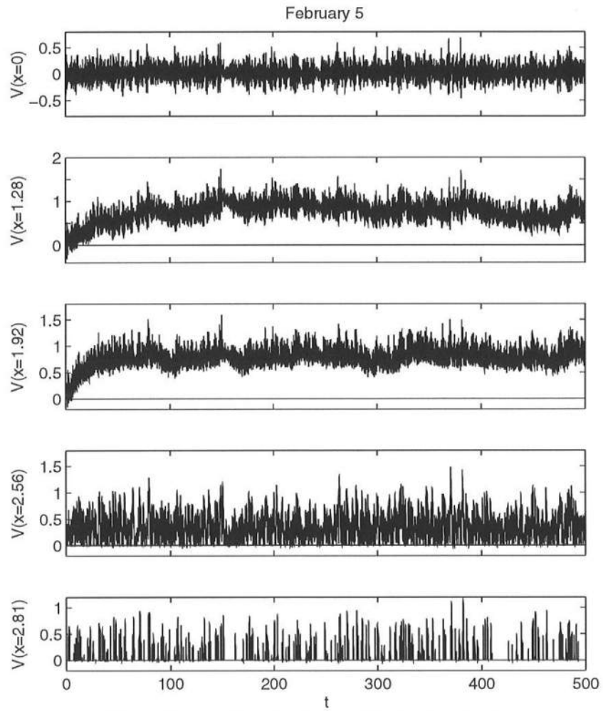
Figure 4.16: Computed temporal variations of depth-averaged alongshore velocity V at x = 0, 1.28, 1.92, 2.56 and 2.81 for February 5.
