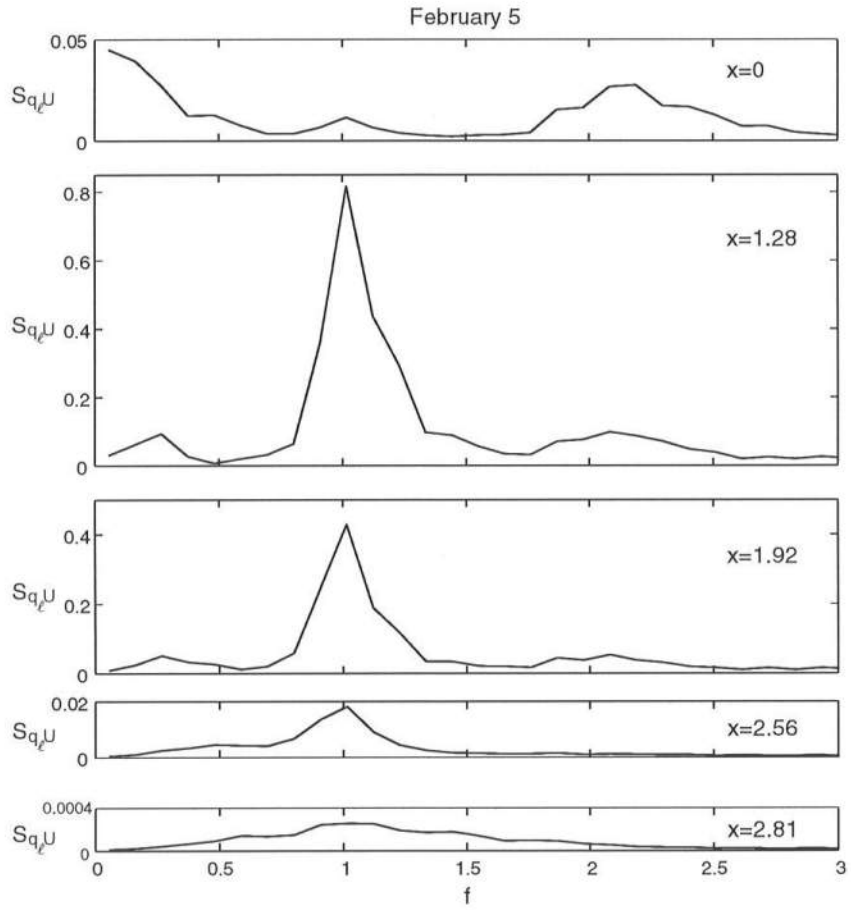
Figure 4.30: Computed frequency spectra of alongshore momentum flux, hUV = q_\ell U , at x = 0, 1.28, 1.92, 2.56, and 2.81 on February 5.
