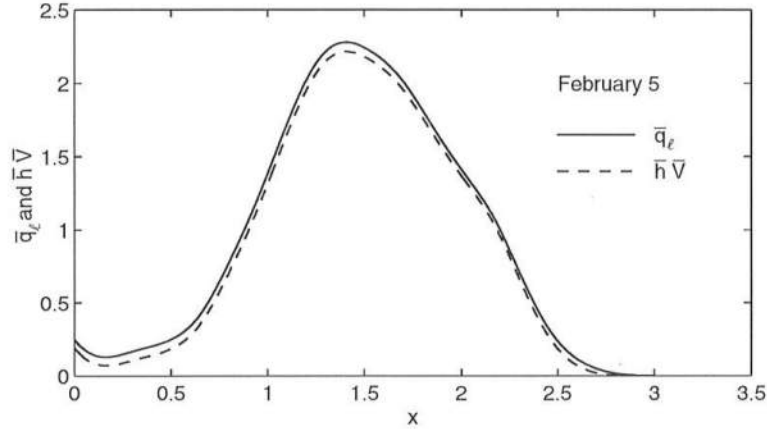
Figure 4.36: Computed cross-shore variations of mean alongshore volume flux \bar{q}_l = \bar{h}\bar{V} and product of mean depth \bar{h} and longshore current \bar{V} on February 5.
