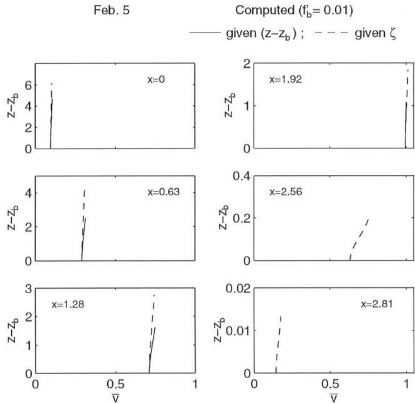
Figure 5.15: Measured and computed vertical variations of longshore current \bar{v} on February 5 for 3D model.
