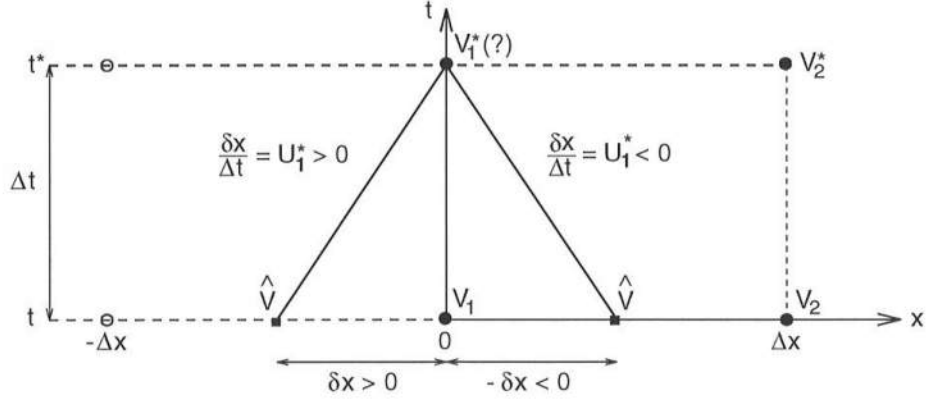
Figure 3.2: Sketch of seaward boundary algorithm for alongshore velocity V .
