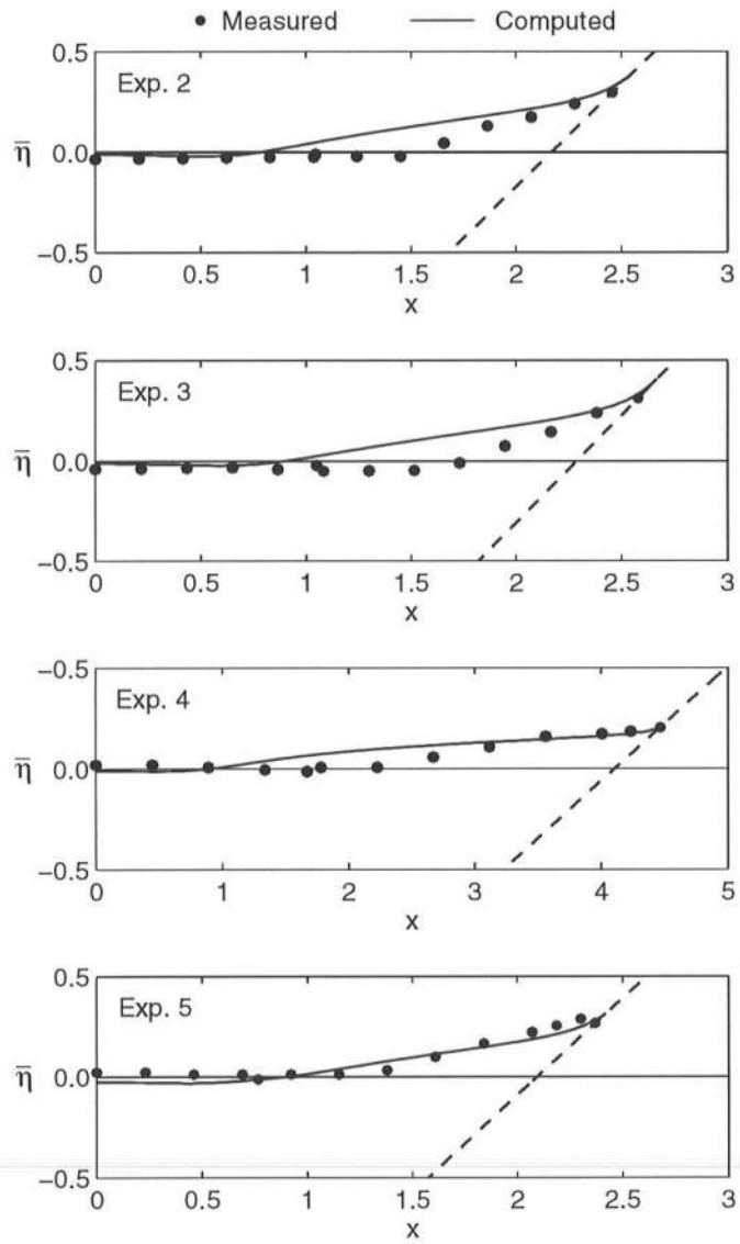
Figure 4.8: Measured and computed wave setup \bar{\eta} for four experiments.
