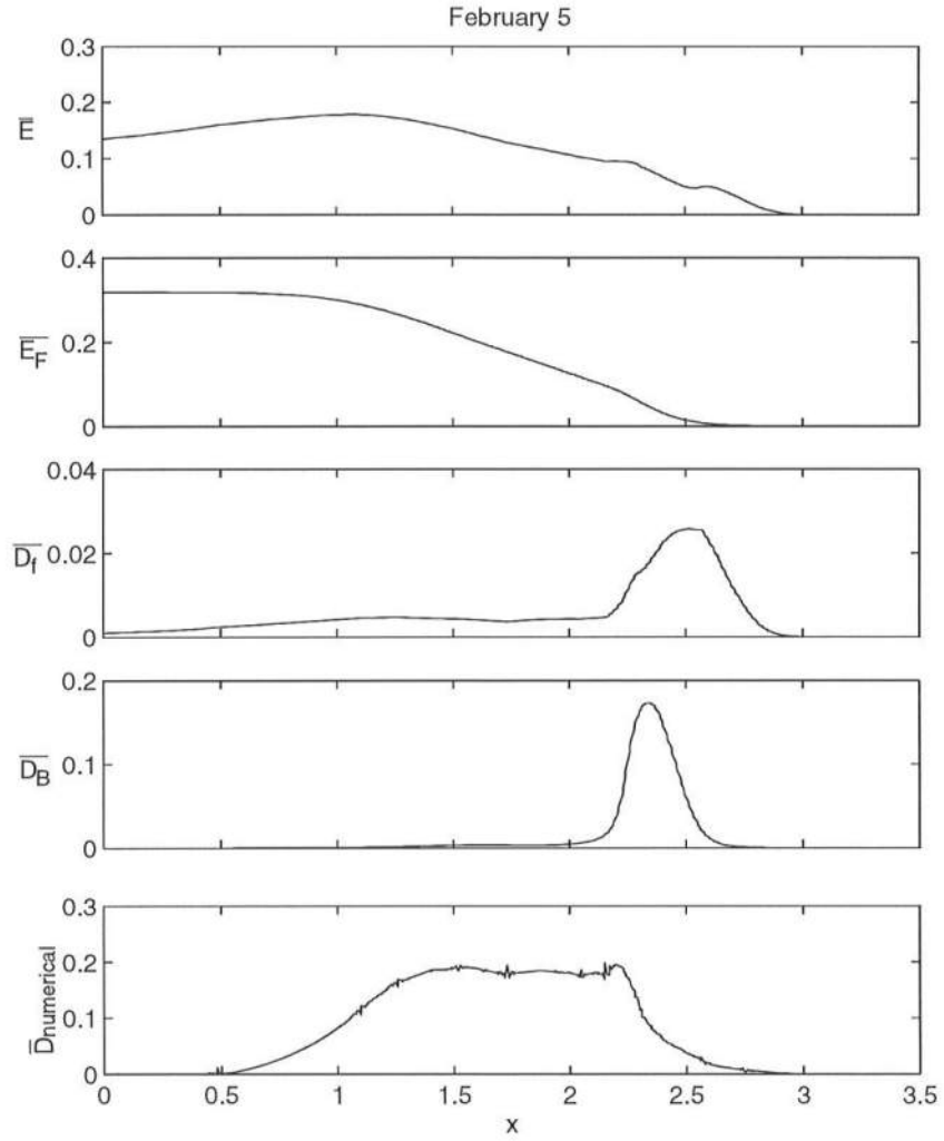
Figure 5.17: Computed cross-shore variations of time-averaged specific energy \overline{E} , energy flux \overline{E}_F , bottom frictional dissipation rate \overline{D}_f , wave breaking dissipation rate \overline{D}_B predicted physically by 3D model, and numerical dissipation rate \overline{D}_{\text{numerical}} estimated using time-averaged energy equation for February 5.
