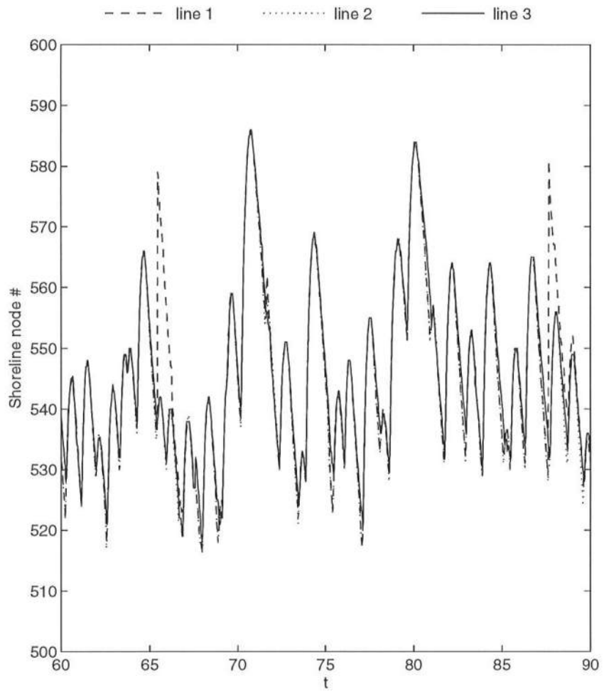
Figure 4.24: Shoreline oscillations at three cross-shore lines for February 6 with \Delta t \approx 0.0007 .
