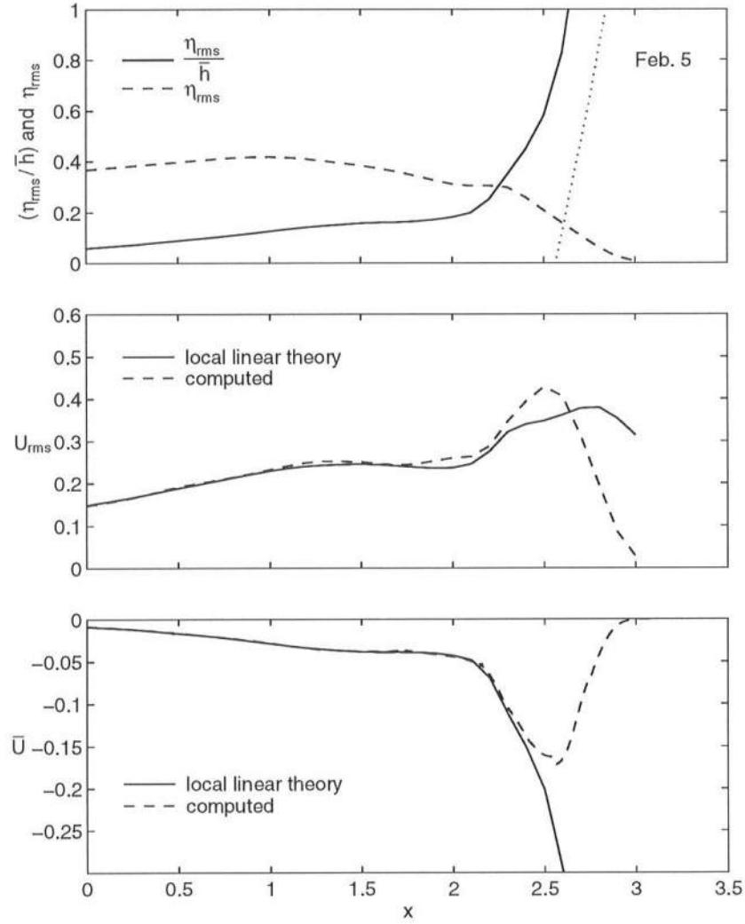
Figure 4.43: Cross-shore variations of \eta_{rms} , \eta_{rms}/\bar{h} , U_{rms} and \bar{U} computed using the 2D model as well as cross-shore variations of U_{rms} and \bar{U} computed using (4.10) and (4.11) together with the normalized bottom elevation for February 5.
