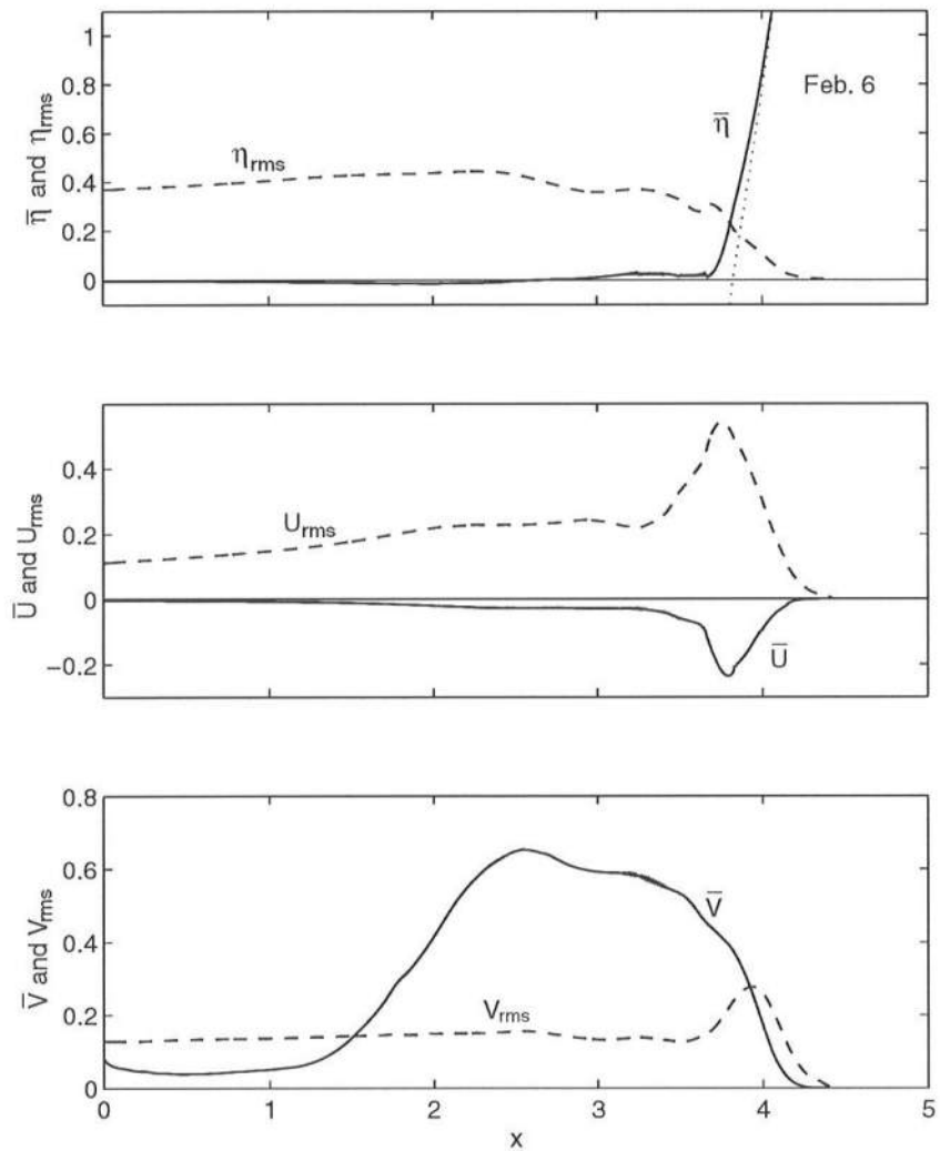
Figure 4.38: Computed cross-shore variations of mean and standard deviation of free surface elevation \eta , cross-shore velocity U and alongshore velocity V for February 6.
