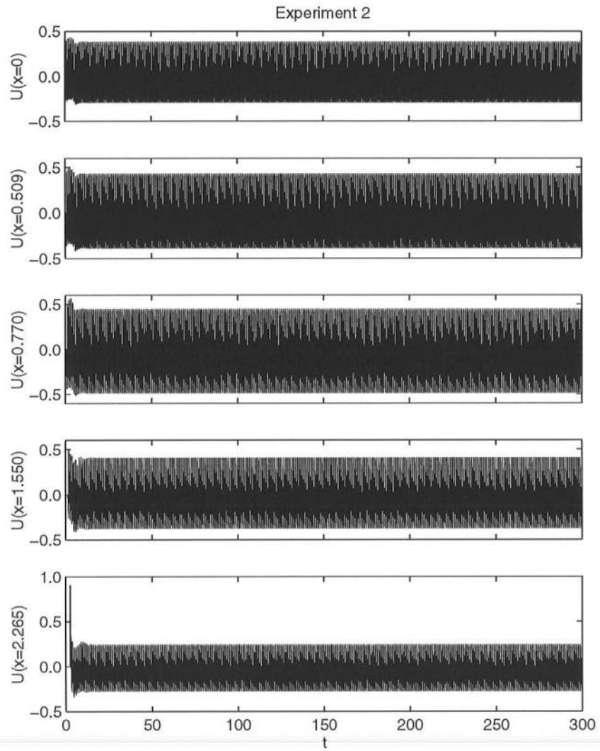
Figure 4.3: Computed temporal variations of depth-averaged cross-shore velocity U at x = 0, 0.509, 0.770, 1.550 and 2.265 .
