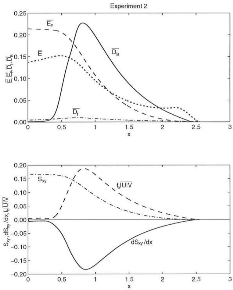
Figure 4.6: Time-averaged cross-shore wave energy and alongshore momentum balances.
