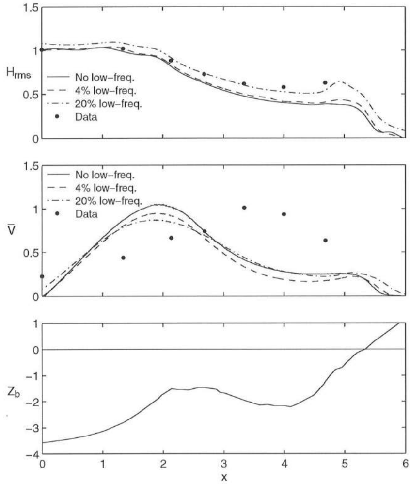
Figure 6.6: Effects of low-frequency wave components on the cross-shore variations of the root-mean-square wave height H_{rms} and longshore current \bar{V} for barred beach.
