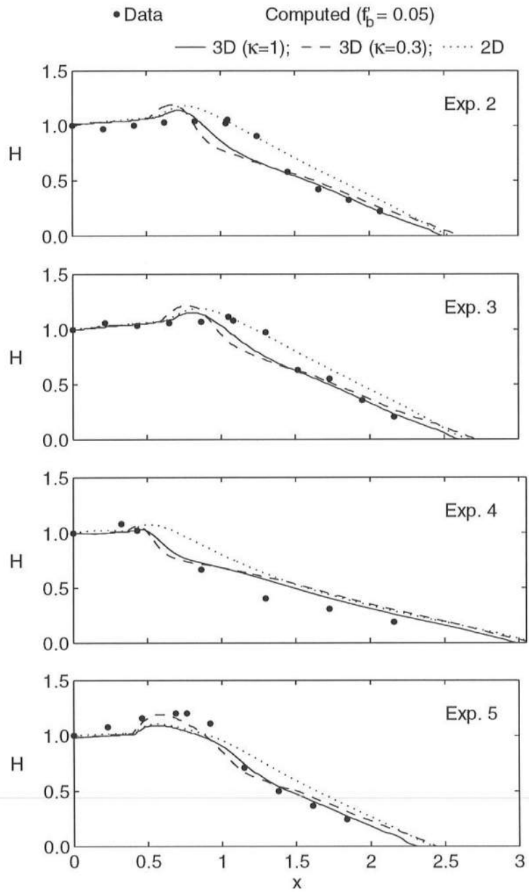
Figure 5.9: Measured and computed wave height H for four experiments using different values of \kappa for 3D model.
