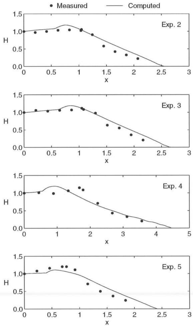
Figure 4.7: Measured and computed local wave height H for four experiments.
