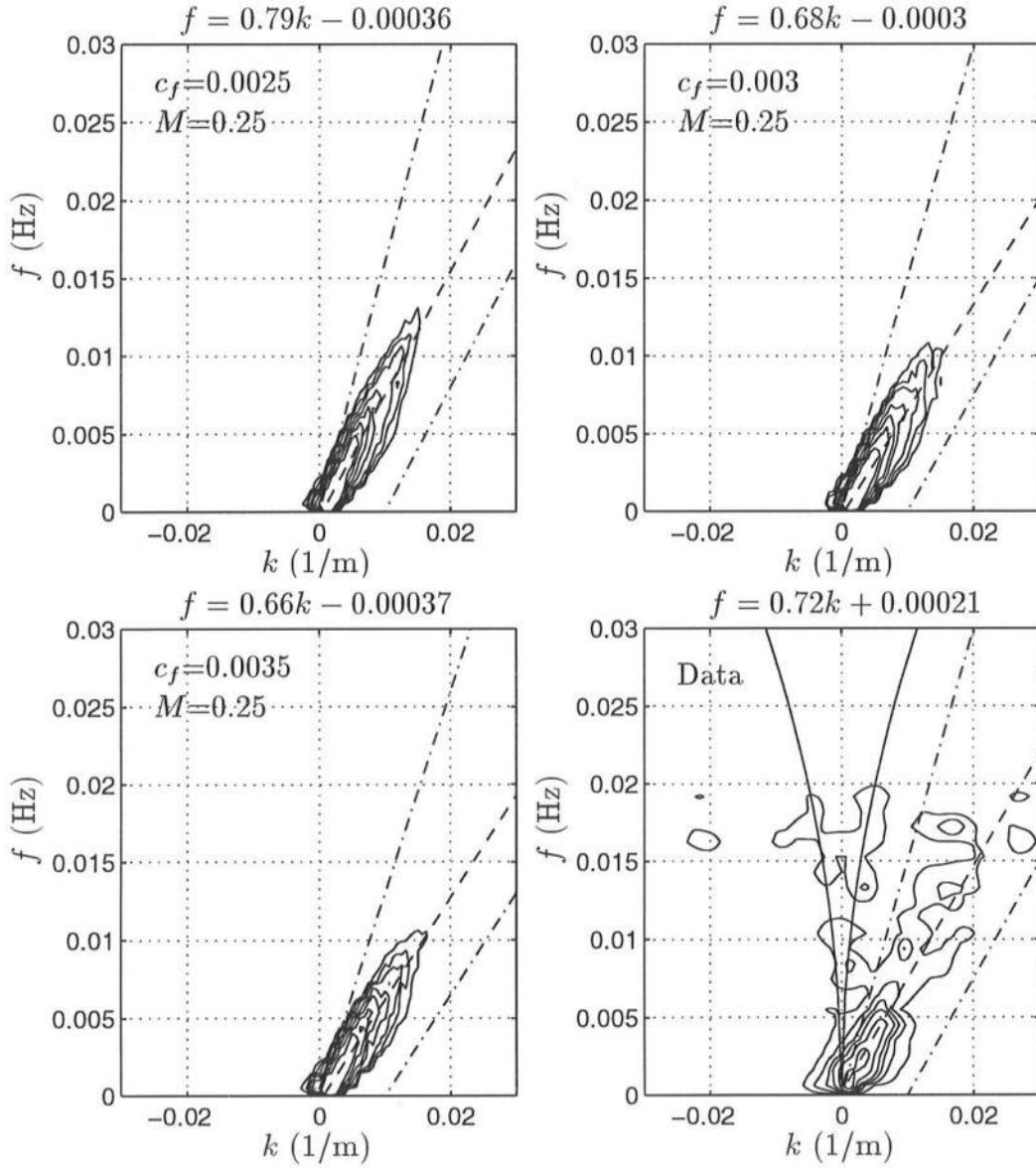
Figure 6.47: October 18: Frequency-cyclic wavenumber spectra S(f, k) ( \text{m}^3/\text{s} ) for computed and measured longshore velocity at x = 35 m. The values for c_{est} are 0.8 m/s for c_f = 0.0025 , 0.75 for c_f = 0.003 , 0.65 m/s for c_f = 0.0035 , and 0.75 m/s for data, and are used in Equation (6.3) to construct the upper and lower cut-off lines (— · —) of the shear wave energy. Contour levels plotted are (10, 30, 60, 100, 200, 400, 800). The equation for the best fit dispersion line (—) is noted above each plot.
