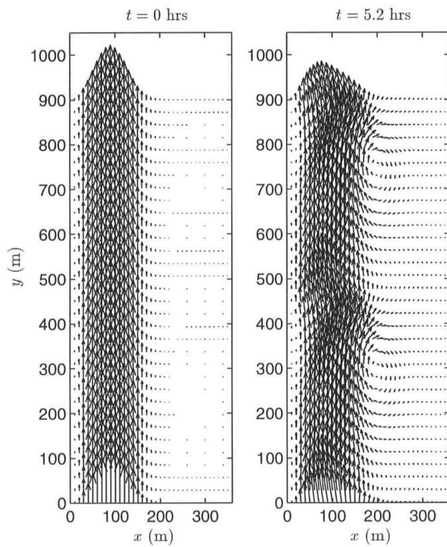
Figure 5.10: ND=2: Snapshots of vector plots of circulation
