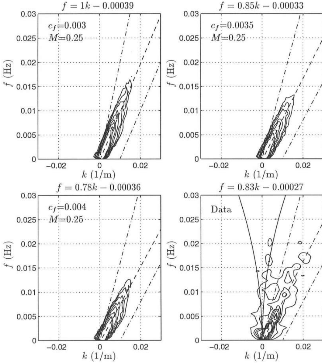
Figure 6.35: October 16: Frequency-cyclic wavenumber spectra S(f, k) ( \text{m}^3/\text{s} ) for computed and measured longshore velocity at x = 35 m. The values for c_{est} are 1 m/s for c_f = 0.003 , 0.8 m/s for c_f = 0.0035 and c_f = 0.004 , and 0.8 m/s for data, and are used in Equation (6.3) to construct the upper and lower cut-off lines (— · —) of the shear wave energy. Contour levels plotted are (10, 30, 60, 100, 200, 400, 800). The equation for the best fit dispersion line (— —) is noted above each plot.
