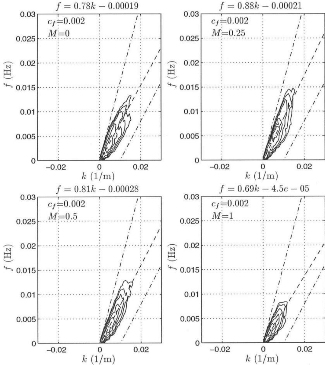
Figure 6.54: October 15: Frequency-cyclic wavenumber spectra S(f, k) ( \text{m}^3/\text{s} ) for computed cross-shore velocity at x=45 m. The value for c_{est} is 0.8 m/s, and is used in Equation (6.3) to construct the upper and lower cut-off lines ( - \cdot - ) of the shear wave energy. Contour levels plotted are (10, 30, 60, 100, 200, 400, 800). The equation for the best fit dispersion line ( - - ) is noted above each plot.
