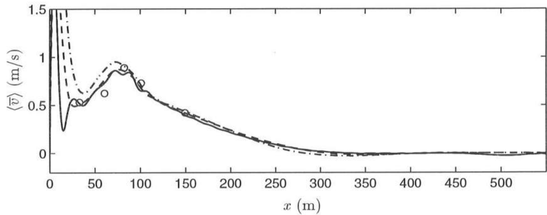
Figure 6.83: October 18: Time and longshore-averaged longshore currents \langle \bar{v} \rangle for c_f = 0.003 and M = 0 (—), M = 0.25 (— —), M = 0.5 (— · —) and sled data ( \circ ).
