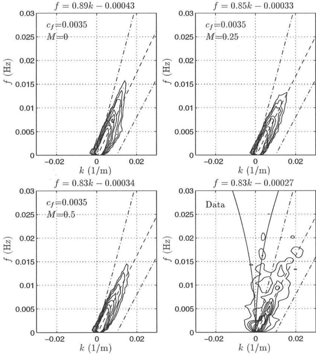
Figure 6.69: October 16: Frequency-cyclic wavenumber spectra S(f, k) ( \text{m}^3/\text{s} ) for computed and measured longshore velocity at x = 35 m. The value for c_{est} is 0.8 m/s, and is used in Equation (6.3) to construct the upper and lower cut-off lines ( - \cdot - ) of the shear wave energy. Contour levels plotted are (10, 30, 60, 100, 200, 400, 800). The equation for the best fit dispersion line ( - - ) is noted above each plot.
