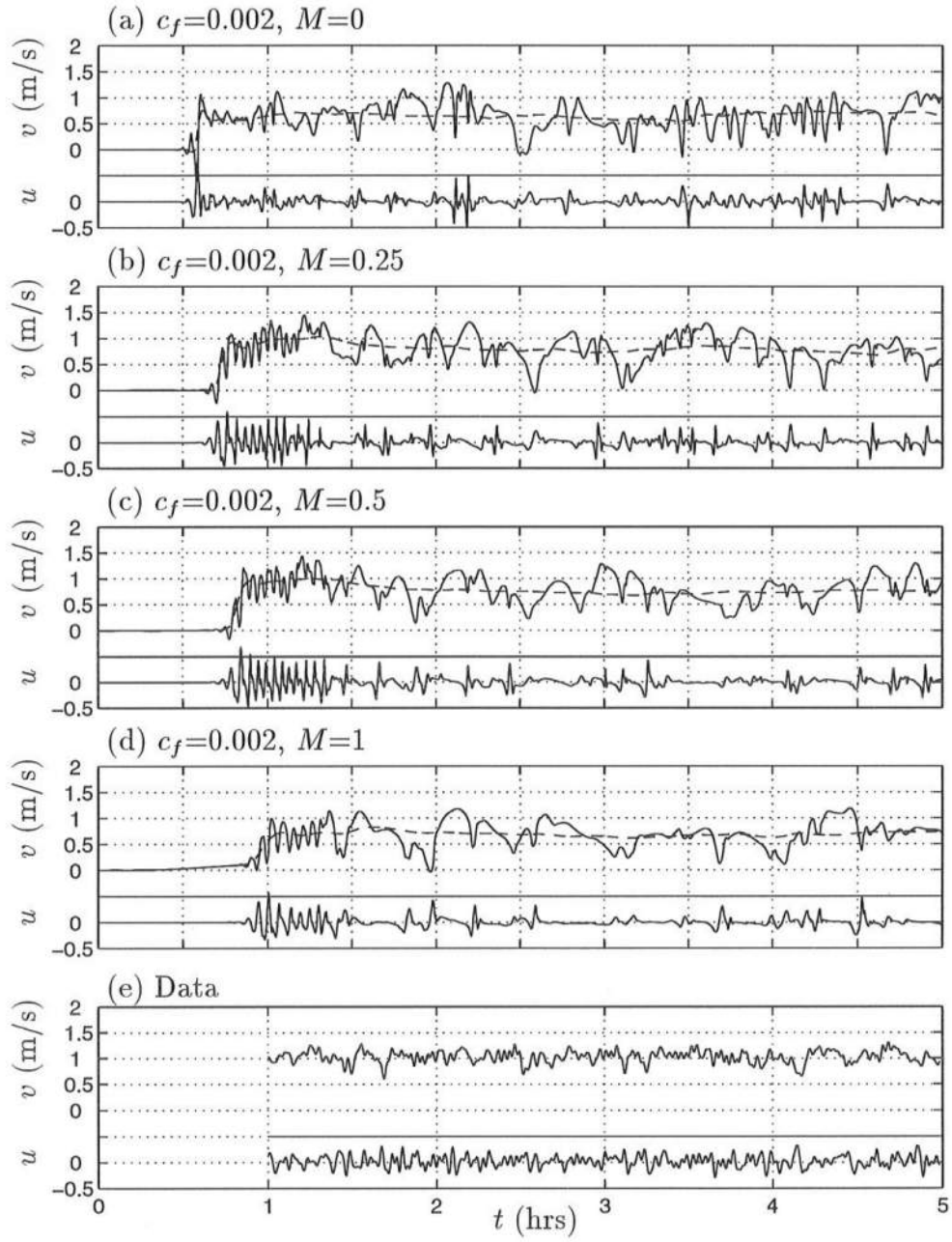
Figure 6.52: October 15: Time series of velocities u , v and \langle v \rangle (— —) at (x, y) = (45 \text{ m}, L_y/2) and time series of velocities u and v of data.
