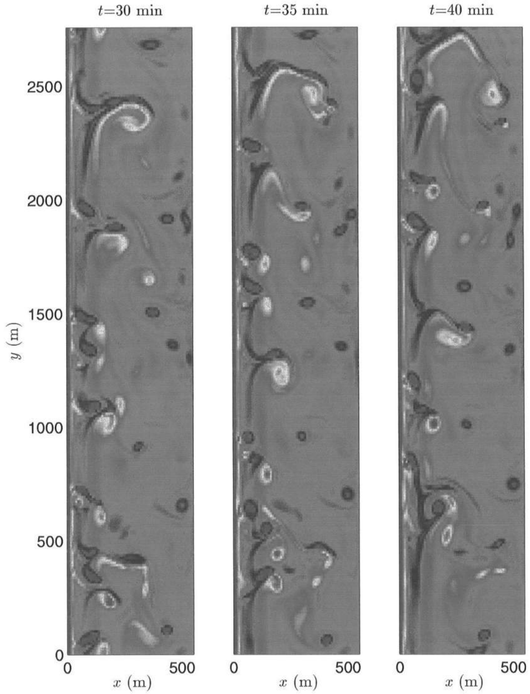
Figure 6.32: October 15: Time evolution of vorticity q (1/s) for c_f = 0.002 and M = 0.25 (continued).
