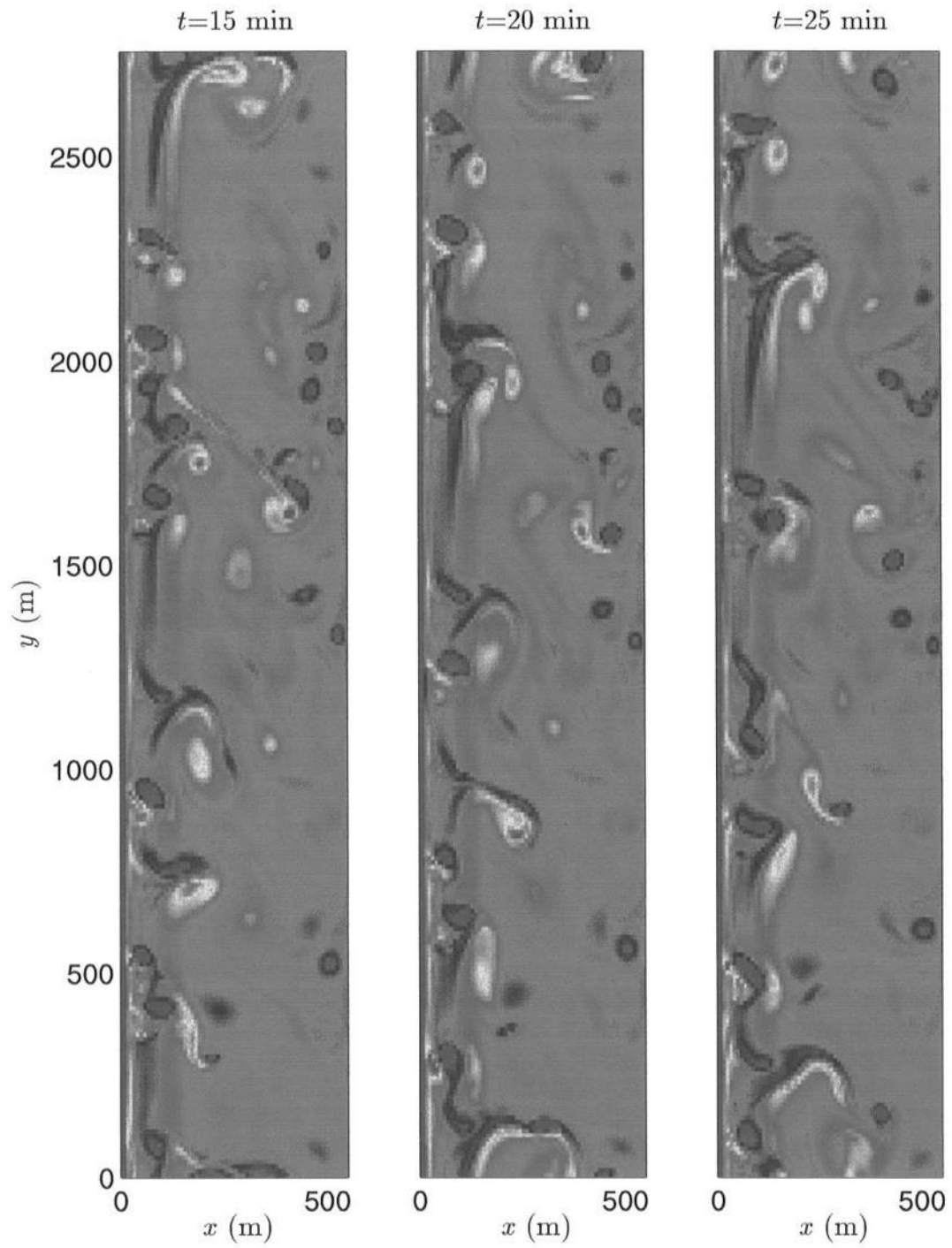
Figure 6.31: October 15: Time evolution of vorticity q (1/s) for c_f = 0.002 and M = 0.25 (continued).
