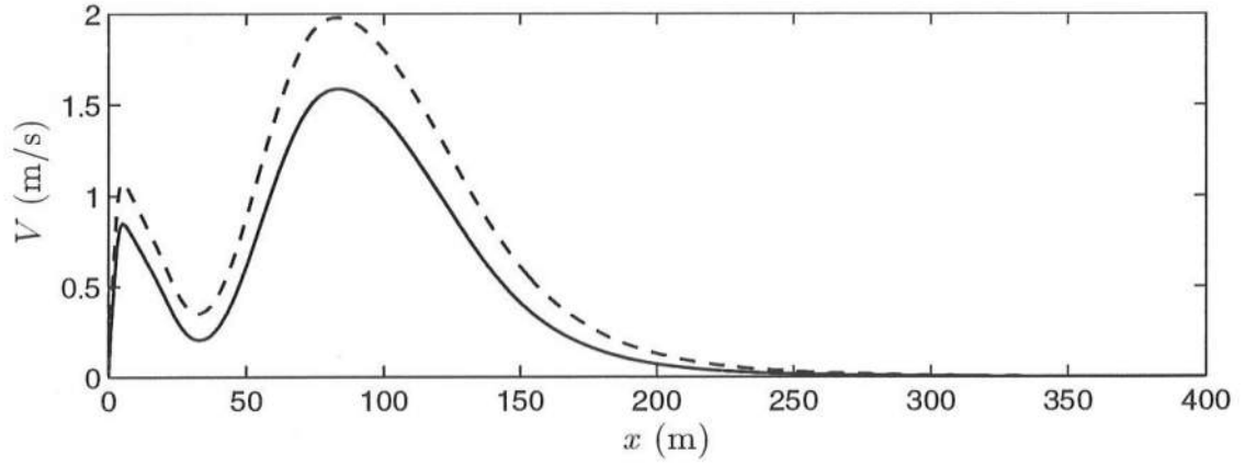
Figure 6.19: Longshore current for October 16 using M = 1 . Friction coefficient c_f = 0.004 (—) and c_f = 0.003 (---).
