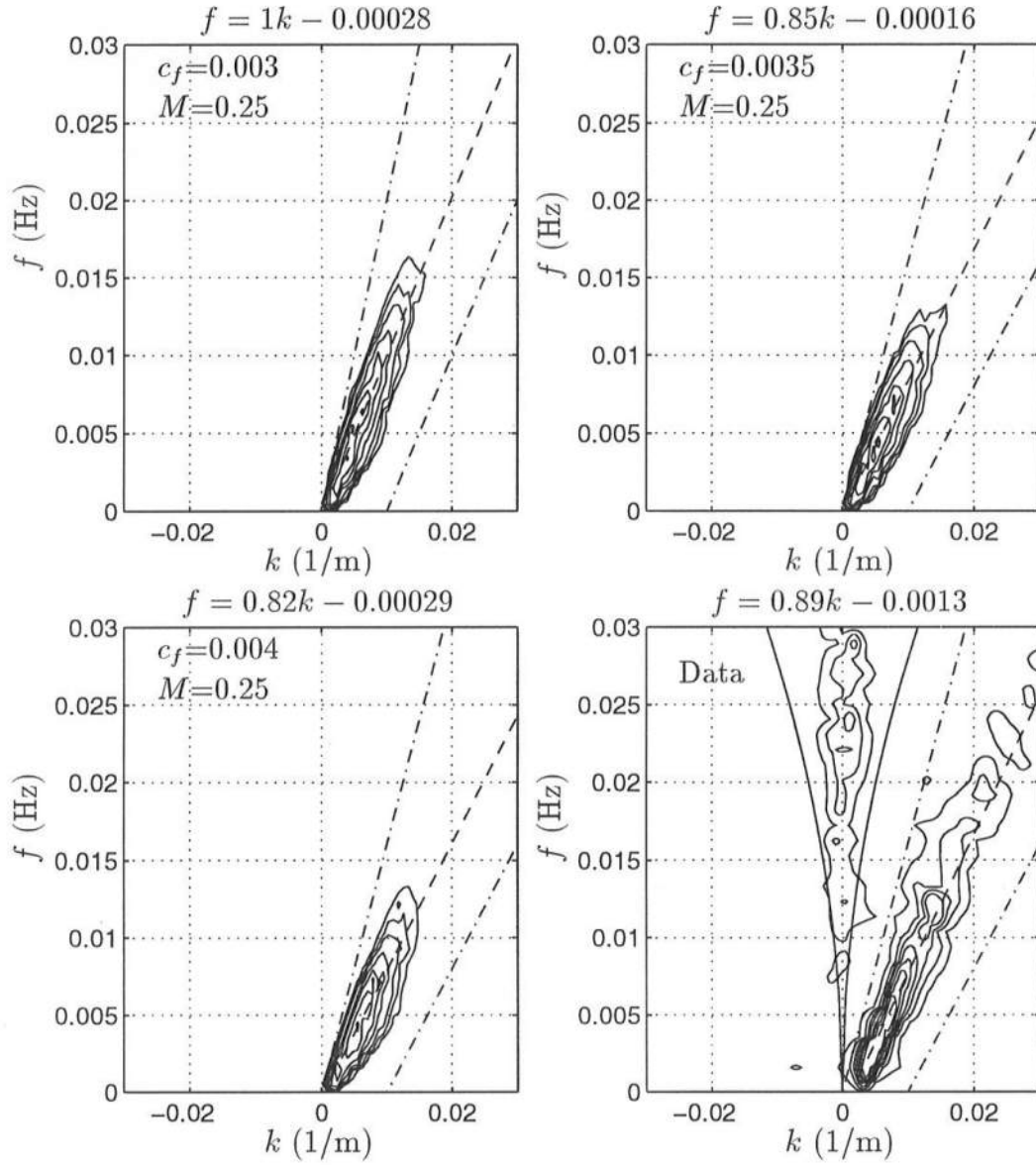
Figure 6.36: October 16: Frequency-cyclic wavenumber spectra S(f, k) ( \text{m}^3/\text{s} ) for computed and measured cross-shore velocity at x = 35 m. The values for c_{est} are 1 m/s for c_f = 0.003 , 0.8 m/s for c_f = 0.0035 and c_f = 0.004 , and 0.8 for data, and are used in Equation (6.3) to construct the upper and lower cut-off lines (— · —) of the shear wave energy. Contour levels plotted are (10 30 60 100 200 400 800). The equation for the best fit dispersion line (—) is noted above each plot.
