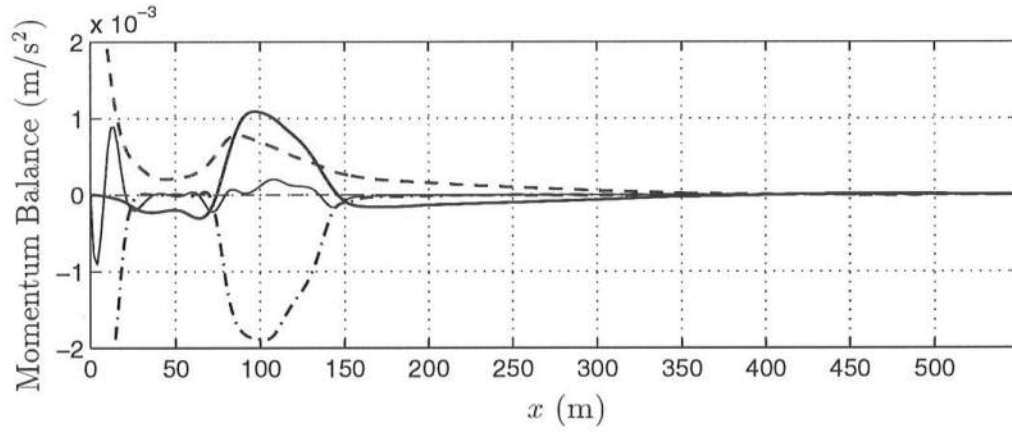
Figure 6.60: October 15: Mean longshore momentum balance for c_f = 0.002 , M = 0.5 . \langle u(\partial v / \partial x) \rangle (thick —), -\langle \tilde{\tau}_y \rangle (- · -), -\langle \tau'_y \rangle (thin —), \langle \frac{\mu}{D} v \rangle (thick - -), residual (thin - -).
