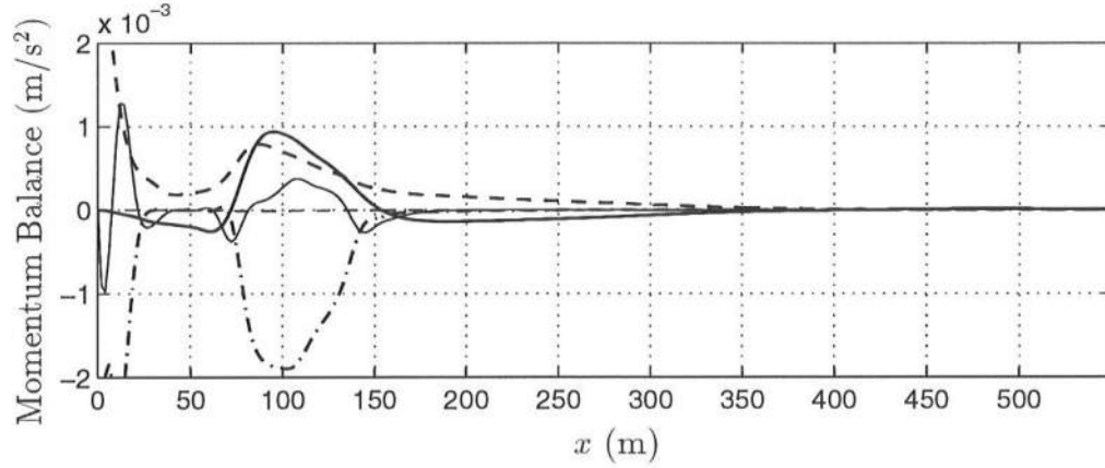
Figure 6.61: October 15: Mean longshore momentum balance for c_f = 0.002 , M = 1 . \langle u(\partial v / \partial x) \rangle (thick —), -\langle \tilde{\tau}_y \rangle (- · -), -\langle \tau_y' \rangle (thin —), \langle \frac{\mu}{D} v \rangle (thick - -), residual (thin - -).
