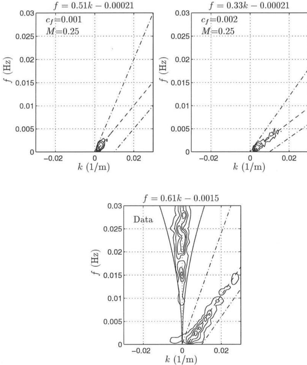
Figure 6.42: October 17: Frequency-cyclic wavenumber spectra S(f, k) (m 3 /s) for computed and measured cross-shore velocity at x = 35 m. The values for c_{est} are 0.5 m/s for c_f = 0.001 , 0.3 m/s for c_f = 0.002 , and 0.6 for data, and are used in Equation (6.3) to construct the upper and lower cut-off lines (— · —) of the shear wave energy. Contour levels plotted are (10 30 60 100 200 400 800). The equation for the best fit dispersion line (— —) is noted above each plot.
