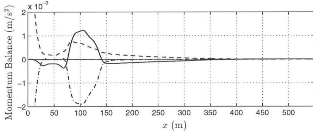
Figure 6.58: October 15: Mean longshore momentum balance for c_f = 0.002 , M = 0 . \langle u(\partial v / \partial x) \rangle (thick —), -\langle \tilde{\tau}_y \rangle (- · -), -\langle \tau_y' \rangle (thin —), \langle \frac{\mu}{D} v \rangle (thick - -), residual (thin - -).
