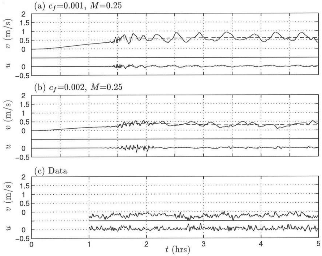
Figure 6.40: October 17: Time series of velocities u , v and \langle v \rangle (— —) at (x, y) = (35 \text{ m}, L_y/2) and time series of velocities u and v of data.
