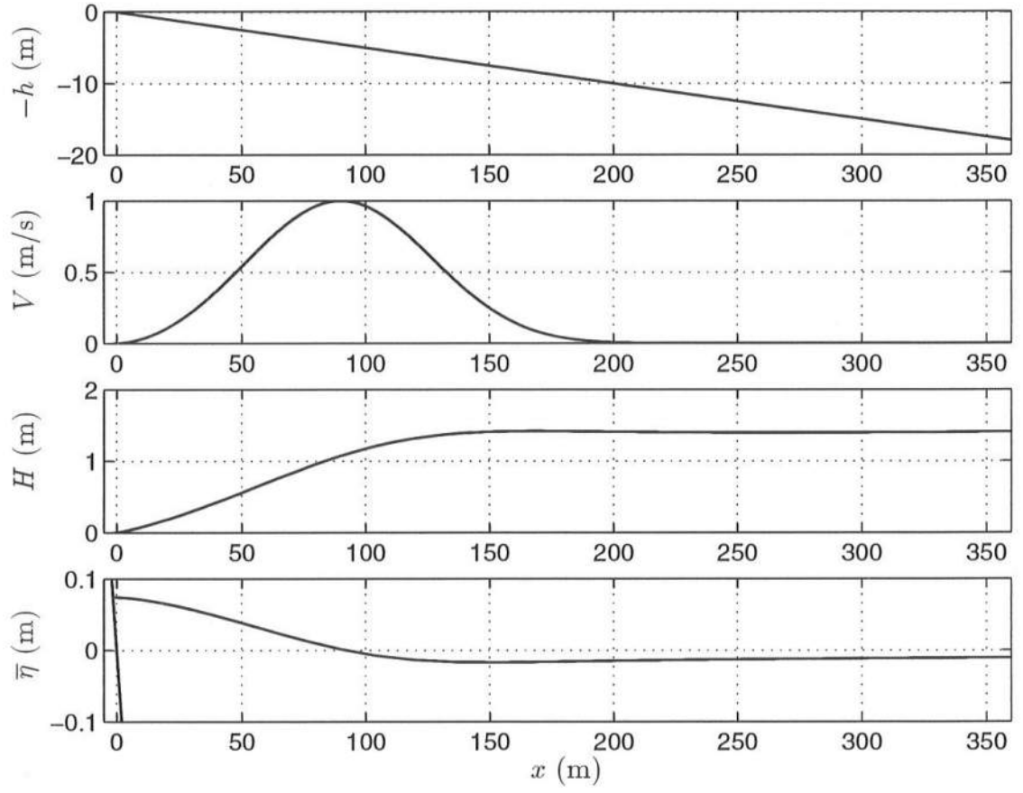
Figure 5.1: (a) Bathymetry for m = 0.05 , (b) longshore current profile, (c) wave height decay and (d) setup for f_p = 0.13 Hz and \theta_0 = 20^\circ .
