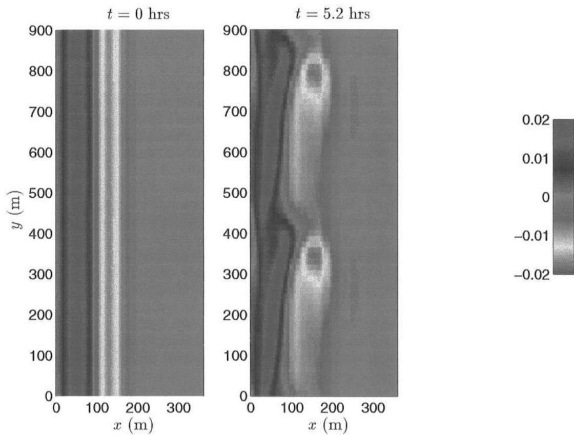
Figure 5.9: ND=2: Snapshots of contour plots of vorticity q (1/s)
