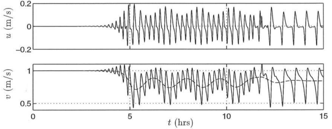
Figure 5.14: ND=2: Time series of u , v and \langle v \rangle (— —) at (x, y) = (90 \text{ m}, 0.5L_y) . Alternate initial condition used.
