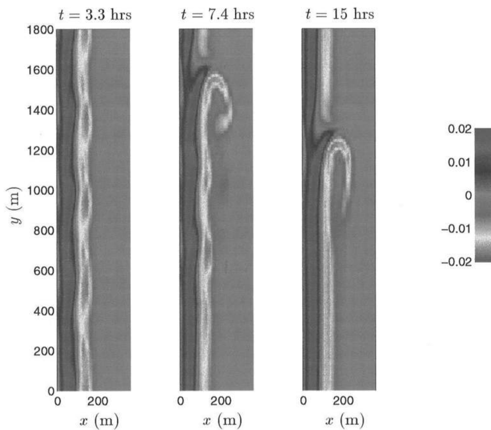
Figure 5.18: ND=4: Snapshots of contour plots of vorticity q ( 1/s )
