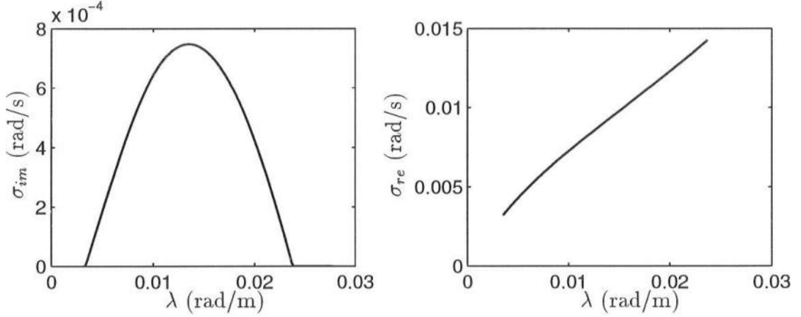
Figure 5.2: Linear instability results for the bottom and current profile shown in Figure 5.1.
