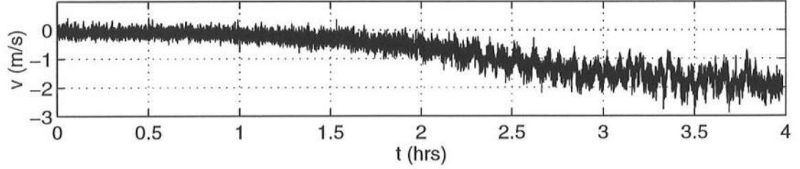
Figure 7.1: October 10: Time series of measured longshore current.
