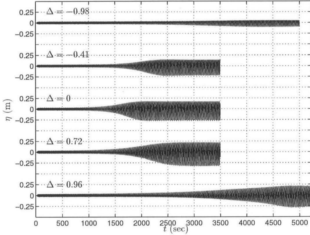
Figure 4.8: Water surface elevation \eta at (x, y) = (6, 0) m for various \Delta values
