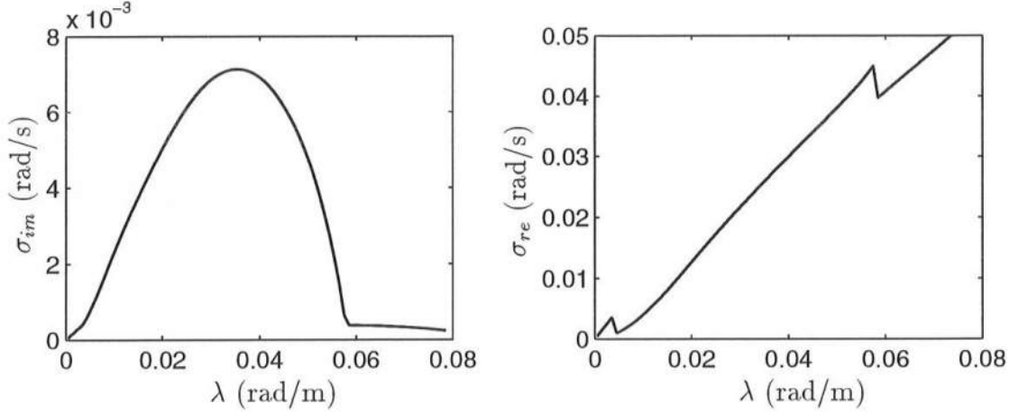
Figure 6.15: Linear instability results for October 15.
