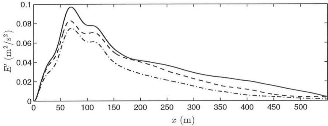
Figure 6.38: October 16: Time and longshore-averaged longshore perturbation kinetic energy \frac{1}{2}\langle u'^2 + v'^2 \rangle for c_f = 0.003 (—), c_f = 0.0035 (---), c_f = 0.004 (- · -).
