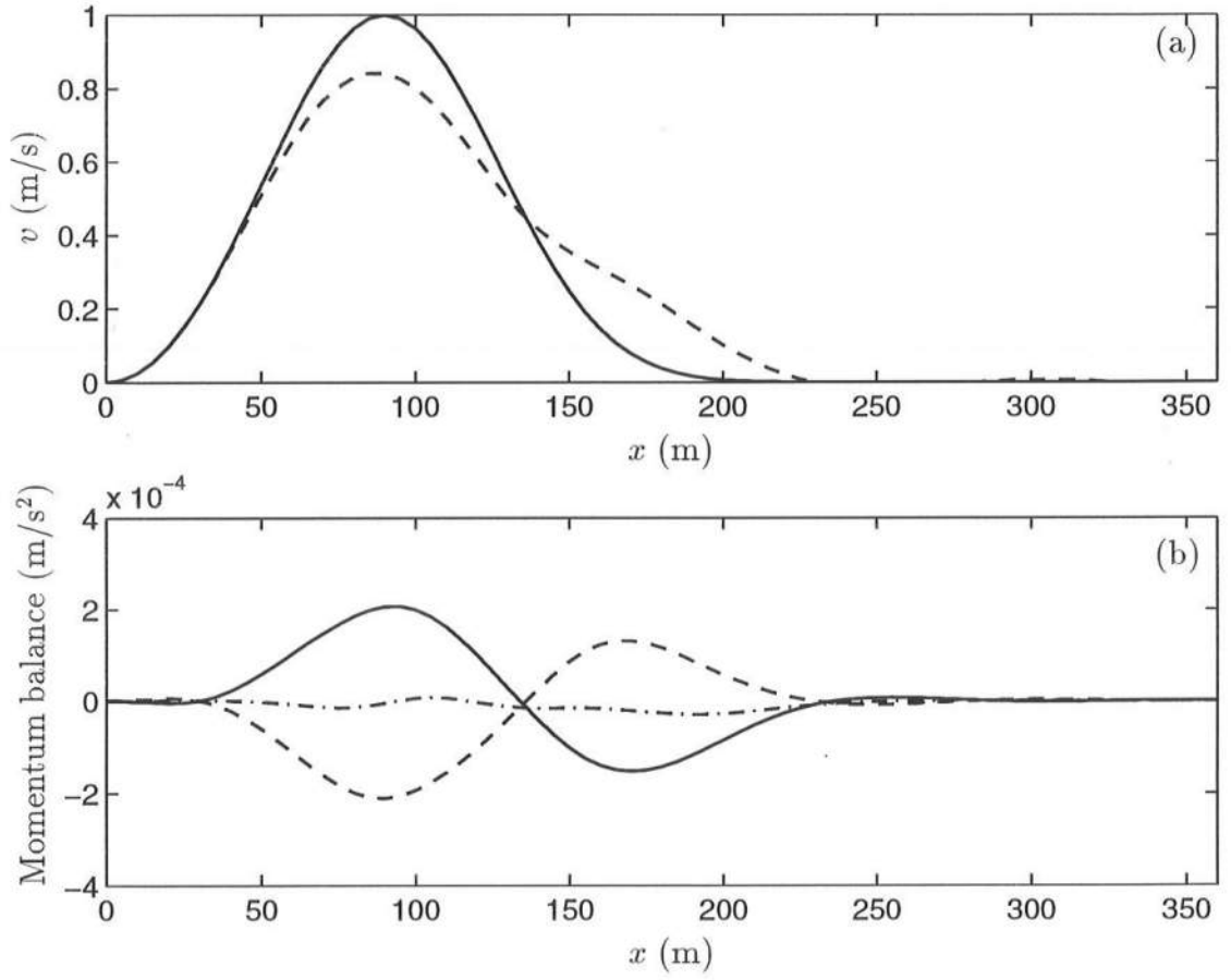
Figure 5.15: ND=2: (a) Initial (—) and final (---) mean current profiles. (b) Longshore-averaged momentum balance. \langle \partial v / \partial t \rangle (- · -), \langle u(\partial v / \partial x) \rangle (---), \langle (\mu/d)(v - V) \rangle (—).
