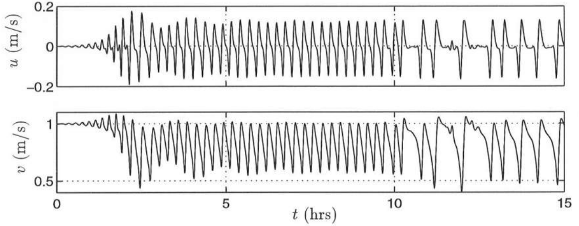
Figure 5.24: ND=16: Time series of u and v at (x, y) = (90 \text{ m}, 0.5L_y) .
