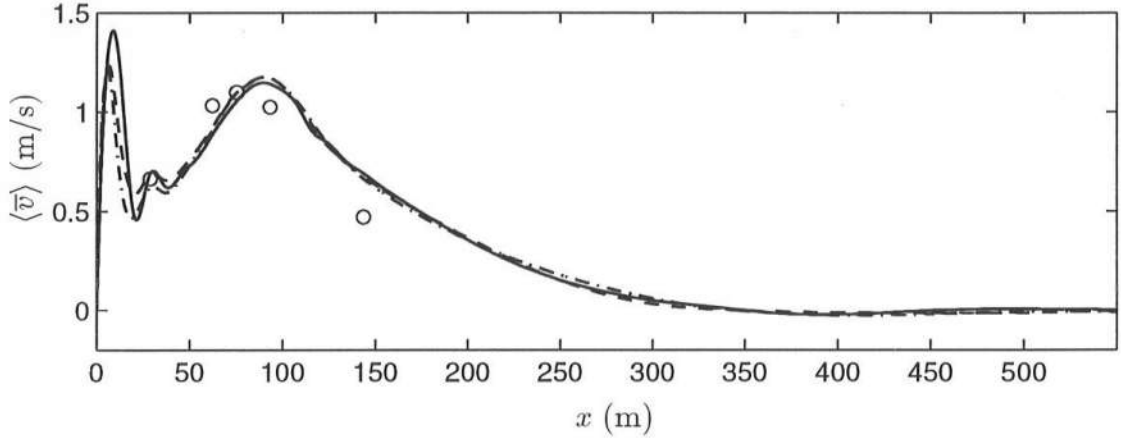
Figure 6.72: October 16: Time and longshore-averaged longshore currents \langle \bar{v} \rangle for c_f = 0.0035 and M = 0 (—), M = 0.25 (---), M = 0.5 (- · -) and sled data ( \circ ).
