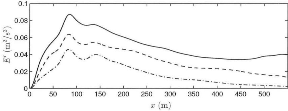
Figure 6.26: October 15: Time and longshore-averaged longshore perturbation kinetic energy \frac{1}{2}\langle u'^2 + v'^2 \rangle for c_f = 0.0015 (—), c_f = 0.002 (---), c_f = 0.003 (- · -).
