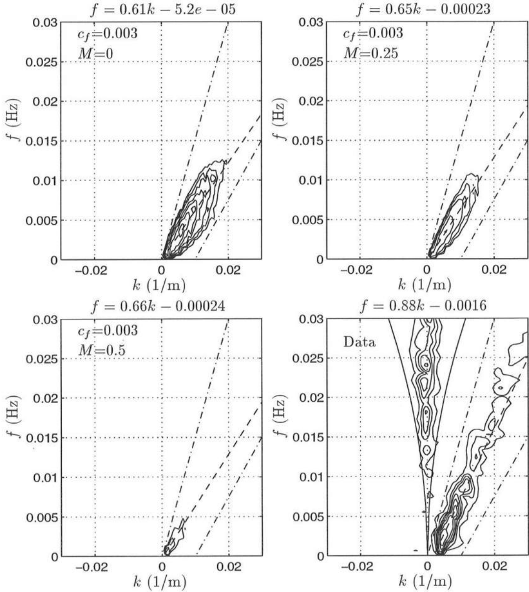
Figure 6.81: October 18: Frequency-cyclic wavenumber spectra S(f, k) ( \text{m}^3/\text{s} ) for computed and measured cross-shore velocity at x = 35 m. The value for c_{est} is 0.75 m/s, and is used in Equation (6.3) to construct the upper and lower cut-off lines ( - \cdot - ) of the shear wave energy. Contour levels plotted are (10, 30, 60, 100, 200, 400, 800). The equation for the best fit dispersion line ( - - ) is noted above each plot.
