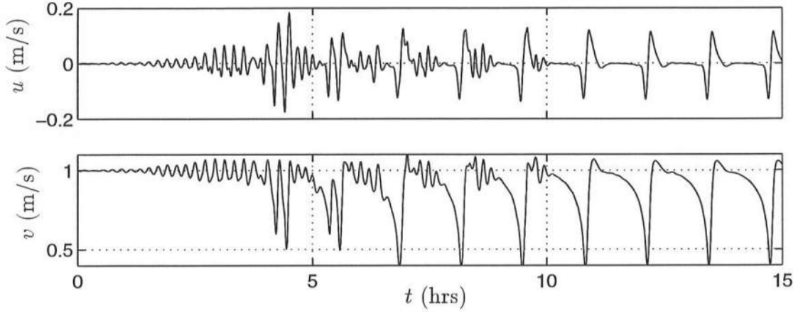
Figure 5.17: ND=4: Time series of u and v at (x, y) = (90 \text{ m}, 0.5L_y) .
