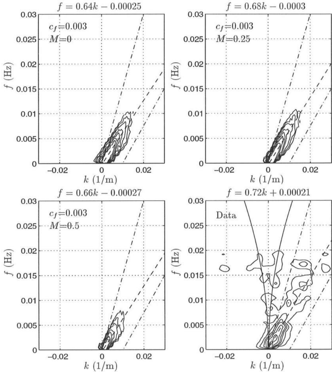
Figure 6.80: October 18: Frequency-cyclic wavenumber spectra S(f, k) ( \text{m}^3/\text{s} ) for computed and measured longshore velocity at x = 35 m. The value for c_{est} is 0.75 m/s, and is used in Equation (6.3) to construct the upper and lower cut-off lines ( - \cdot - ) of the shear wave energy. Contour levels plotted are (10, 30, 60, 100, 200, 400, 800). The equation for the best fit dispersion line ( - - ) is noted above each plot.
