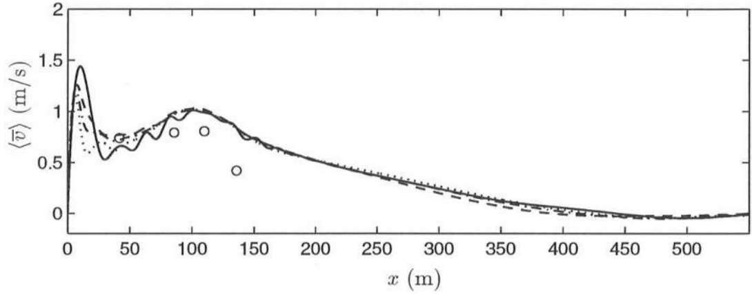
Figure 6.56: October 15: Time and longshore-averaged longshore currents \langle \bar{v} \rangle for c_f = 0.002 and M = 0 (—), M = 0.25 (---), M = 0.5 (- · -), M = 1 (· · ·) and sled data (○).
