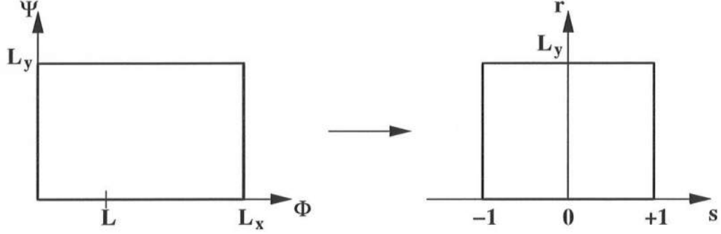
Figure 3.3: Transformation from the intermediate to the computational domain
