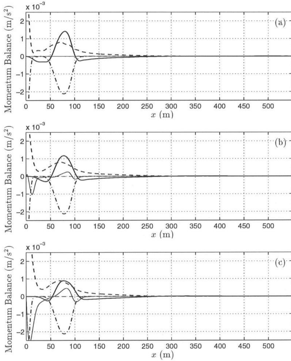
Figure 6.85: October 18: Mean longshore momentum balance for c_f = 0.003 and (a) M = 0 , (b) M = 0.25 and (c) M = 0.5 . \langle u(\partial v / \partial x) \rangle (thick —), -\langle \tilde{\tau}_y \rangle (- · -), -\langle \tau_y^I \rangle (thin —), \langle \frac{\mu}{D} v \rangle (thick - -), residual (thin - -).
