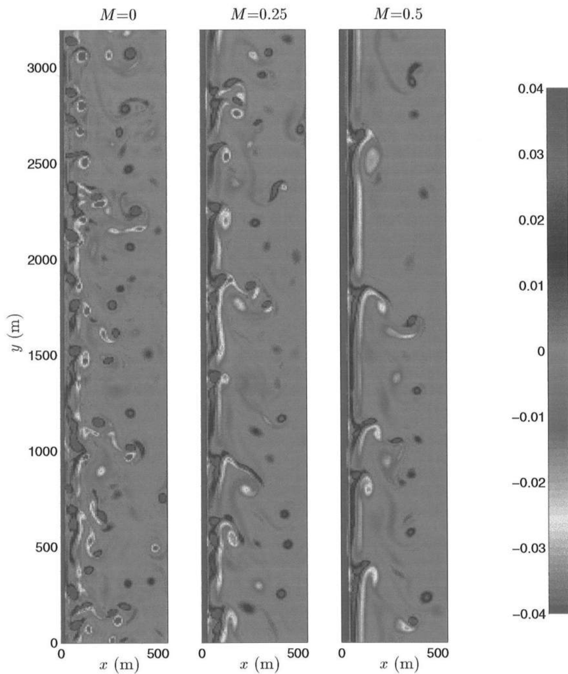
Figure 6.86: October 18: Contour plots of vorticity q ( 1/s ) at t = 5 hrs for c_f = 0.003 and M = 0, 0.25, 0.5 .
