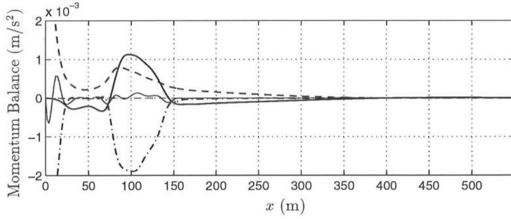
Figure 6.59: October 15: Mean longshore momentum balance for c_f = 0.002 , M = 0.25 . \langle u(\partial v / \partial x) \rangle (thick —), -\langle \tilde{\tau}_y \rangle (- · -), -\langle \tau'_y \rangle (thin —), \langle \frac{\mu}{D} v \rangle (thick - -), residual (thin - -).
