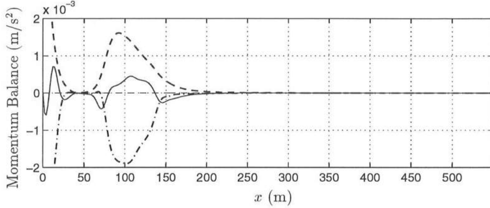
Figure 6.62: October 15: Mean longshore momentum balance in the absence of shear instabilities for c_f = 0.002 and M = 0.25 . -\langle\tilde{\tau}_y\rangle ( - \cdot - ), -\langle\tau_y'\rangle (thin \text{---} ), \langle\frac{\mu}{D}v\rangle (thick \text{---} ), residual (thin - - ).
