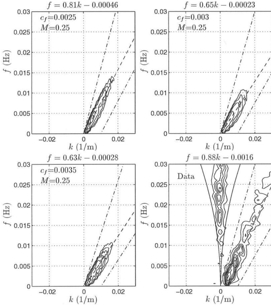
Figure 6.48: October 18: Frequency-cyclic wavenumber spectra S(f, k) ( \text{m}^3/\text{s} ) for computed and measured cross-shore velocity at x = 35 m. The values for c_{est} are 0.8 m/s for c_f = 0.0025 , 0.75 for c_f = 0.003 , 0.65 m/s for c_f = 0.0035 , and 0.75 m/s for data, and are used in Equation (6.3) to construct the upper and lower cut-off lines (---) of the shear wave energy. Contour levels plotted are (10 30 60 100 200 400 800). The equation for the best fit dispersion line (---) is noted above each plot.
