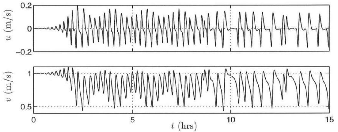
Figure 5.20: ND=8: Time series of u and v at (x, y) = (90 \text{ m}, 0.5L_y) .
