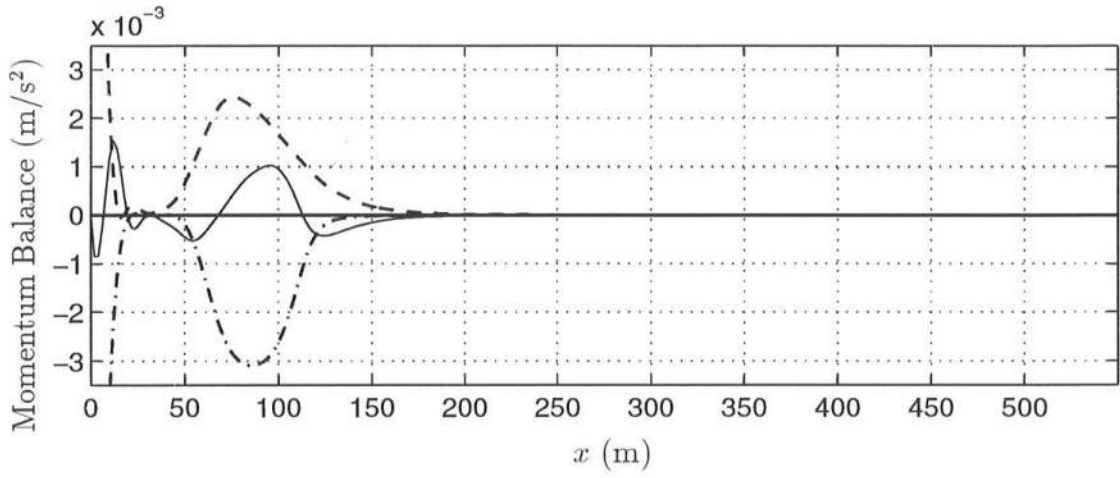
Figure 6.75: October 16: Mean longshore momentum balance in the absence of shear instabilities for c_f = 0.0035 and M = 0.5 . -\langle\tilde{\tau}_y\rangle ( - \cdot - ), -\langle\tau_y^I\rangle (thin — ), \langle\frac{\mu}{D}v\rangle (thick - - ), residual (thin - \cdot - ).
