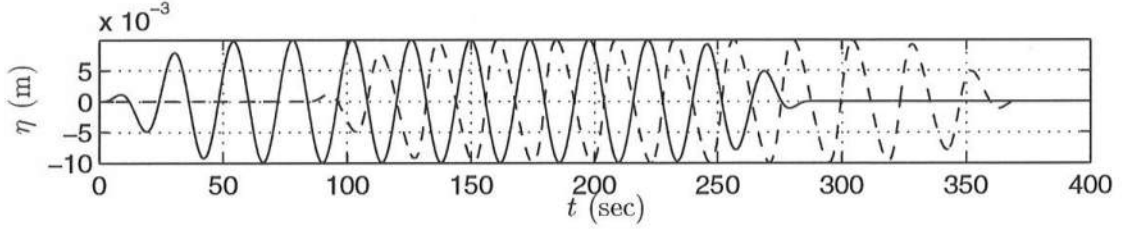
Figure 4.4: Simultaneous absorption-generation: Incoming wave (—) and outgoing wave (— —). R_{ag} = 6.3 \times 10^{-4} , R_a = 1.9 \times 10^{-4}
