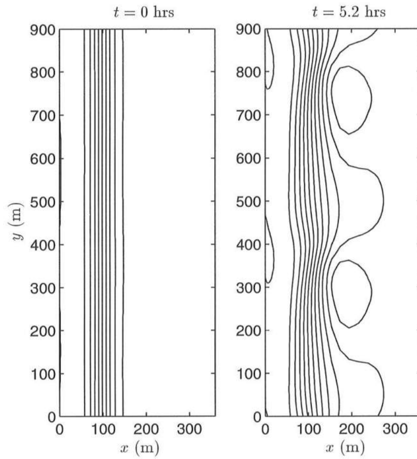
Figure 5.11: ND=2: Snapshots of streamlines
