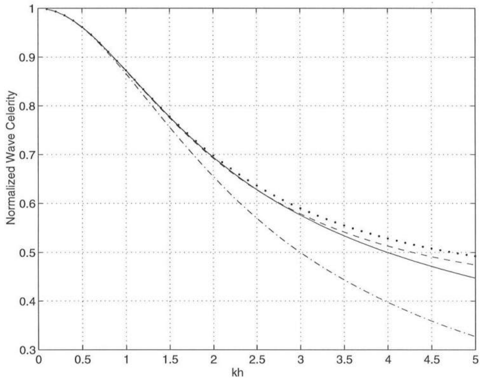
Figure 1: Comparison of linear dispersion relationships: solid line – exact solution; dash line – \alpha = -0.390 , optimal value ; dotted line – \alpha = -2/5 , (2,2) Padé approximant; dash-dot line – \alpha = -1/3 .
