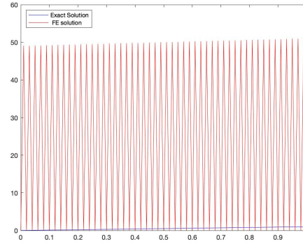
Fig.2: f = 1, n = 102, \varepsilon = 10^{-6}
