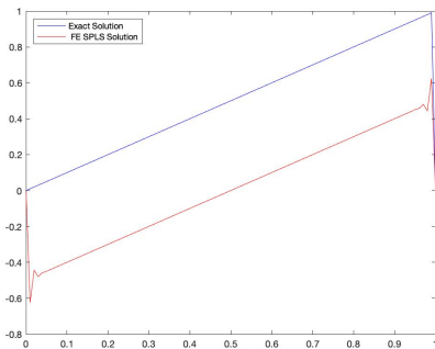
Fig.7: f = 1, n = 101, \varepsilon = 10^{-6}
