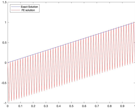
Fig.1: f = 1, n = 101, \varepsilon = 10^{-6}
