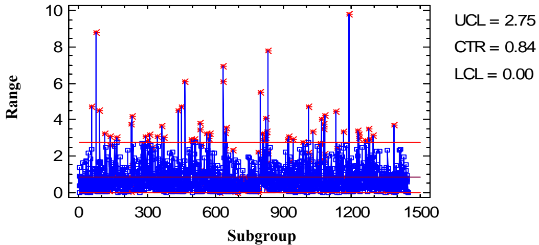
Range chart for Density of Core
