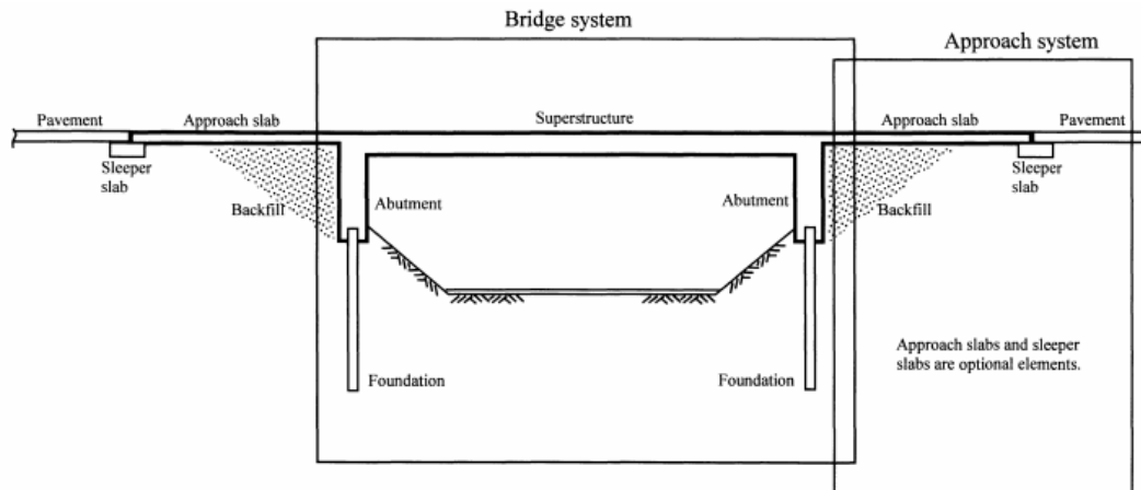
Figure 6. Diagram. Simplified geometry of an integral abutment bridge. Figure 1. Simplified geometry of an integral abutment bridge. Reprinted from The Behavior of Integral Abutment Bridges , by S. Arsoy et al., 1999, FHWA/VTRC 00-CR3 , p.2. Copyright [1999] by Virginia Department of Transportation.
