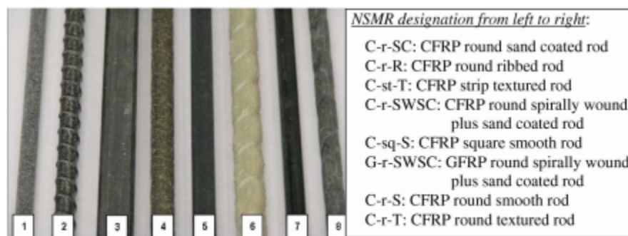
Figure 1. Photo. Illustration of various FRP NSM reinforcements. Reprinted from “Assessing the strengthening effect of various near-surface-mounted FRP reinforcements on concrete bridge slab overhangs” by D. Lee & L. Cheng, 2011, Journal of Composites for Construction, 15(4), p.616.
