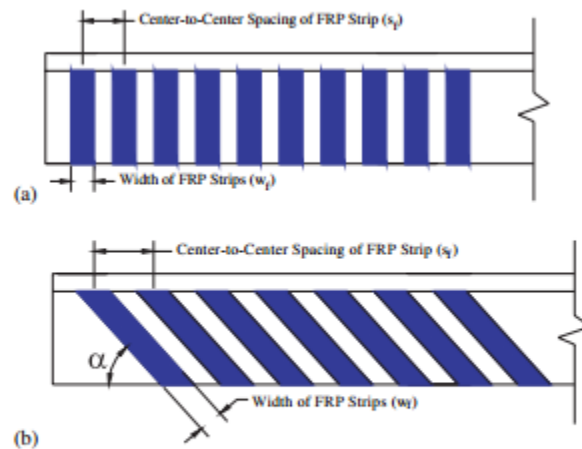
Figure 14. Diagram. Strengthening Scheme: Side View – (a) Fibers at 90° direction, and (b) Fibers at Inclined Direction. Figure B3.2. Strengthening Scheme: Side View. Reprinted from Design for FRP systems for strengthening concrete girders in shear , by A. Belarbi et al., 2011, NCHRP 678 , p.62. Copyright [2011] by National Academy of Sciences.
