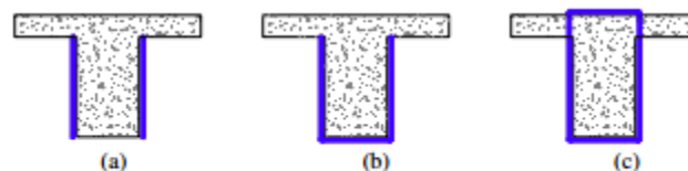
Figure 13. Diagram. Strengthening Scheme: Cross-Sectional View. (a) Side bonding, (b) U-wrap, and (c) Complete wrap. Figure B3.1. Strengthening Scheme: Cross-Sectional View. Reprinted from Design for FRP systems for strengthening concrete girders in shear , by A. Belarbi et al., 2011, NCHRP 678 , p.61. Copyright [2011] by National Academy of Sciences.
