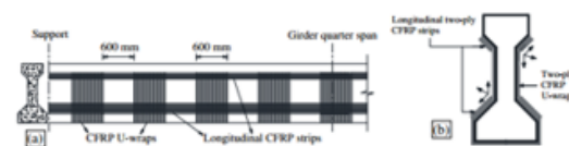
Proposed CFRP arrangement (a) along girder elevation; (b) on the cross-section
