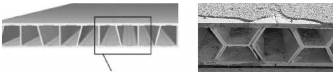
Figure 12. Photo. Pultruded hollow core sandwich configuration. Figure 3.3.3-1. Pultruded hollow core sandwich configuration. Reprinted from Field inspection of in-service FRP bridge decks , by N.M. Telang et al., 2006, NCHRP 564 , p.20. Copyright [2006] by Transportation Research Board.
