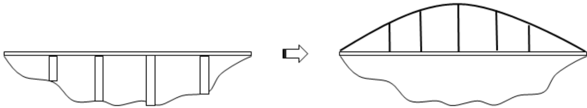
Figure 5. Diagram. Conversion of a continuous multi-span bridge to a network arch bridge.
