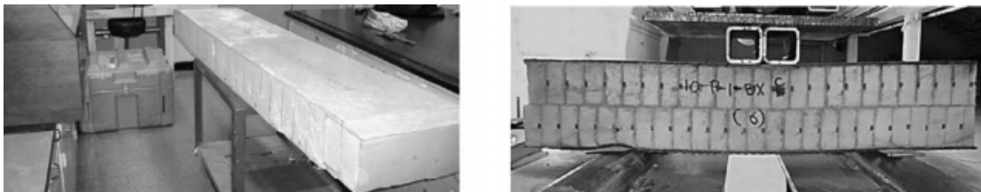
Figure 11. Photo. Solid core sandwich configuration. Figure 3.3.2-1. Solid core sandwich configuration. Reprinted from Field inspection of in-service FRP bridge decks , by N.M. Telang et al., 2006, NCHRP 564 , p.19. Copyright [2006] by Transportation Research Board.
