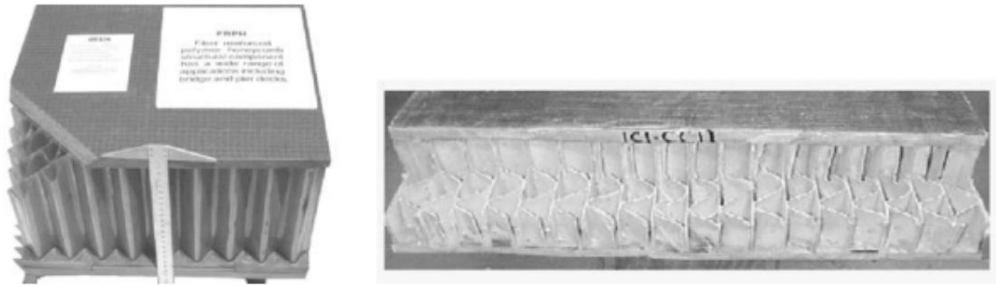
Figure 10. Photo. Honeycomb sandwich configuration. Figure 3.3.1-1. Honeycomb sandwich configuration. Reprinted from Field inspection of in-service FRP bridge decks , by N.M. Telang et al., 2006, NCHRP 564 , p.19. Copyright [2006] by Transportation Research Board.
