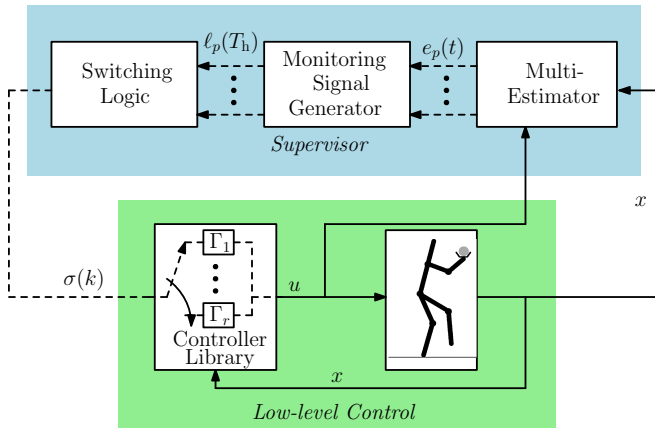
Fig. 1. Supervisory control block diagram. The high-level supervisor is shown in blue and the low-level execution loop is shown in green. At every step, the switching signal \sigma(k) engages a controller from the controller library and the within-step supervisor assesses its performance using the multi-estimator and the monitoring signal generator components.
