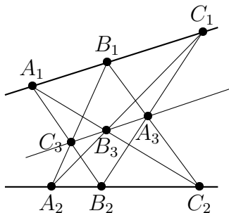
Figure 1: Diagram of the Pappus configuration in a projective plane.
