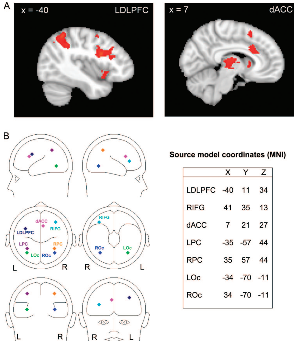
Figure 1. (A) Left dorsolateral prefrontal cortex (LDLPFC) and dorsal anterior cingulate cortex (dACC) activation for incongruent versus congruent stimuli ( z = 3.0902 , p = .01 , cluster size = 34; corrected p < .05 ). Crosshairs placed at center of intensity. (B) Functional MRI Montreal Neurological Institute (MNI) coordinates for source model containing seven regional sources used in brain electrical source analysis source modeling. L = left; R = right; RIFG = right inferior frontal gyrus; LPC = left parietal cortex; RPC = right parietal cortex; LOc = left occipital cortex; ROc = right occipital cortex. Adapted from “The Time Course of Activity in Dorsolateral Prefrontal Cortex and Anterior Cingulate Cortex During Top-Down Attentional Control,” by R. L. Silton, W. Heller, D. N. Towers, A. S. Engels, J. M. Spielberg, J. C. Edgar, . . . G. A. Miller, 2010, NeuroImage , 50, p. 1296. Copyright 2010 by Elsevier.
