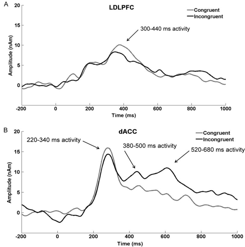
Figure 3. (A) Grand-average source waveforms for left dorsolateral prefrontal cortex (LDLPFC) elicited during the color–word Stroop task for congruent and incongruent conditions, highlighting the 300–440-ms scoring window. N = 100 . (B) Grand-average source waveforms for dorsal anterior cingulate cortex (dACC) elicited during the color–word Stroop task for congruent and incongruent conditions, highlighting the 220–340-ms and 520–680-ms scoring windows. N = 100 . From “The Time Course of Activity in Dorsolateral Prefrontal Cortex and Anterior Cingulate Cortex During Top-Down Attentional Control,” by R. L. Silton, W. Heller, D. N. Towers, A. S. Engels, J. M. Spielberg, J. C. Edgar, . . . G. A. Miller, 2010, NeuroImage , 50, p. 1298. Copyright 2010 by Elsevier.
