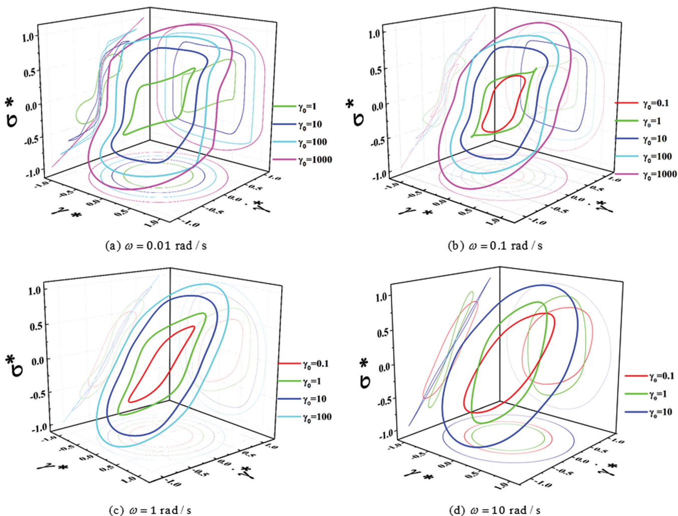
FIG. 8. (a) LAOS data at \omega = 0.01 (rad/s) over a range of strain amplitudes (LAOS data normalized by maximum values, then normalized stress values scaled by 0.5, 0.67, 0.83, and 1 for \gamma_0 = 1, 10, 100 , and 1000, respectively, for presentation purposes). (b) LAOS data at \omega = 0.1 (rad/s) over a range of \gamma_0 (LAOS data normalized by maximum values, then normalized stress values scaled by 0.33, 0.5, 0.67, 0.83, and 1 for \gamma_0 = 0.1, 1, 10, 100 , and 1000, respectively, for presentation purposes). (c) LAOS data at \omega = 1 (rad/s) over range of \gamma_0 (LAOS data normalized by maximum values, then normalized stress values scaled by 0.5, 0.67, 0.83, and 1 for \gamma_0 = 0.1, 1, 10 , and 100, respectively, for presentation purposes). (d) LAOS data at \omega = 10 (rad/s) over range of \gamma_0 (LAOS data normalized by maximum values, then normalized stress values scaled by 0.67, 0.83, and 1 for \gamma_0 = 0.1, 1 , and 10, respectively, for presentation purposes).
