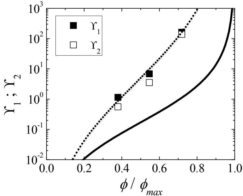
Figure 14. First (closed symbols) and second (open symbols) normal stress difference coefficients for suspensions of cubic particles in the shear-thickened state as a function of the proximity to maximum packing. The solid line is a semi-empirical model of the first normal stress difference coefficient for dispersions of spherical colloids in the shear-thickened state from Morris and Boulay 17 with the model prefactor coefficient reported by Cwalina and Wagner 8 (Equation 14). The dashed line is the model fit to the first normal stress difference coefficient data for suspensions of cubic particles using the modified lubrication form (Equation 15). The model fits of the second normal stress difference coefficient data for suspensions of spheres and cubes are not shown as they both differ from their respective first normal stress difference coefficient models only by small values of the prefactor constants.
