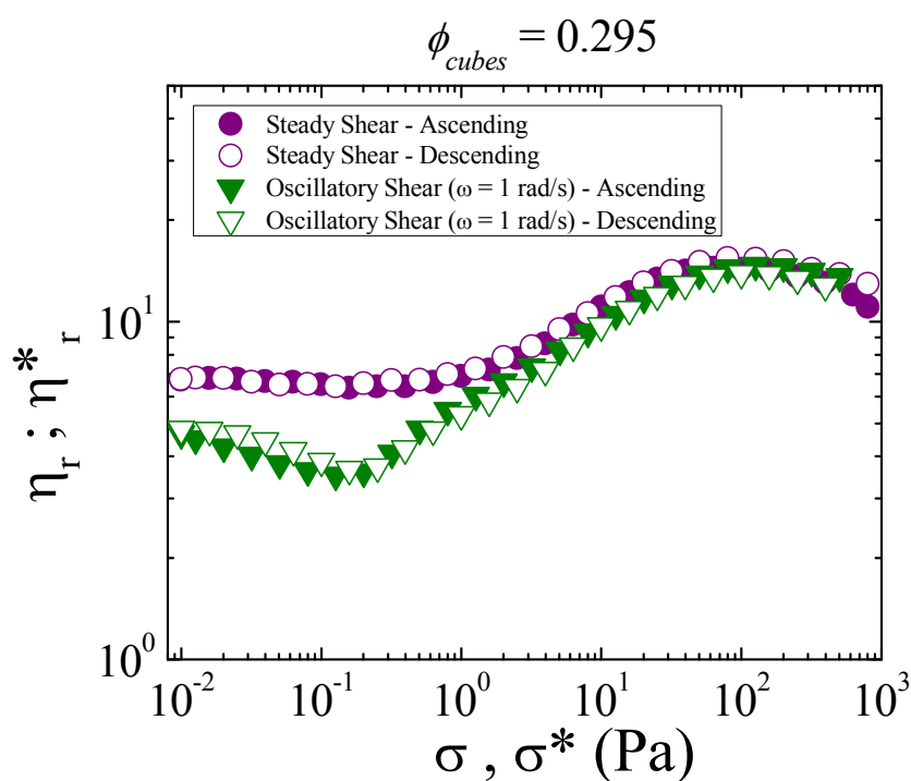
Figure 4. Relative steady shear viscosity (circles) and relative complex viscosity for a \phi_{cubes} = 0.295 suspension measured at \omega = 1 rad/s (triangles) as a function of the applied shear stress and shear stress-amplitude, respectively. Sweeps in the ascending (filled symbols) and descending (open symbols) directions demonstrate the reversibility of the measurements.
