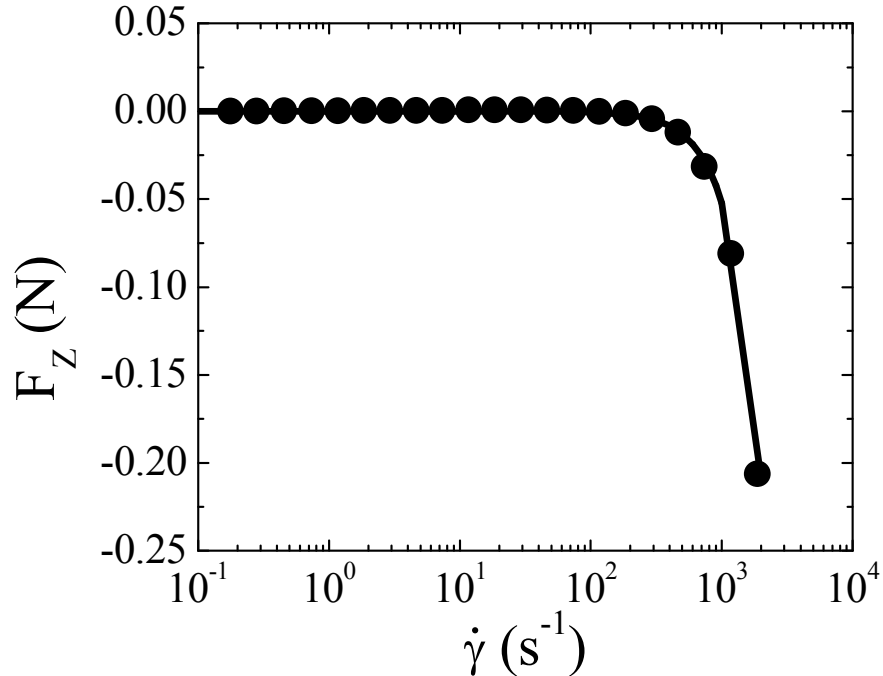
Figure A.1. Measured axial thrust as a function of the applied shear rate for a Newtonian PEG-200 solvent using a 40 mm 2^0 cone and plate tooling. The solid line is the expected contribution to the axial thrust from inertia given by Equation A.1.
