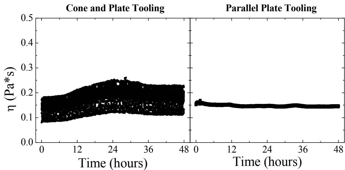
Figure 6. Viscosity measured for a \phi_{\text{cubes}} = 0.295 suspension during a steady shear peak hold at \sigma = 0.1 Pa following overnight sedimentation performed in cone and plate (left) and parallel plate (right) geometries. For comparison, the magnitude of the steady shear viscosity before sedimentation is given in Figure 5.
