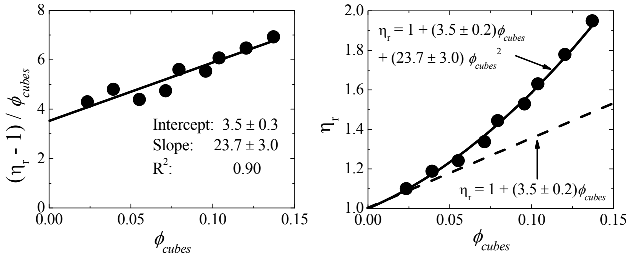
Figure 3. (Left) Data analyzed according to Equation 2 with values of k_E and k_H extracted from the y-intercept and slope, respectively. (Right) Concentration dependence of the suspension viscosity in the dilute and semi-dilute concentration regimes. The dashed line contains the isolated particle contribution to the suspension viscosity and the solid line contains the additional \phi^2 dependence outside the dilute regime.
