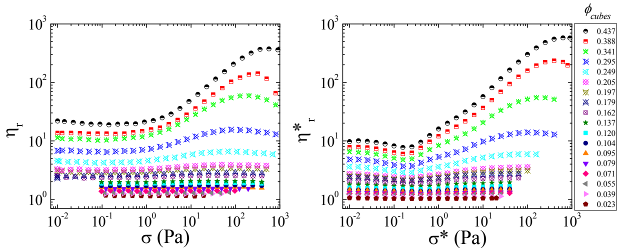
Figure 7. Steady shear viscosity as a function of the applied shear stress (left) and complex viscosity measured at 1 rad/s as a function of the applied shear stress-amplitude (right). All measurements were reversible, but only sweeps in the ascending direction are shown (see Figure 4 for a demonstration of the reversibility).
