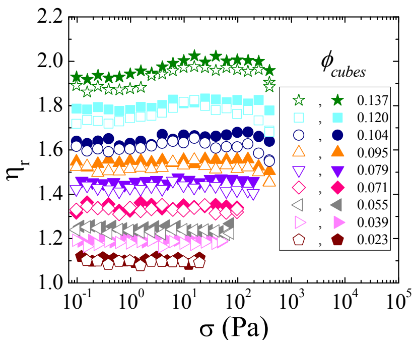
Figure 2. Steady shear viscosity plotted as a function of the applied shear stress for dilute and semi-dilute suspensions of cubic particles in a Newtonian PEG-200 suspending medium. The filled and open symbols mark steady flow sweeps in the descending and ascending directions.
