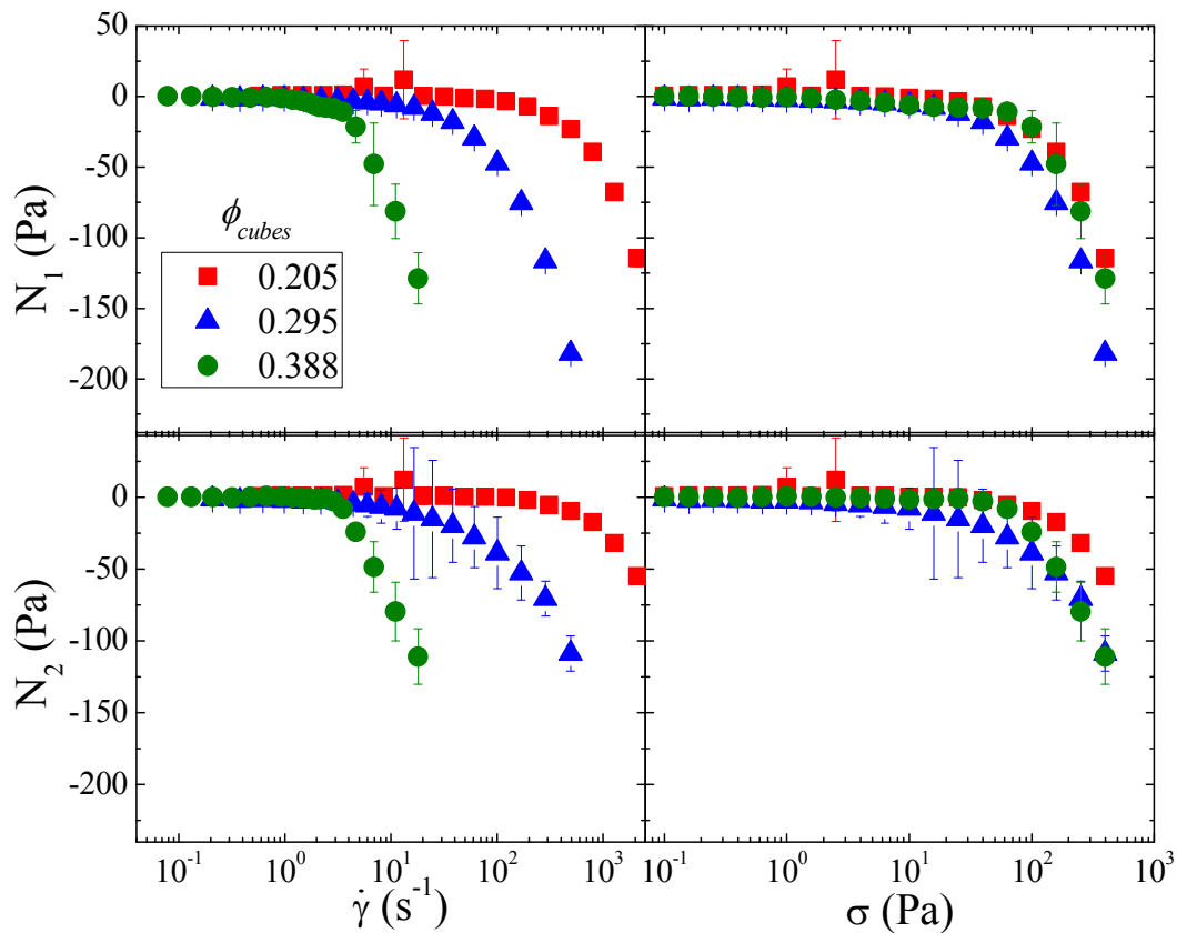
Figure 11. First (top) and second (bottom) normal stress difference as a function of the shear rate (left) and shear stress (right) for selected volume fractions.
