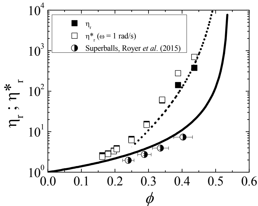
Figure 9. Steady shear viscosity (filled symbols) and complex viscosity (open symbols) measured in the shear-thickened state for suspensions of cubic particles. The solid line is the model fit to the measured viscosity of the shear-thickened state for suspensions of spherical particles from Cwalina and Wagner 8 . The dashed line is the predicted value of the viscosity in the shear-thickened state for suspensions of cubic particles where the lubrication squeeze flow is modified from spheres to cubes (Equation 11). The half-filled circles are the viscosity in the shear-thickened state measured by Royer et al. 45 for suspensions of superballs.
