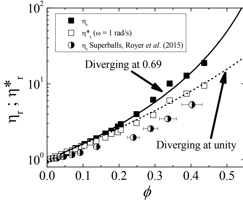
Figure 8. Low shear steady (closed) and complex (open) viscosity as a function of the volume fraction of cubic particles. The solid and dotted lines are fits to the steady shear viscosity and complex viscosity, respectively, using a modified Eilers equation with an adjustable power law exponent. The half-filled circles mark the low shear viscosity under steady shear for suspension of superballs as measured by Royer et al. 45 .
