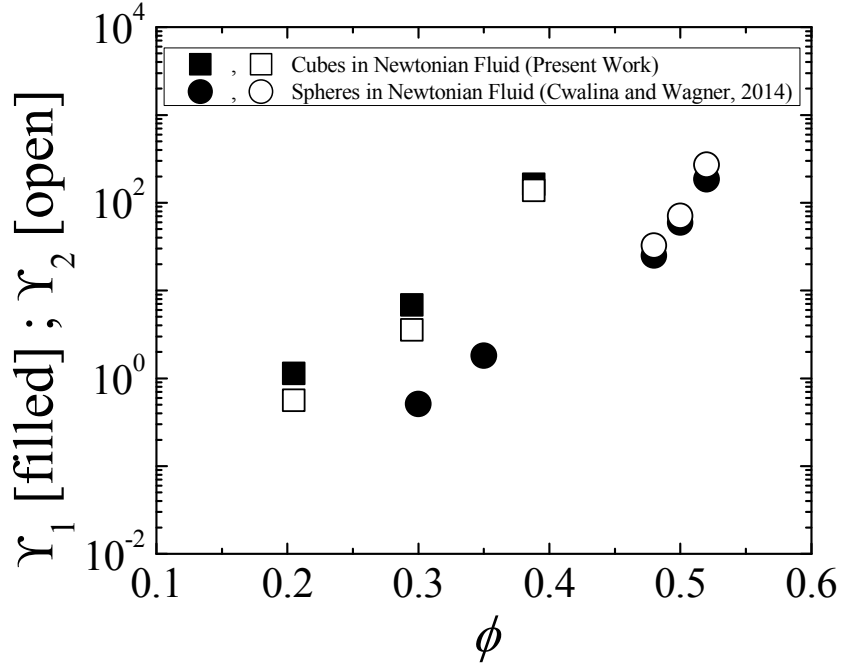
Figure 13. First (filled symbols) and second (open symbols) normal stress difference coefficients for suspensions in the shear-thickened state as a function of the particle volume for the suspensions of cubic particles in a Newtonian fluid considered in the present work (squares) and those measured previously for spherical colloids in a Newtonian fluid by Cwalina and Wagner 8 . Error bars are smaller than data points.
