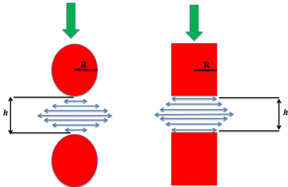
Figure 10. Lubrication squeeze flow between two spherical particles (left) and two cubic particles (right) with an identical characteristic half-width, R .
