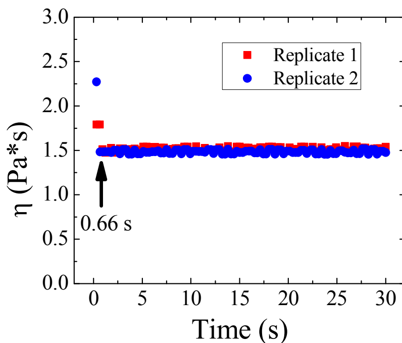
Figure C.1 Steady shear peak hold performed at \sigma = 0.1 Pa on a Newtonian viscosity standard (Cannon) following 300 seconds of oscillation at \sigma^* = 0.1 Pa and \omega = 1 rad/s. Two replicate experiments were performed to establish the lag time of the instrument.
