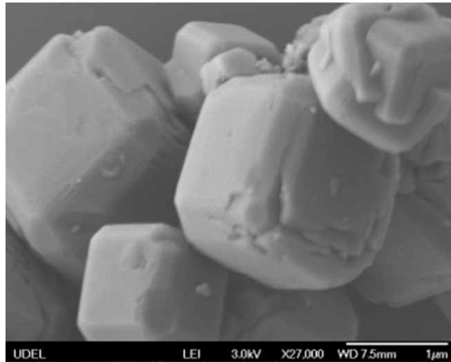
Figure 1. SEM image of cubic aluminosilicate zeolite particles used in this study. The scale bar in the lower right is 1 \mu\text{m} .
