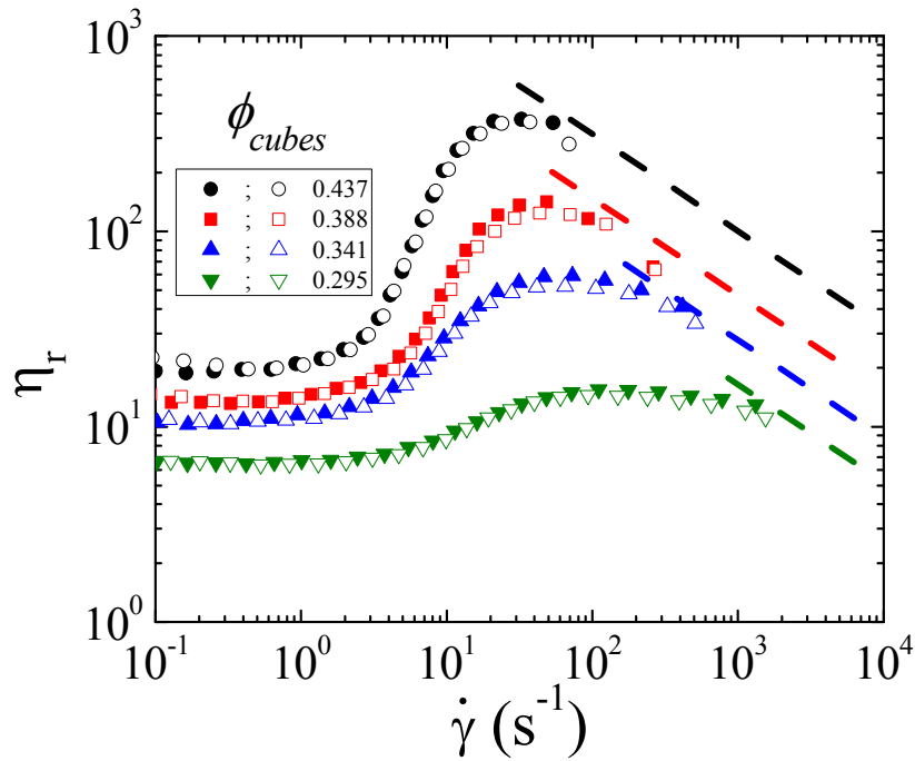
Figure B.1 Predicted elastohydrodynamic scaling (dashed lines) for the relative viscosity as a function of the shear rate for concentrated suspensions of cubic particles.
