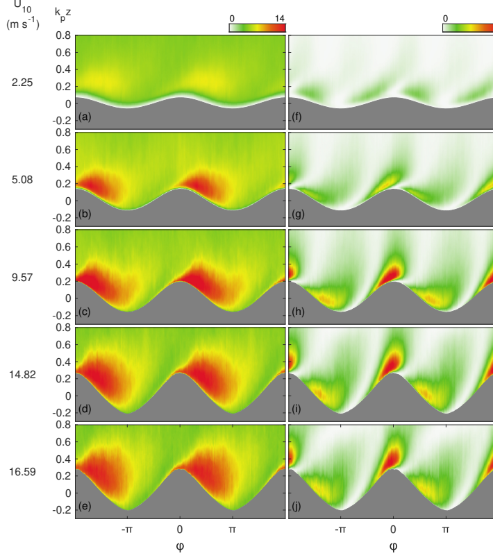
FIGURE 2. Wave-phase coherent distributions of the normalized (a-e) TKE, \langle e_t \rangle / u_*^2 , and (f-j) WKE, \langle e_w \rangle / u_*^2 , where e_t = 3(U_1'U_1' + U_3'U_3')/4 and e_w = (\bar{U}_1\bar{U}_1 + \bar{U}_3\bar{U}_3)/2 , for all experimental conditions. The wave-phase coherent fields are plotted above the mean water surface as a function of the dimensionless distance k_p z . The 10 m wind speeds corresponding to each experimental condition are indicated on the left.
