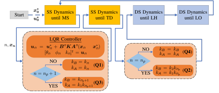
Fig. 4: Overview of the biomechanics-inspired proposed controller. The model is initiated with the optimal state-control pair (x_0^*, u_0^*) to achieve periodic gait with a desired forward velocity at MS. The {MS, TD} and {LH, LO} gait events are identified using single support (SS) and double support (DS) dynamics, respectively. At every MS event, the LQR controller is implemented and the u_n feedback law is derived. During the perturbation step ( n = n_p ), the stiffness of both legs is initially determined by the LQR controller at MS (Q1) and then it is amplified at TD by the control gains k_1 and k_2 (Q2). At the next step ( n = n_p + 1 ), the leg experiencing the perturbation (A) maintains an increased stiffness at MS, while the stiffness of the leg about to land on rigid terrain (B) is determined based on the LQR controller with no adjustment (Q3). Then, at TD, the stiffness of both legs is not altered (Q4). Finally, the stiffness for both legs is determined based on the LQR for all other steps.
