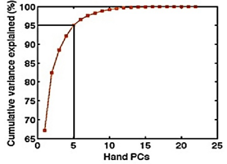
Fig. 3. The cumulative variance for the principal components extracted from the hand kinematics.
