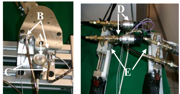
Fig 1. The shoulder joint-first link prototype: Shoulder top view (top), encoder (A), load cells (B), and Bowden cables (C) (bottom left), pressure sensors (D) and potentiometers (E) mated with the pistons (bottom right).
