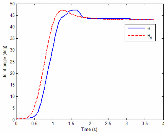
Fig. 8. Joint trajectory
