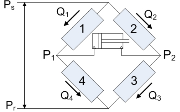
Fig. 5. Three-land-four-way spool valve
