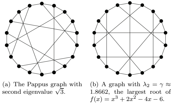
FIG. 4. The 3-regular graphs on 18 vertices with \lambda_2 < 1.9 .
