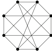
FIG. 3. The 4-regular graph G on 8 vertices with \lambda_2(G) = \sqrt{5} - 1 .
