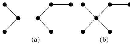
FIG. 1. Graphs with spectral radius greater than 2.
