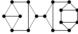
FIG. 5. The unique 3-regular graph with largest least eigenvalue less than -2 .
