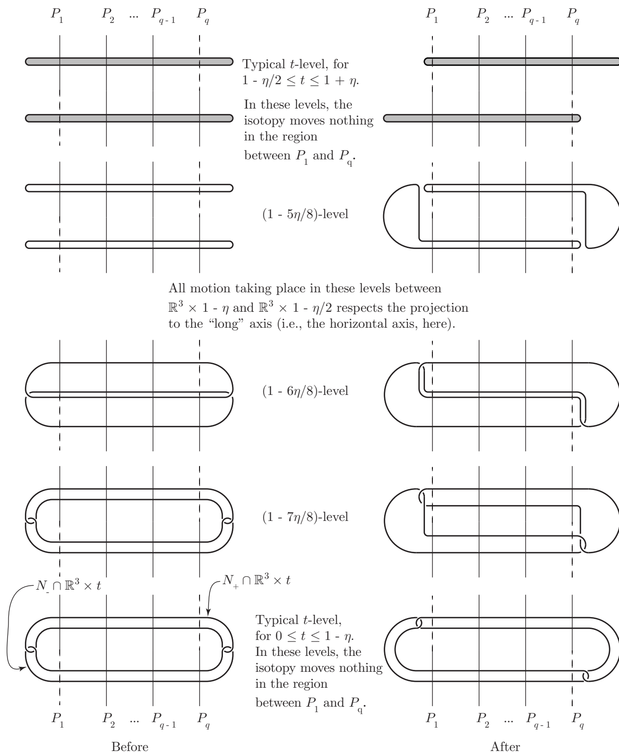
FIGURE IIA-2. The left side shows how N_-^4 \cap N_+^4 is situated in N_0^4 before the isotopy is applied. The right side shows how the image of N_-^4 \cap N_+^4 is situated in N_0^4 after the isotopy is applied, at the end of Step 1.
