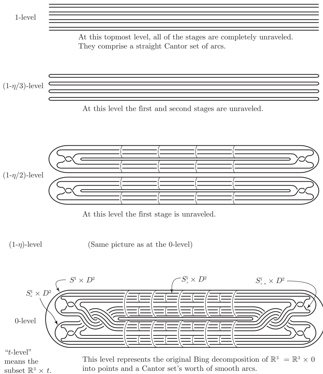
FIGURE IIA-1. Unraveling the original Bing decomposition in \mathbb{R}^3 \times [0, \infty)
