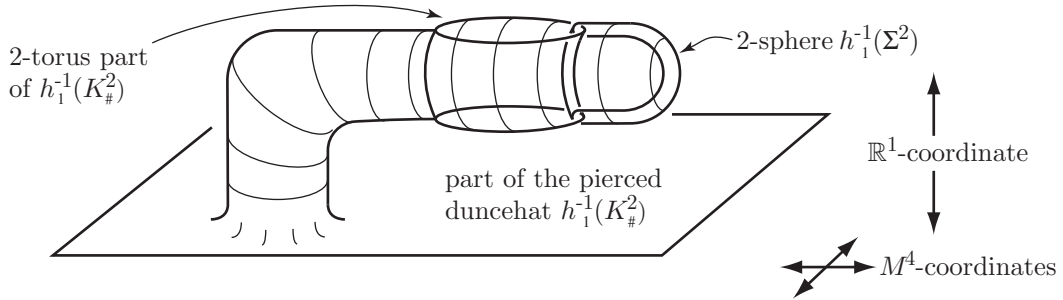
Part (b). Another view of K^2 \times \mathbb{R}^1 \cap h_1^{-1}(M^4 \times 0) , which consists of the pierced duncehat h_1^{-1}(K_{\#}^2) and the 2-sphere h_1^{-1}(\Sigma^2) . The view in Part (a) is a slice of this.
