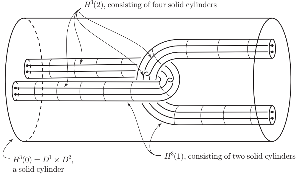
FIGURE II-2. The model handle sequence H^3(0) \supset H^3(1) \supset H^3(2) \supset \dots
