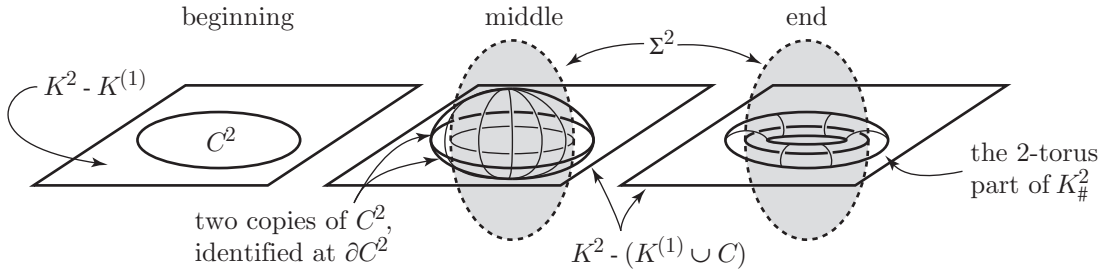
Part (c). Three stages in the growth of the pierced duncehat K_{\#}^2 and the linking 2-sphere \Sigma^2 , taking place in M^4 \times 0 . The 2-sphere \Sigma^2 has dotted lines to indicate that the hemispheres of \Sigma^2 lie in the 4th dimension; only the equator of \Sigma^2 lies in this 3-dimensional slice of M^4 \times 0 .
