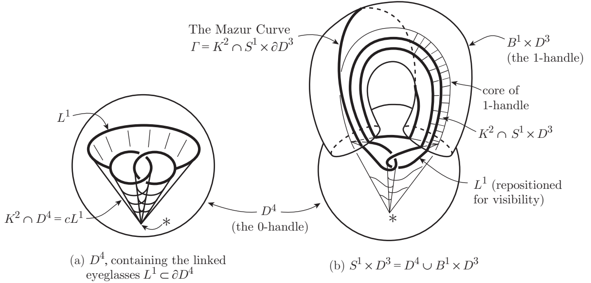
FIGURE I-1. The Mazur 4-manifold M^4 = 0\text{-handle } D^4 \cup 1\text{-handle } B^1 \times D^3 \cup 2\text{-handle } B^2 \times D^2 , and its duncehat spine K^2
