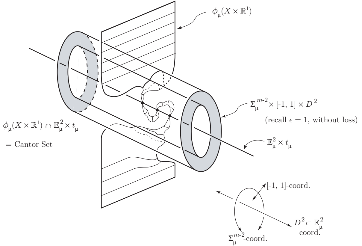
FIGURE II-5. The construction of h_4 and h_\alpha
