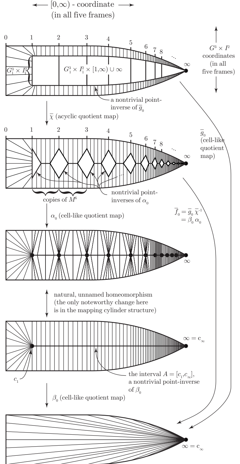
FIGURE IV-1. The nontrivial point inverses of the various maps \bar{\chi} , \alpha_0 , \beta_0 , \bar{g}_0 , and \bar{f}_0 , together with their pinched neighborhoods
