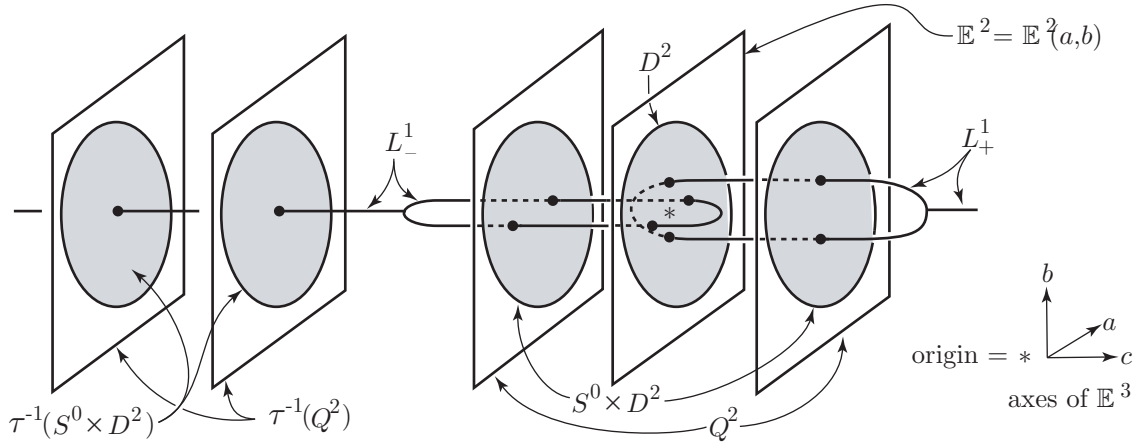
Part (b). The model 3-space \mathbb{E}^3
