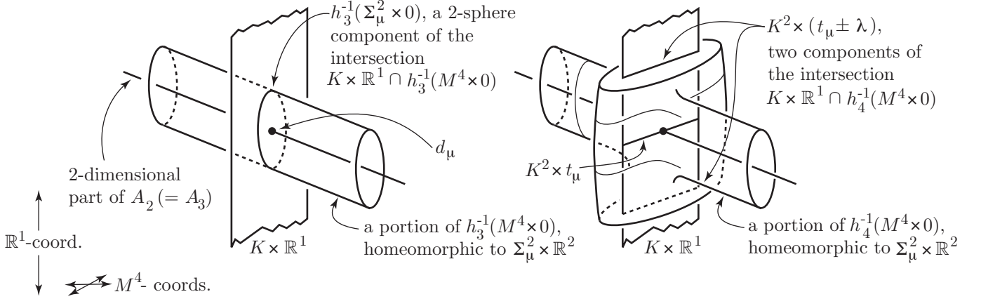
FIGURE I-6. Step i = 4 : the passage from h_3 to h_4
