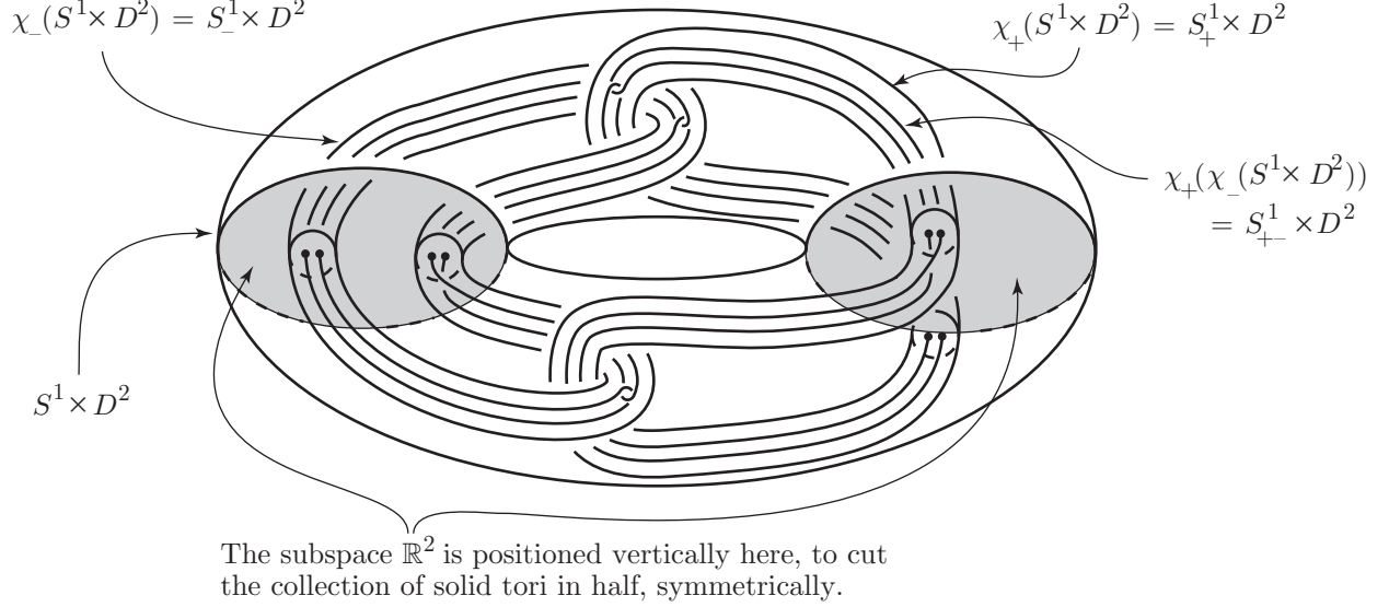
FIGURE I-4. The Bing collection of thickened 1-spheres (i.e., solid tori) in \mathbb{R}^3
