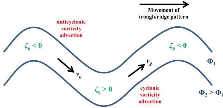
Figure 1. Conceptual view of the movement of middle-tropospheric ridges and troughs from the perspective of the geostrophic vorticity advection forcing term.
