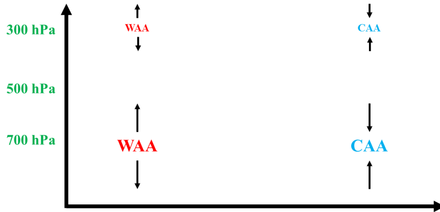
Figure 2. Idealized schematic of the thickness-based interpretation of the effects of (left) warm potential-temperature advection (or WAA) decreasing in magnitude upward and (right) cold potential-temperature advection (or CAA) decreasing in magnitude upward on height tendency at 500 hPa. The black arrows indicate the influence of potential temperature advection upon the local thickness, with larger arrows denoting a larger change in thickness (of either sign); arrows pointing in opposite directions indicating increasing thickness, and arrows pointing toward each other indicating decreasing thickness. At left, the 500 hPa height increases more due to the increased thickness below than it decreases due to the increased thickness above, and thus height tendency is positive. At right, the 500 hPa height decreases more due to the decreased thickness below than it decreases due to the decreased thickness above, and thus height tendency is negative.
