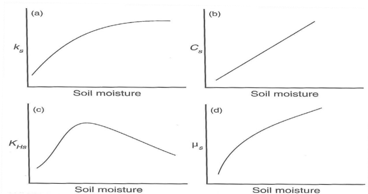
Figure 3. Dependence of (a) thermal conductivity, (b) heat capacity, (c) thermal diffusivity, and (d) thermal admittance on soil moisture. Figure reproduced from Warner (2011), their Fig. 5.2.
