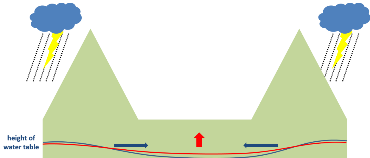
Figure 5. An idealized illustration of thunderstorms contributing to inundation and water table rises (blue) on mountain slopes, after which time lateral transport acts to attempt to restore equilibrium, raising the water table in the valley while lowering it slightly on the mountain slopes (red).
