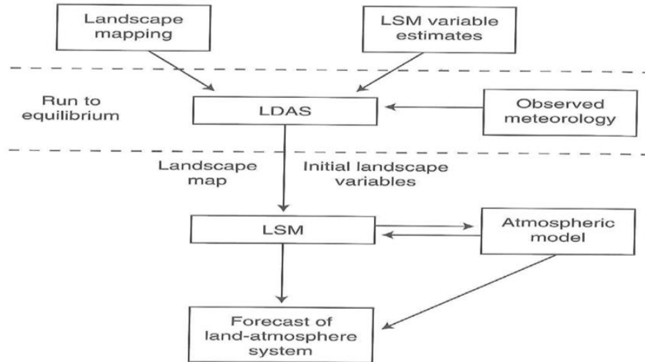
Figure 1. Conceptual schematic of land-surface modeling systems, including the framework of land data assimilation and its role in providing inputs to a coupled atmosphere-land modeling system. Figure reproduced from Warner (2011), their Fig. 5.6.
