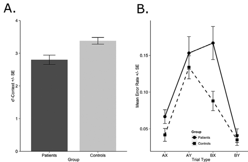
Fig. 1. Dot Pattern Expectancy (DPX) behavioral results. A. d' -context scores on the DPX task. B. Error rates separated by group, trial type. Error bars represent standard error of the mean.
