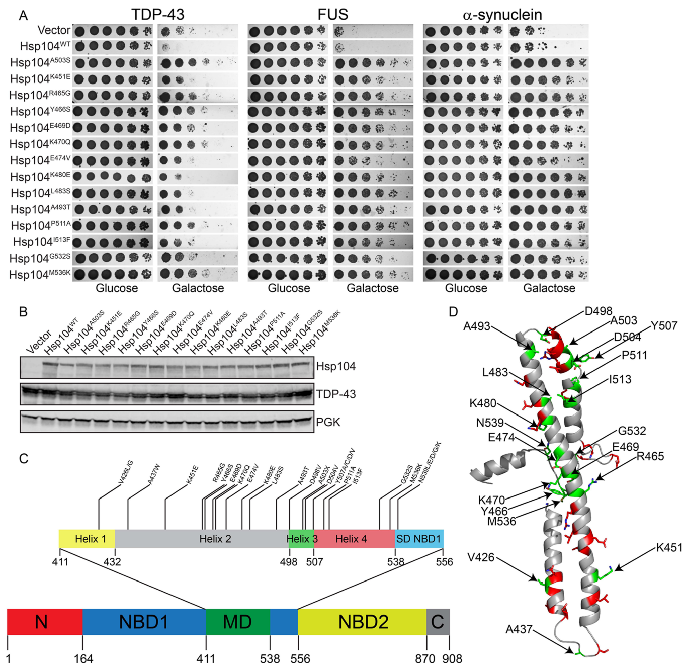
Figure 1. Hsp104 potentiation. Diverse missense mutations in disparate positions throughout the MD and small domain of NBD1 potentiate Hsp104. (A) Δhsp104 yeasts integrated with genes encoding TDP-43, FUS, or \alpha -synuclein were transformed with the indicated Hsp104 missense mutants or control. Strains were serially diluted 5-fold and spotted on glucose (off) or galactose (on) media. (B) Selected strains from A were induced for 5 h, lysed, and immunoblotted. 3-Phosphoglycerate kinase (PGK) serves as a loading control. (C) Potentiating mutations are distributed throughout the MD of Hsp104. The MD (green, residues 411–538) is comprised of four helices and is inserted into nucleotide-binding domain 1 (NBD1, blue). Potentiating mutations shown in this figure are further described in this paper and our earlier work. 17 (D) Homology model of the MD and a portion of the small domain of NBD1 of Hsp104, where side chains studied are shown as sticks. Residues where the tested mutations potentiate Hsp104 are shown in green and are numbered. Residues where the tested mutations do not potentiate Hsp104 are shown in red.
