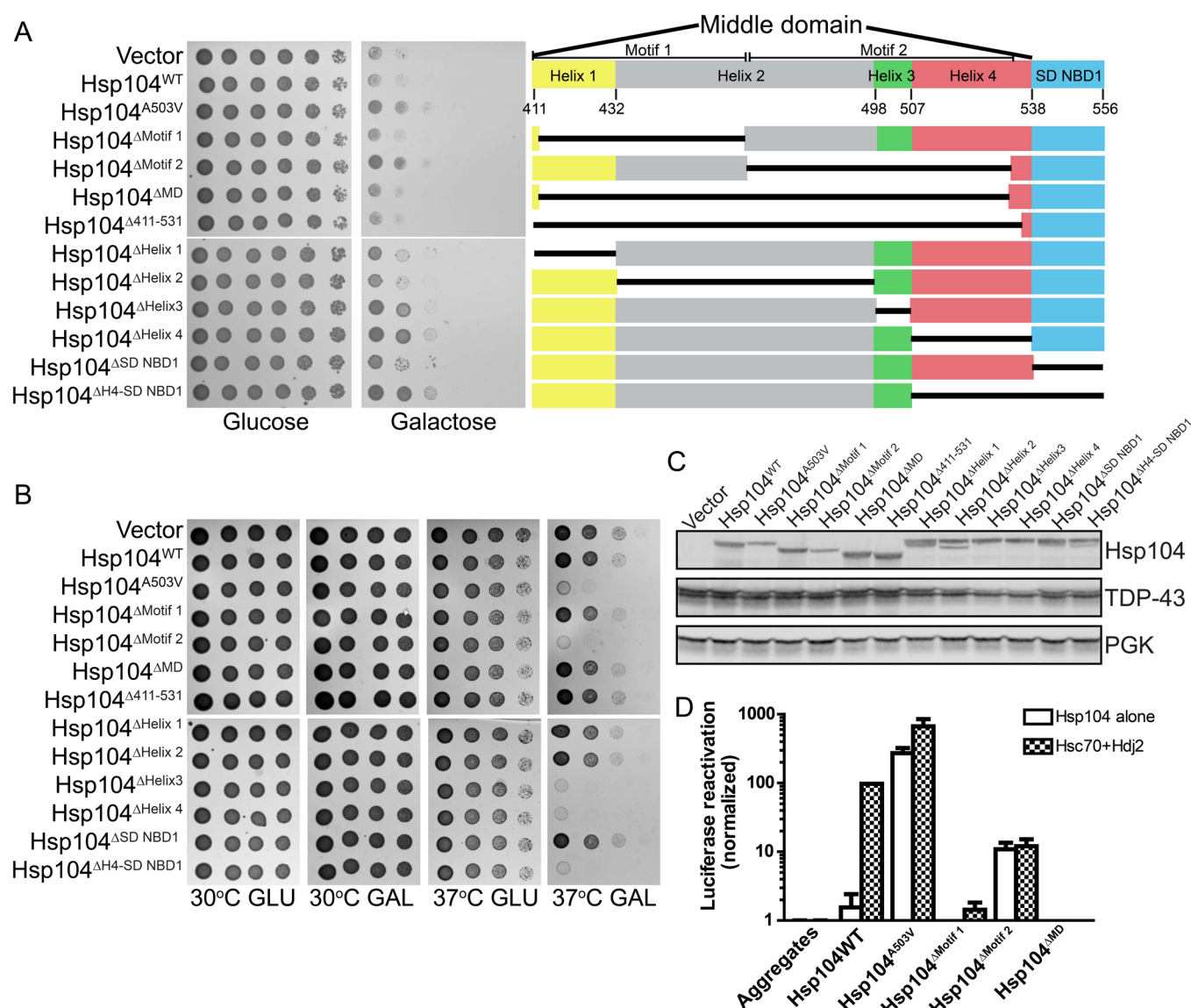
Figure 4. Deletion of Hsp104 MD motifs and helices. Deletion of MD motif 2, helix 3, or helix 4 potentiates Hsp104. (A) W303Δ hsp104 yeasts integrated with pAG303GAL-TDP-43 were transformed with the indicated 416GAL-Hsp104 deletion construct, empty plasmid, Hsp104 WT , or Hsp104 A503V . Strains were serially diluted 5-fold and spotted on glucose (off) or galactose (on) media (left). Organization of the middle domain and small domain of NBD1 (right). (B) W303Δ hsp104 yeasts were transformed with the indicated 416GAL-Hsp104 plasmid or empty vector control. Yeasts were grown to saturation in synthetic raffinose medium, serially diluted, and spotted onto SD-Ura or SGal-Ura media and incubated at 30 or 37 °C. Plates were analyzed after 2–3 days of growth. (C) Selected strains from A were induced for 5 h, lysed, and immunoblotted. 3-Phosphoglycerate kinase (PGK) serves as a loading control. (D) Luciferase aggregates were incubated with the purified Hsp104 variants (0.167 μM hexamer) plus (checkered bars) or minus (clear bars) Hsc70 (0.167 μM) and Hdj2 (0.167 μM). Values represent means ± SEM ( n = 3).
