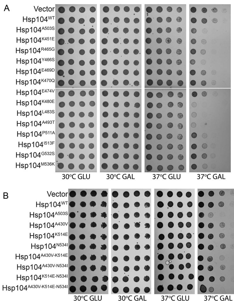
Figure 3. Temperature sensitivity. Novel potentiated Hsp104 variants can display a diminished temperature-sensitive phenotype. (A) W303Δ hsp104 yeasts were transformed with the indicated 416GAL-Hsp104 plasmid or empty vector control. Yeasts were grown to saturation in synthetic raffinose medium, serially diluted, and spotted onto SD-Ura or SGal-Ura media and incubated at 30 or 37 °C. Plates were analyzed after 2–3 days of growth. (B) Experiments were carried out as in A to test the putative synergistic variants.
