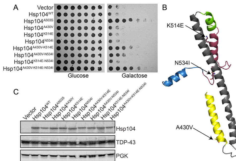
Figure 2. Synergy between mutations in the MD distal loop and helix 4. This synergy yields potentiated Hsp104 variants. (A) \Delta hsp104 yeasts integrated with pAG303GAL-TDP-43 were transformed with each of the indicated pAG416GAL-Hsp104 variants or vector control. Strains were serially diluted 5-fold and spotted on glucose (off) or galactose (on) media. (B) Homology model of the MD and a portion of the small domain of NBD1 of Hsp104. Side chains of the key residues are shown as sticks. (C) Selected strains from A were induced for 5 h, lysed, and immunoblotted. 3-Phosphoglycerate kinase (PGK) serves as a loading control.
