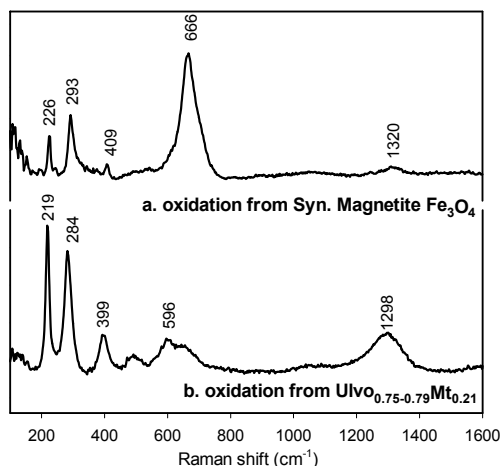
FIGURE 14. Raman peak positions of oxidation products from an end-member magnetite and an \text{Usp-Mgt}_{\text{ss}} grain.
