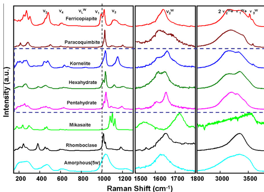
Fig. 2. Raman spectra of eight synthesized anhydrate and hydrated ferric sulfates: ranges from 150 to 1500 \text{cm}^{-1} ( \text{SO}_4 tetrahedra internal and external vibrations), 1500 to 1800 \text{cm}^{-1} (water bending vibrations), and 2600 to 3800 \text{cm}^{-1} (water stretching vibrations), are shown separately.
