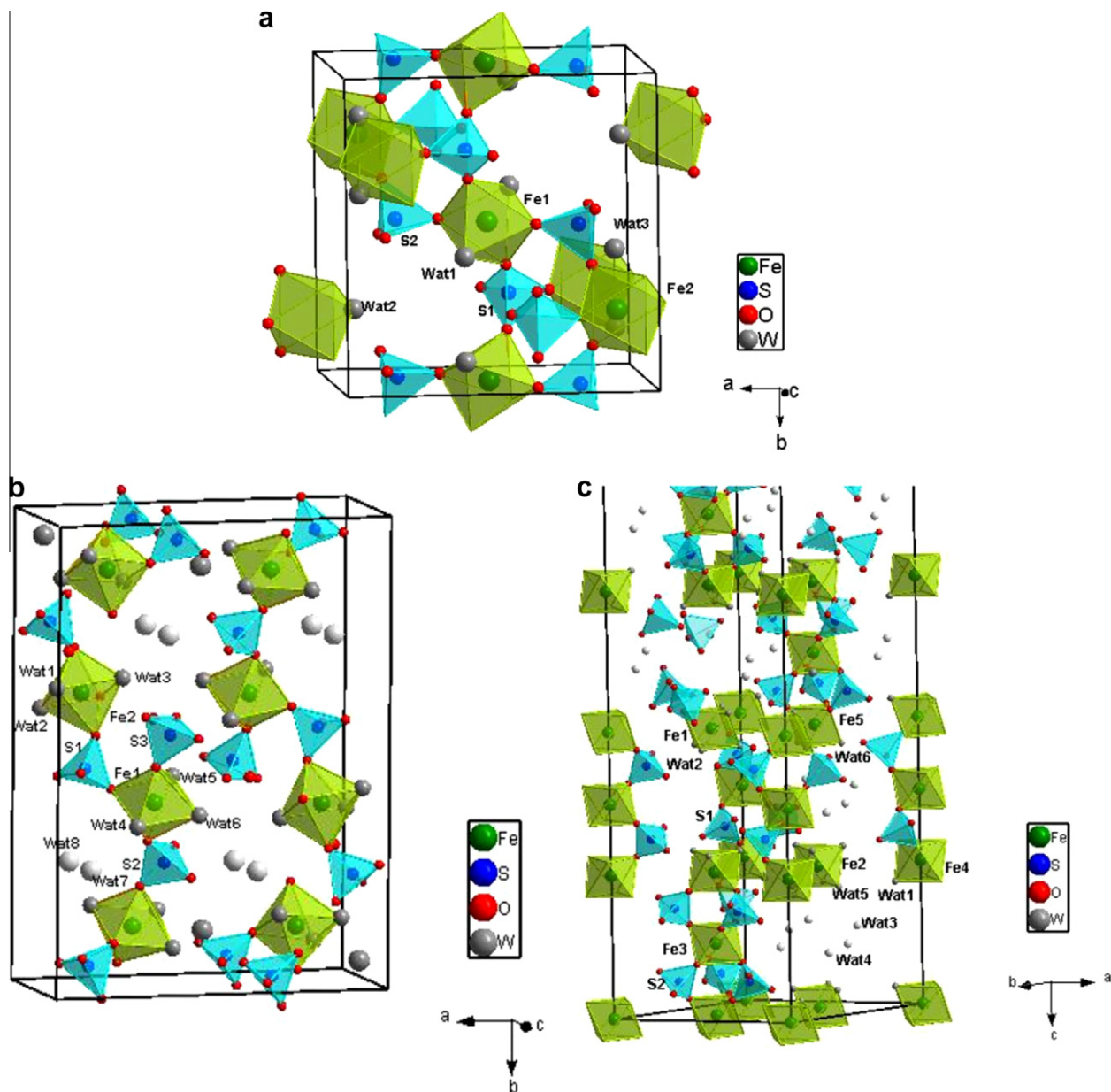
Fig. 1. Polygonal drawings of three hydrated ferric-sulfate structures: (a) pentahydrate; (b) kornelite; (c) paracoquimbite (only show 1/2 of a unit cell).
