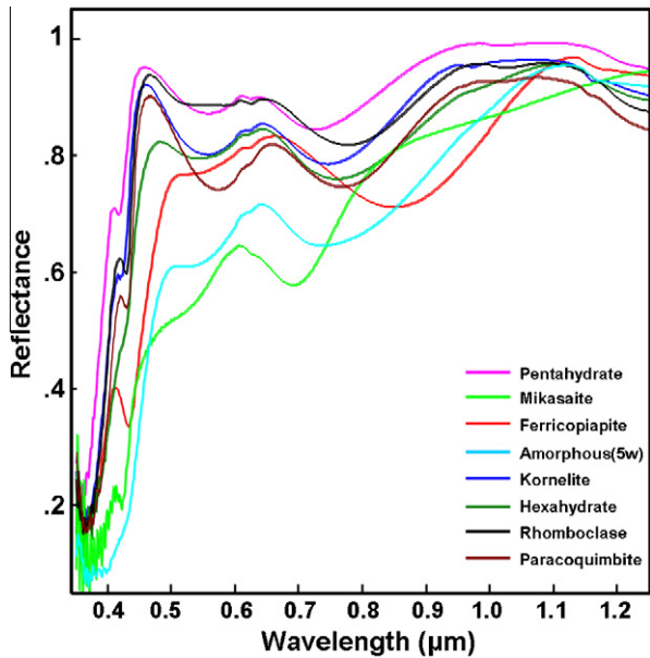
Fig. 5. Vis–NIR reflectance spectra (0.35–1.25 μm) of eight ferric sulfates.
