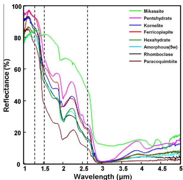
Fig. 4. NIR diffuse reflectance spectra (1–5 \mu\text{m} ) of eight ferric sulfates.
