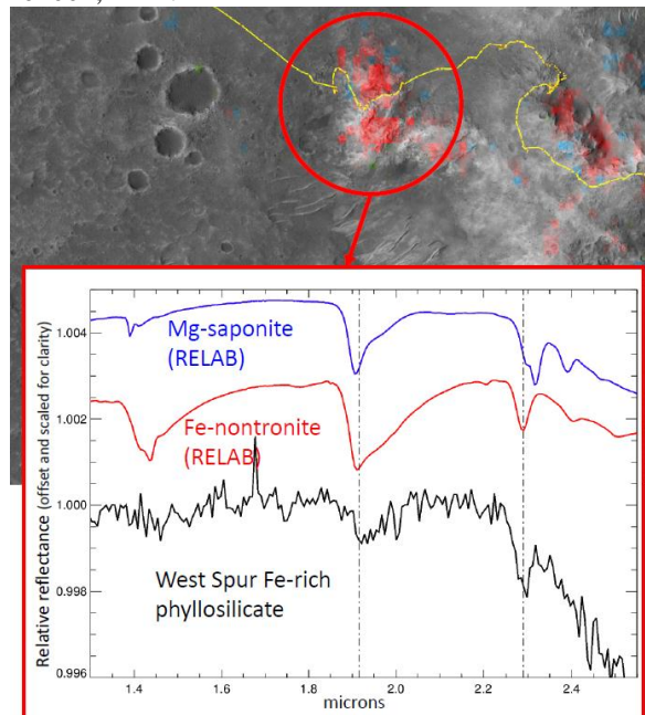
Figure 3. CRISM mineral map of the 2.30 \mu\text{m} absorption band (red) over West Spur derived from the stacking procedure. A spectrum extracted from the red area is compared to Mg-phyllsilicate (blue) and Fe-phyllsilicate. The yellow line indicates the track of Spirit.
